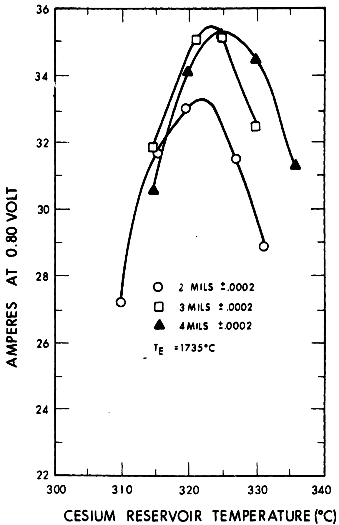
Figure 51. Converter Optimization at 0.80 Volt. Temperature of Collector 704°C to 710°C (all dc data points)
