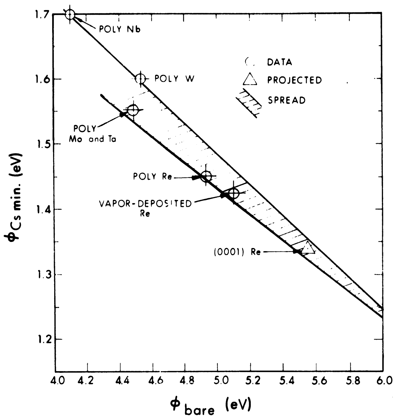
Figure 1. Empirical Relationship Between Bare Work Function and Minimum Cesium-adsorbed Work Function
