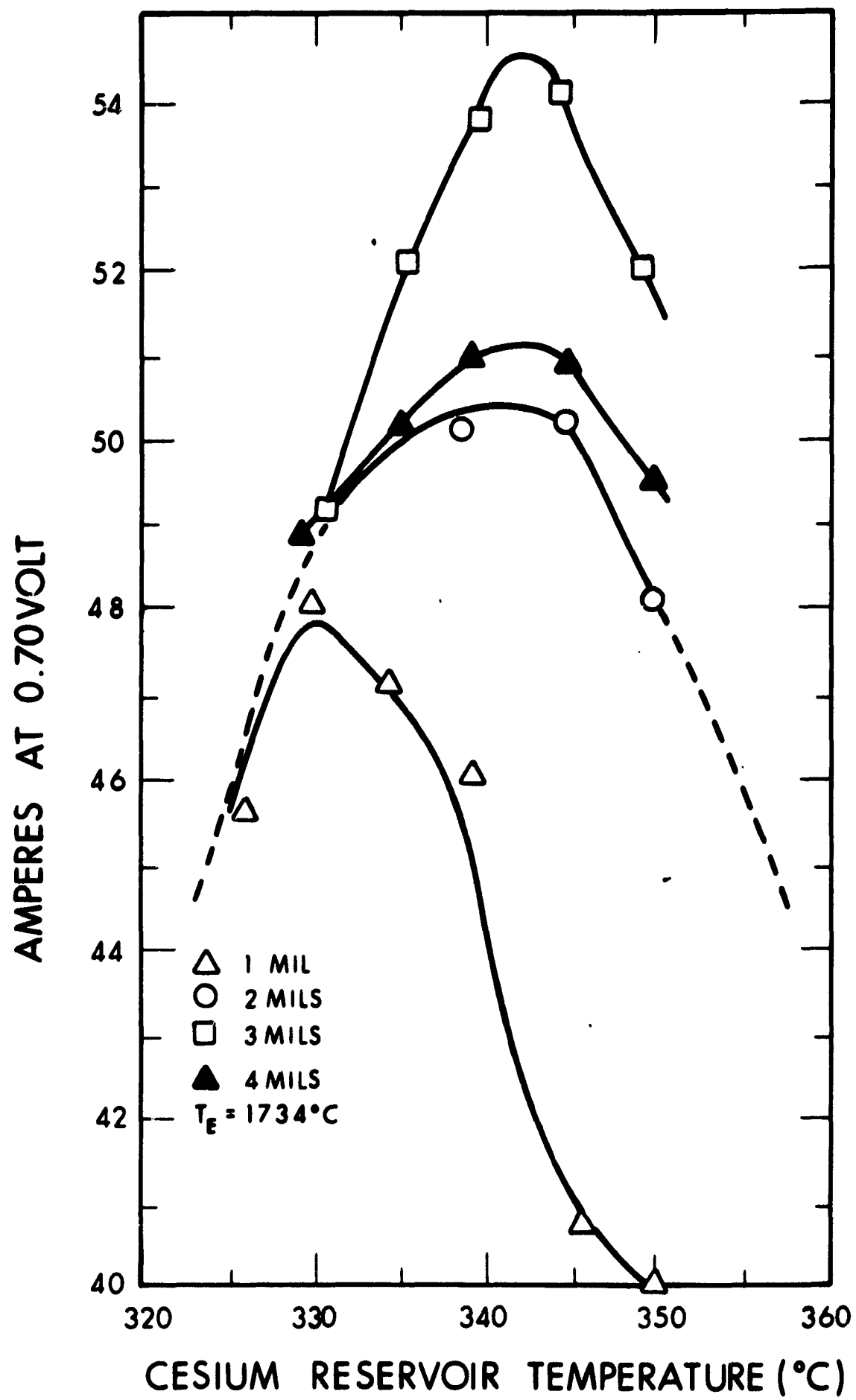
Figure 49. Converter Optimization at 0.70 Volt. Temperature of Collector 775°C (all dc data points)
