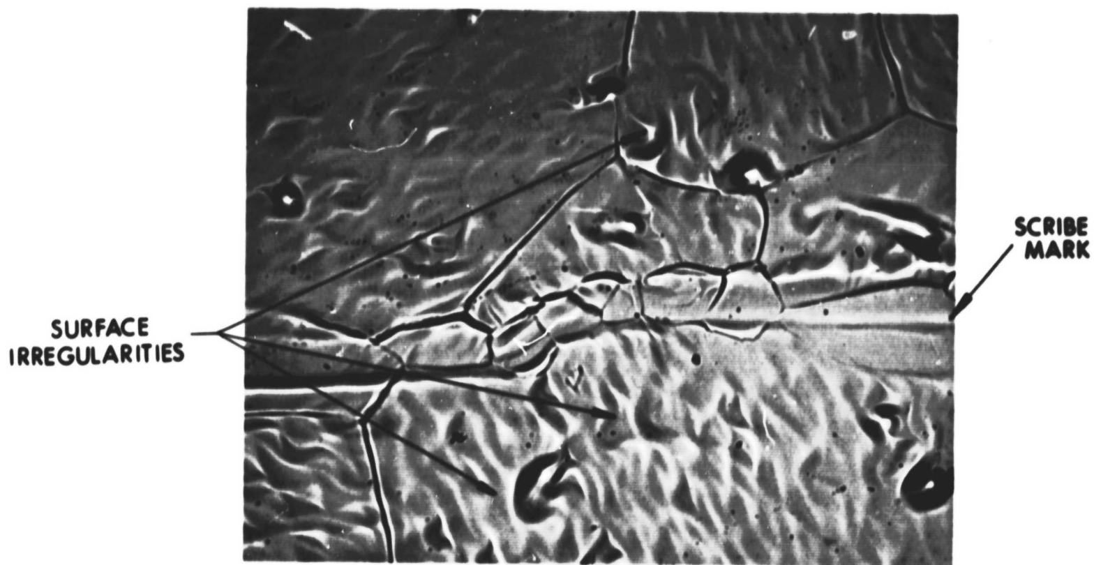
Figure 2. 500X Photomicrograph of Diamond Lapped Vapor-Deposited Rhenium, Sample II, After 2 Hours of Vacuum Outgassing at 2300°C and 60 Hours of Operation at 1900°C
