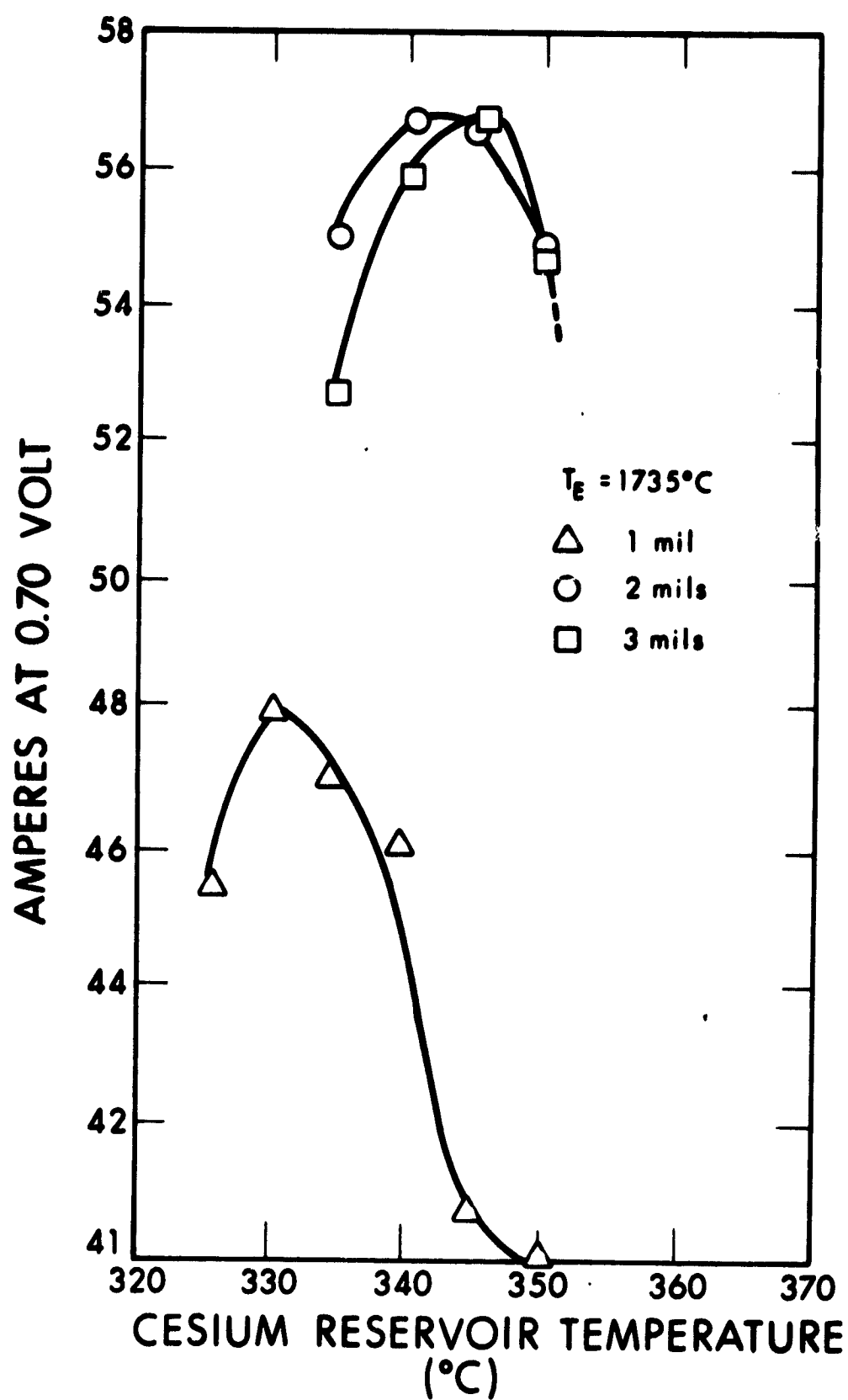
Figure 48. Converter Optimization at 0.70 Volt. Temperature of Collector 745^\circ\text{C} to 760^\circ\text{C} (all dc data points)
