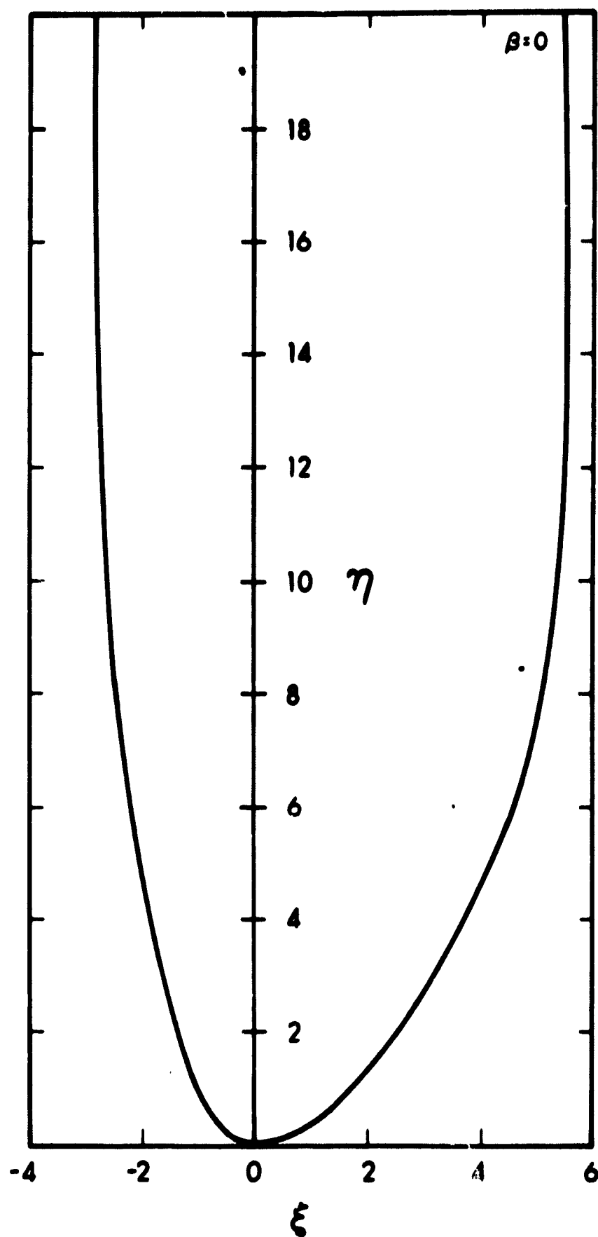
Figure 68. Normalized Potential, \eta , versus Normalized Distance, \xi , in the Interelectrode Space for \beta = 0 ( \beta is defined in the text)
