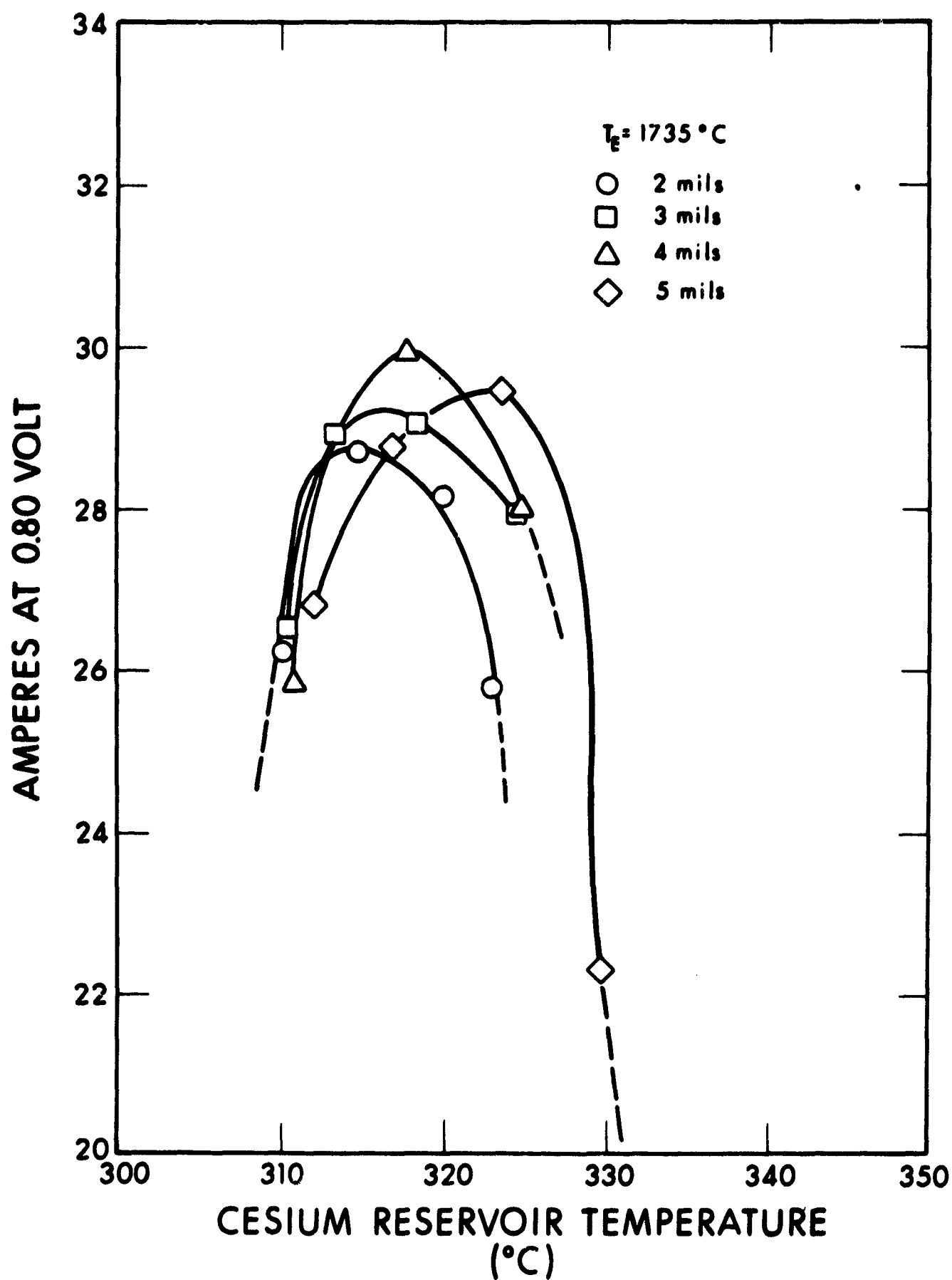
Figure 50. Converter Optimization at 0.80 Volt. Temperature of Collector 640^\circ\text{C} to 650^\circ\text{C} (all dc data points)
