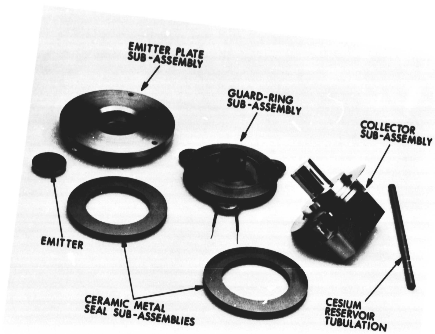
Figure 36. Variable Parameter Test Vehicle Subassemblies and Components
