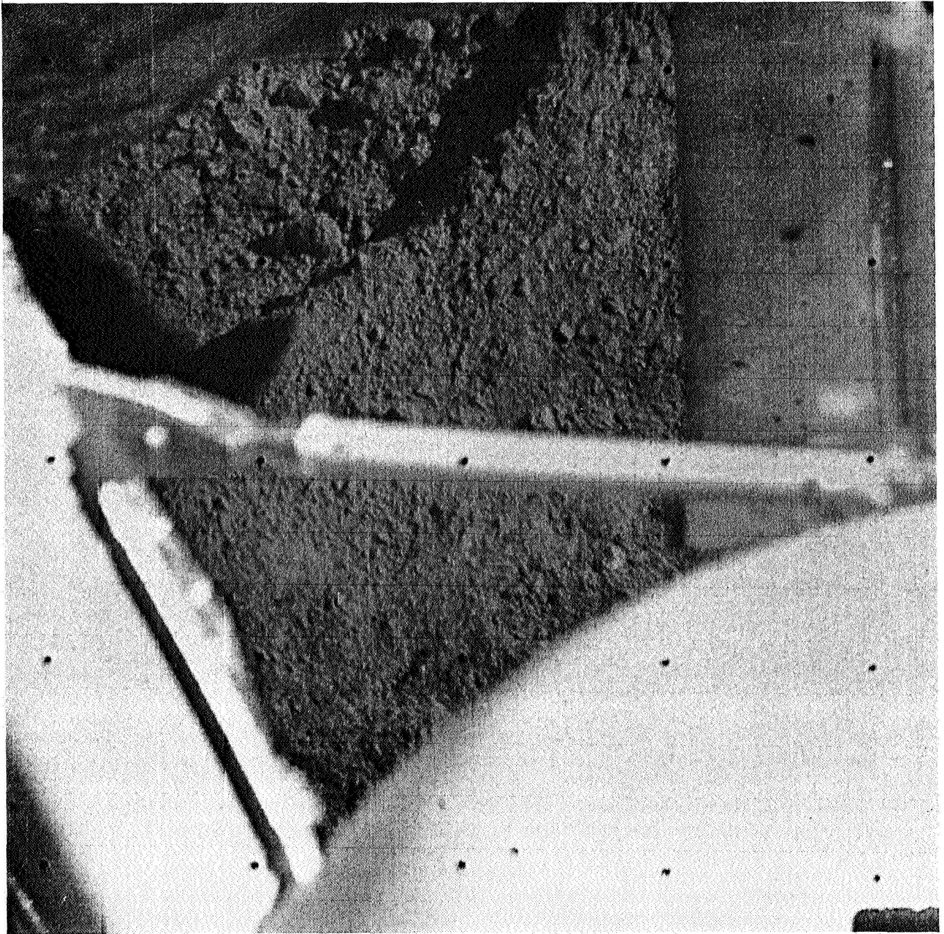
Fig. VI-12. Computer-processed picture of surface depression made by crushable block assembly 3. (Note depression made in upper left-hand corner; part of a propellant tank obscures the imprint in extreme left-hand corner. Sun angle is 41^\circ and from the right of the picture.)
