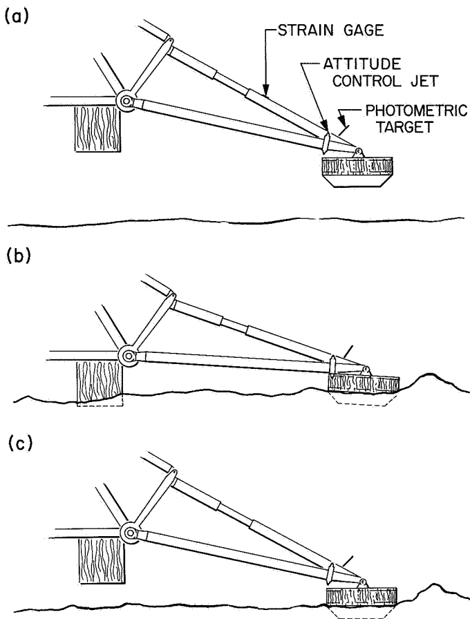
Fig. VI-3. Surveyor landing leg assembly, showing articulation in events during landing. [Assembly is shown fully extended in (a); during landing, the shock absorber compresses and the footpad moves up and away from the spaceframe, as shown in (b); assembly is shown re-extended after landing in (c).]
