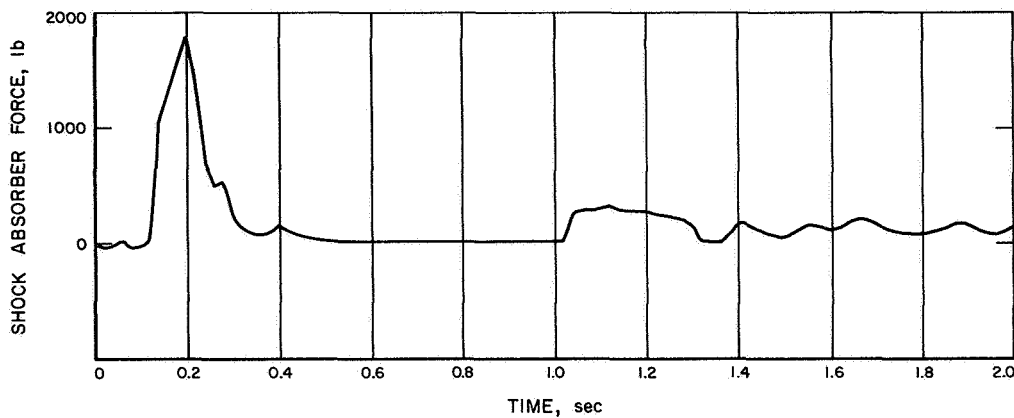
Fig. VI-5. Computer-simulated axial shock absorber strain gage data for landing on a hard surface
