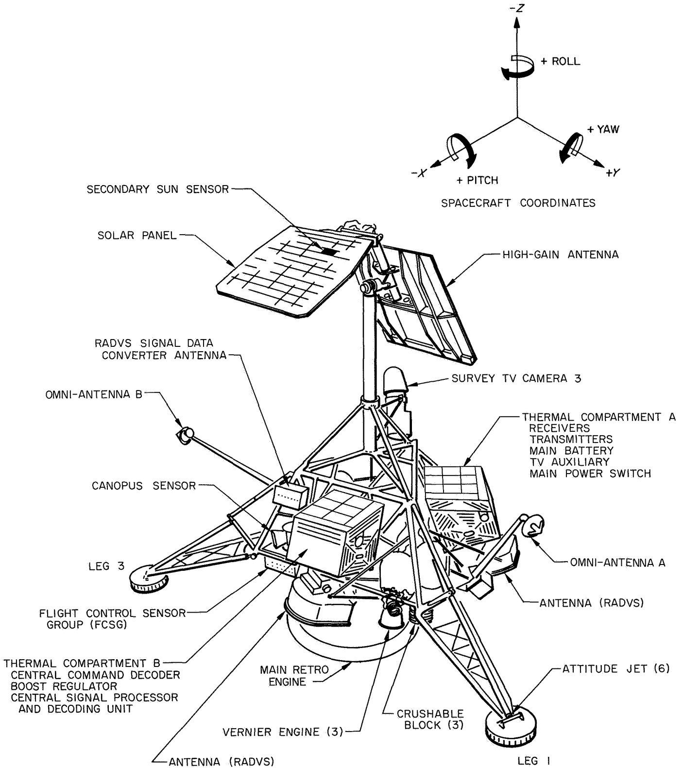
Fig. IV-3. Surveyor spacecraft configuration
