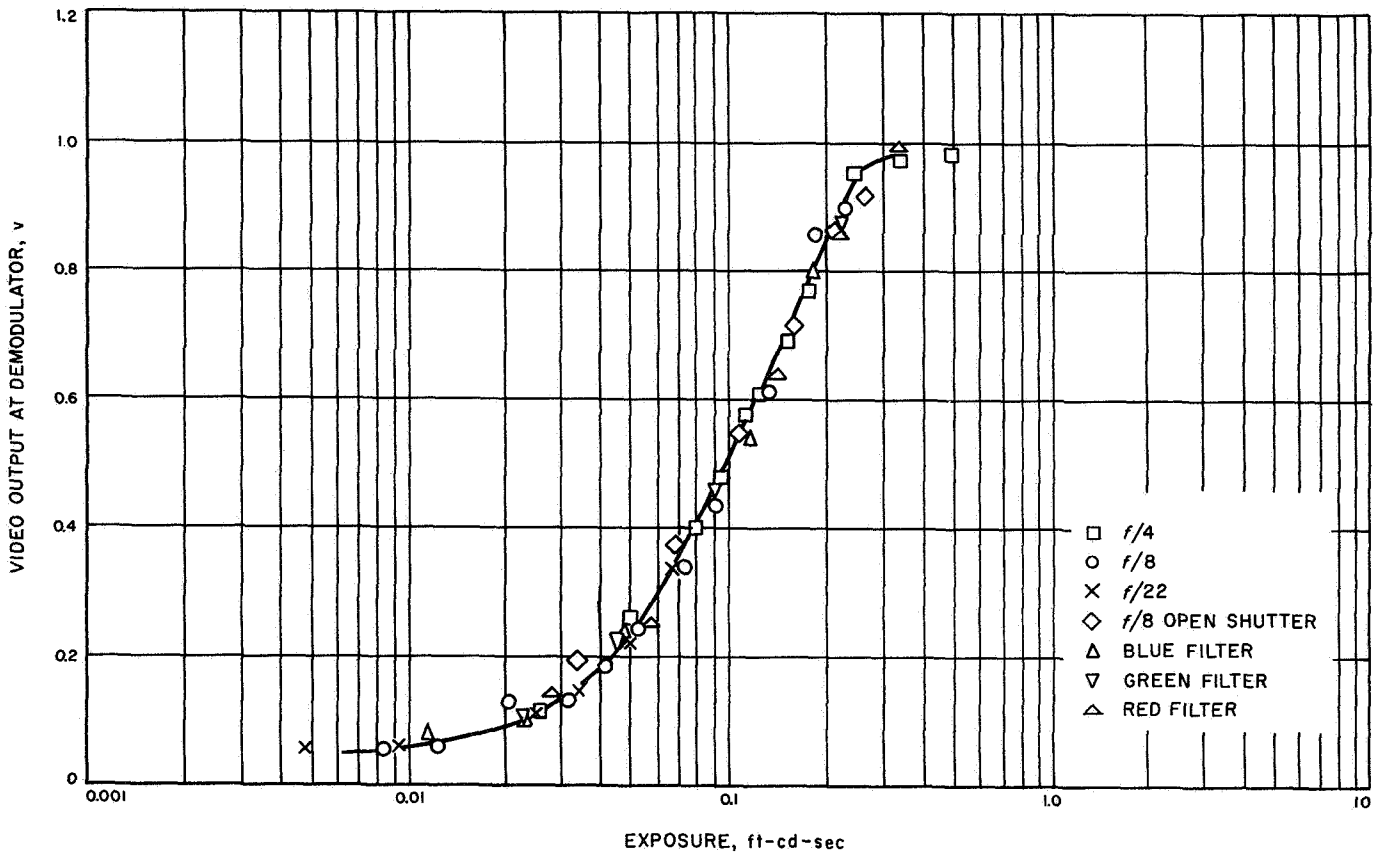
Fig. III-2. Calibration data for Surveyor I TV camera, showing dynamic range
