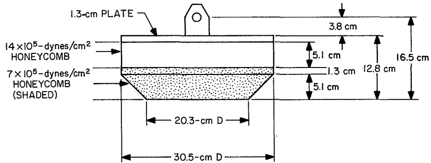
Fig. VI-2. Dimensions of landing gear assembly
