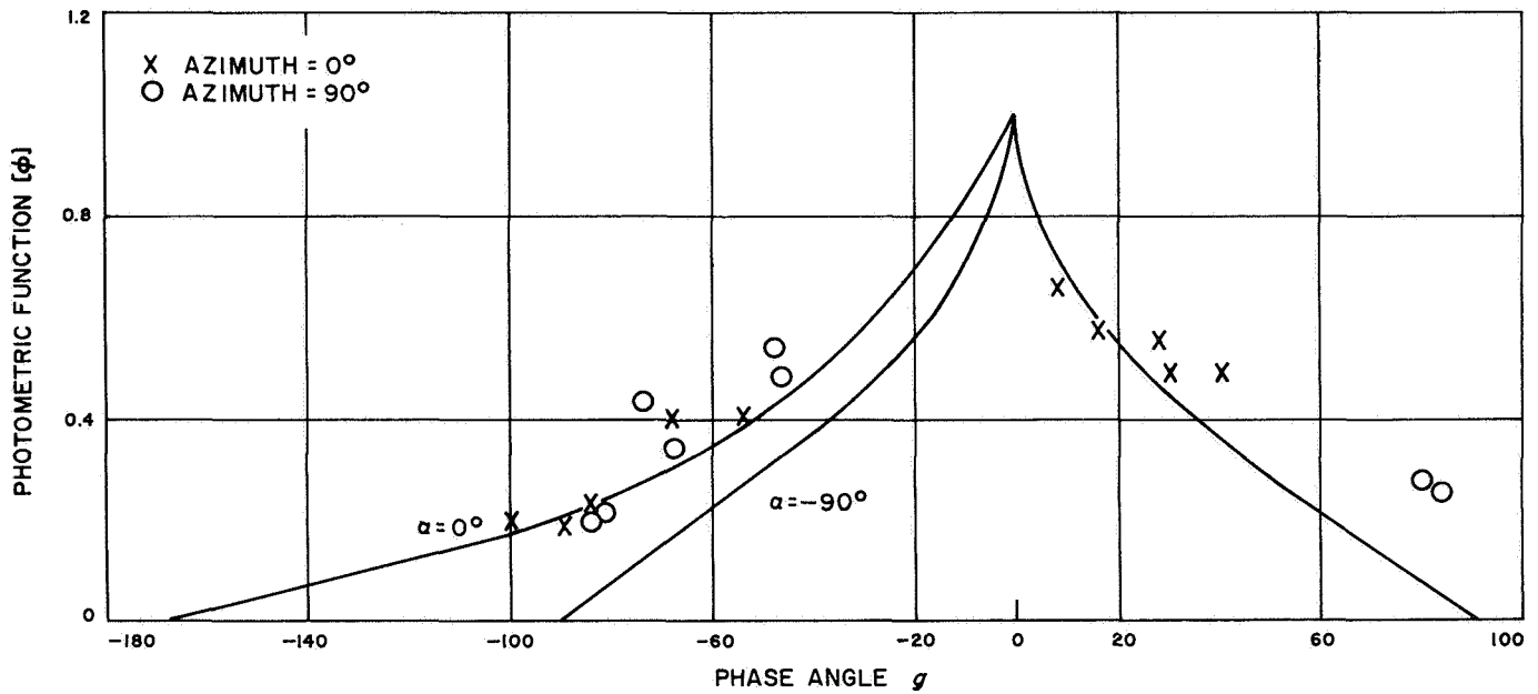
Fig. III-29. Photometric function versus phase angle. (Curves are mean values of terrestrially observed data.)
