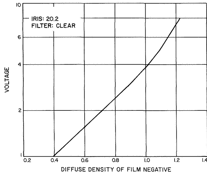
Fig. III-28. Typical plot of measured film density versus voltage from electronic grey scale
