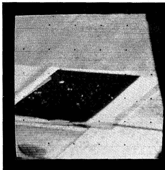
Fig. A-5. Polaroid picture of substances on radiator: largest particle 2.500 mm (0.100 in.); 100-mm focal length
