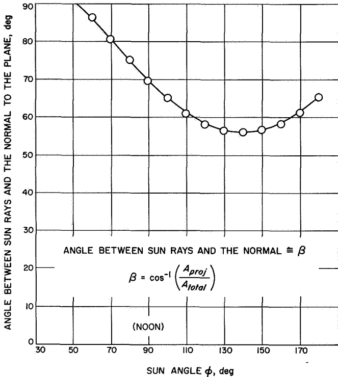
Fig. IV-9. Angle between sun rays and the normal to outboard plane of compartment A during first lunar day
