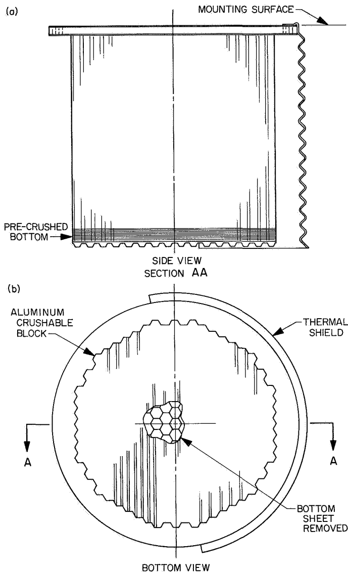
Fig. VI-14. Two views of crushable block assembly 3 including thermal shield: (a) side view and (b) bottom view
