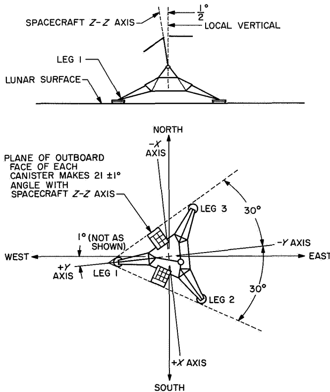
Fig. IV-6. Surveyor I spacecraft landed orientation
