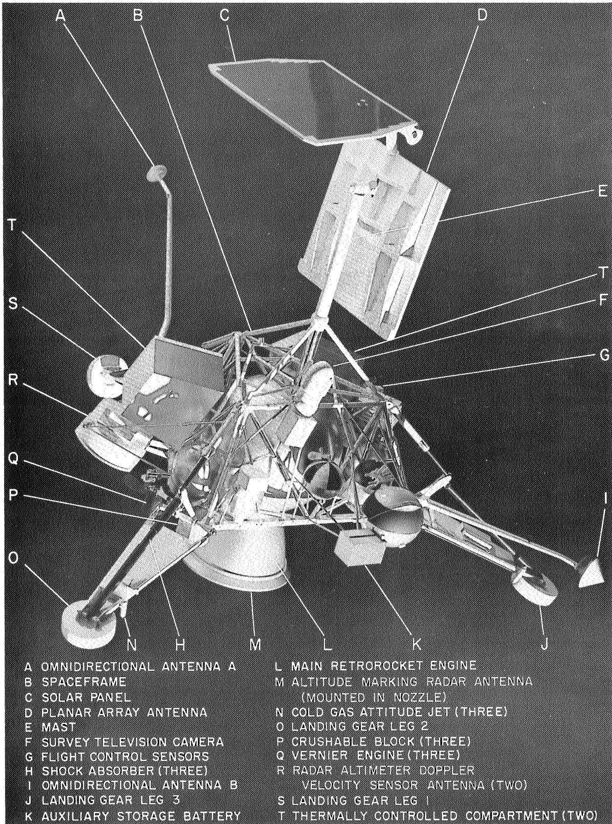
Fig. II-1. Surveyor I spacecraft configuration
