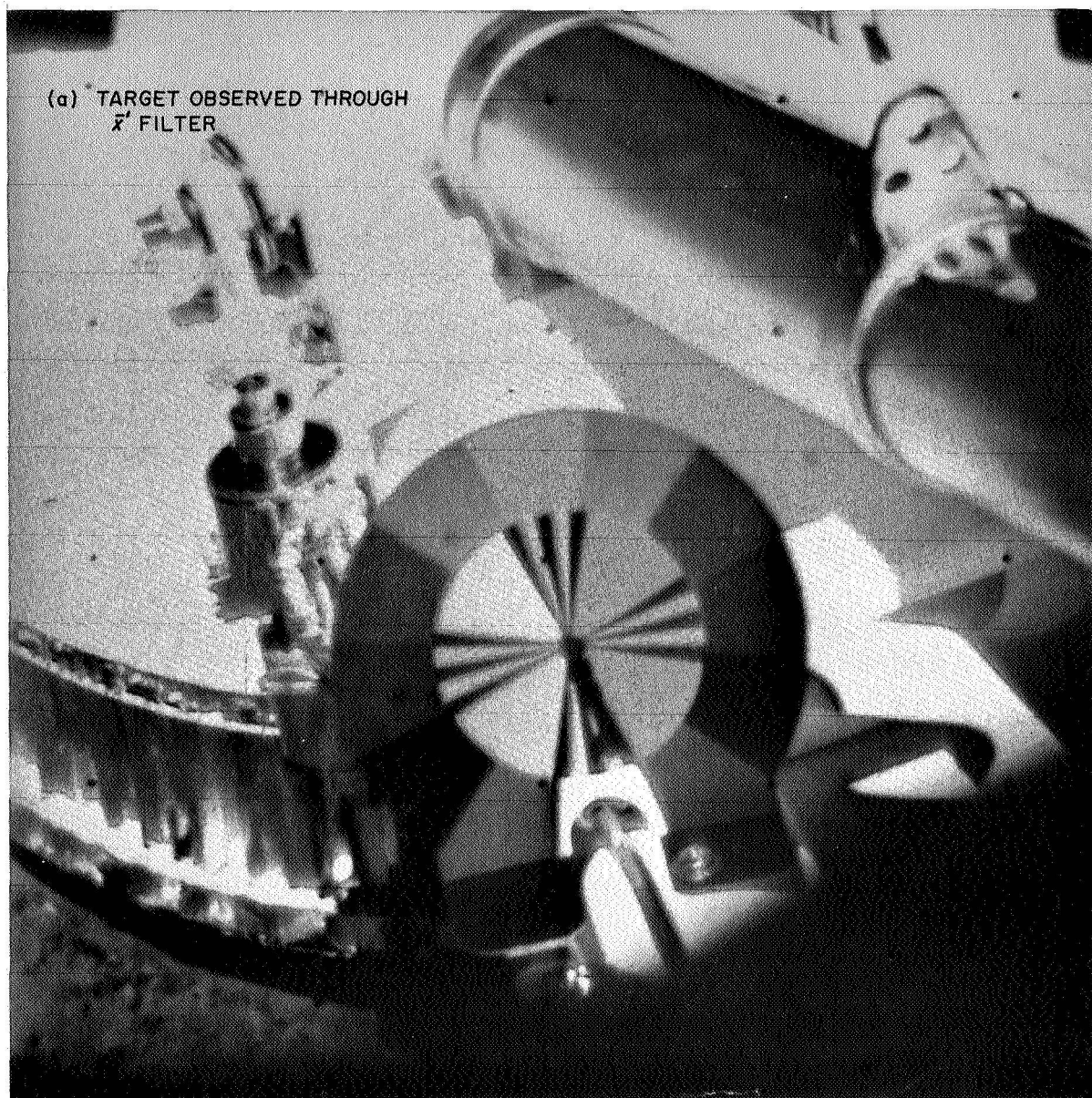
Fig. III-5. Photometric target on footpad 2
