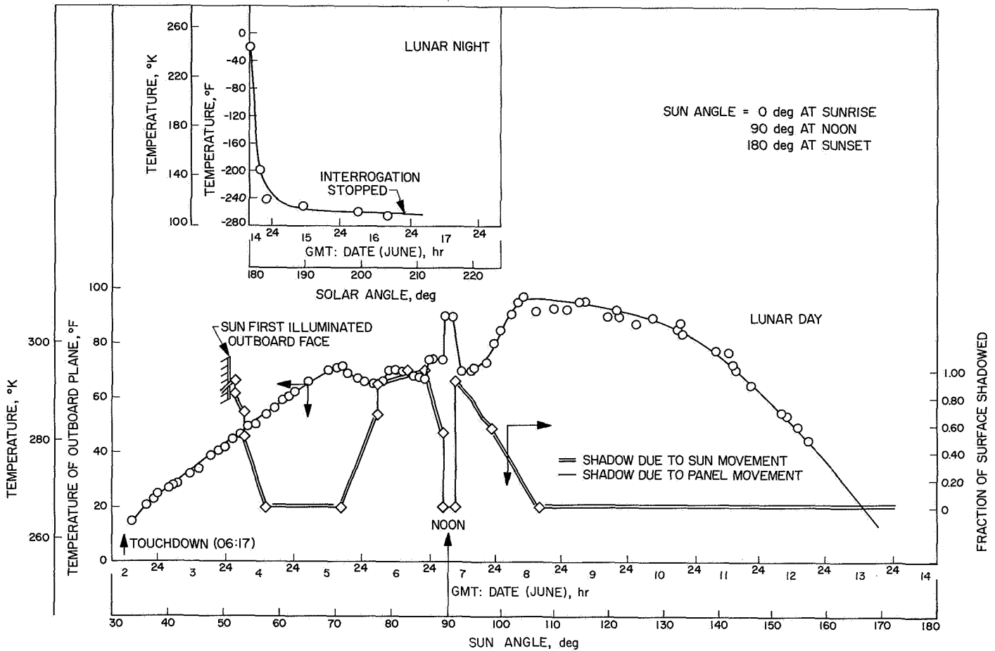
Fig. IV-7. Temperature and shadow of outboard face of compartment A during first lunar day and night
