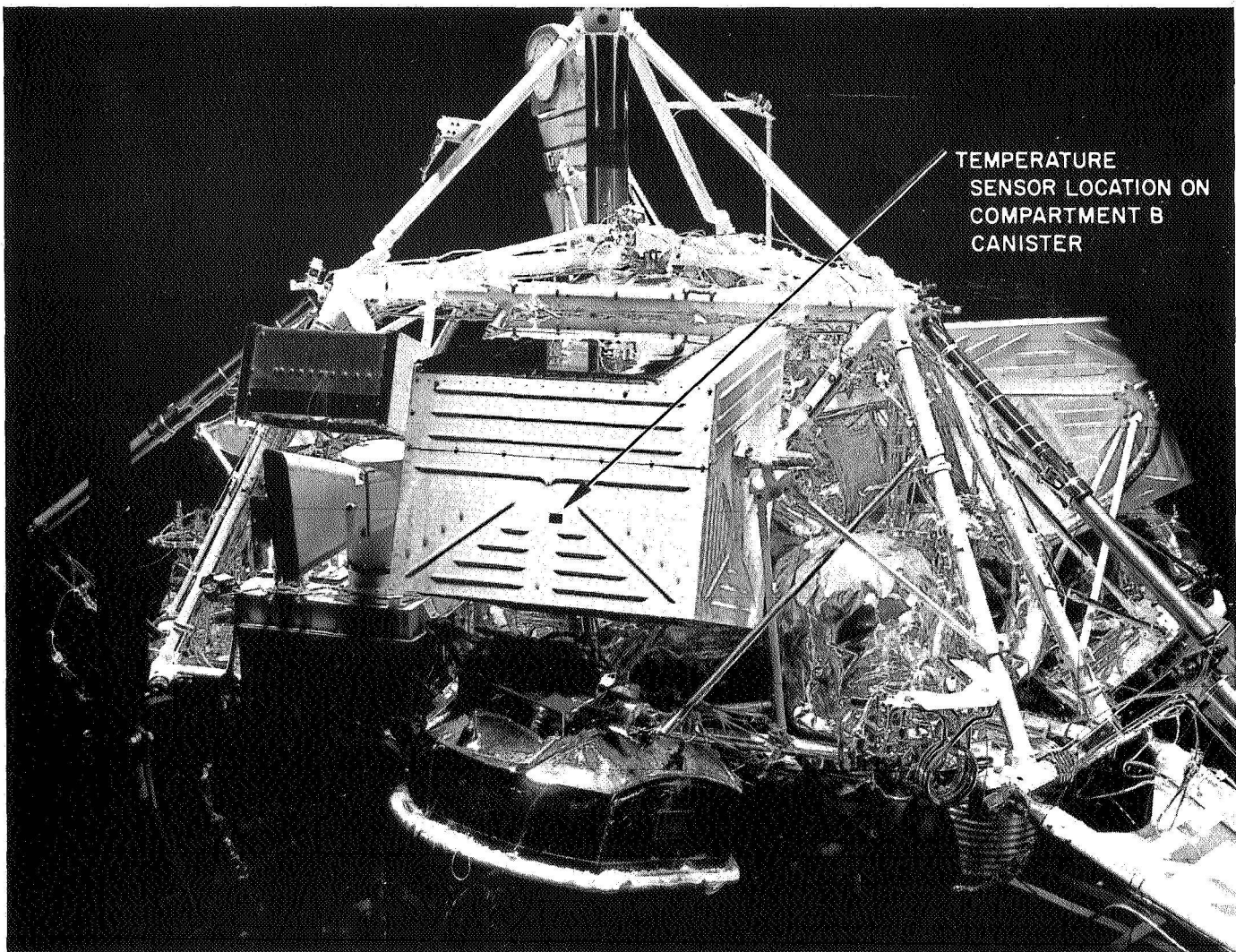
Fig. IV-5. Surveyor model showing compartment B
