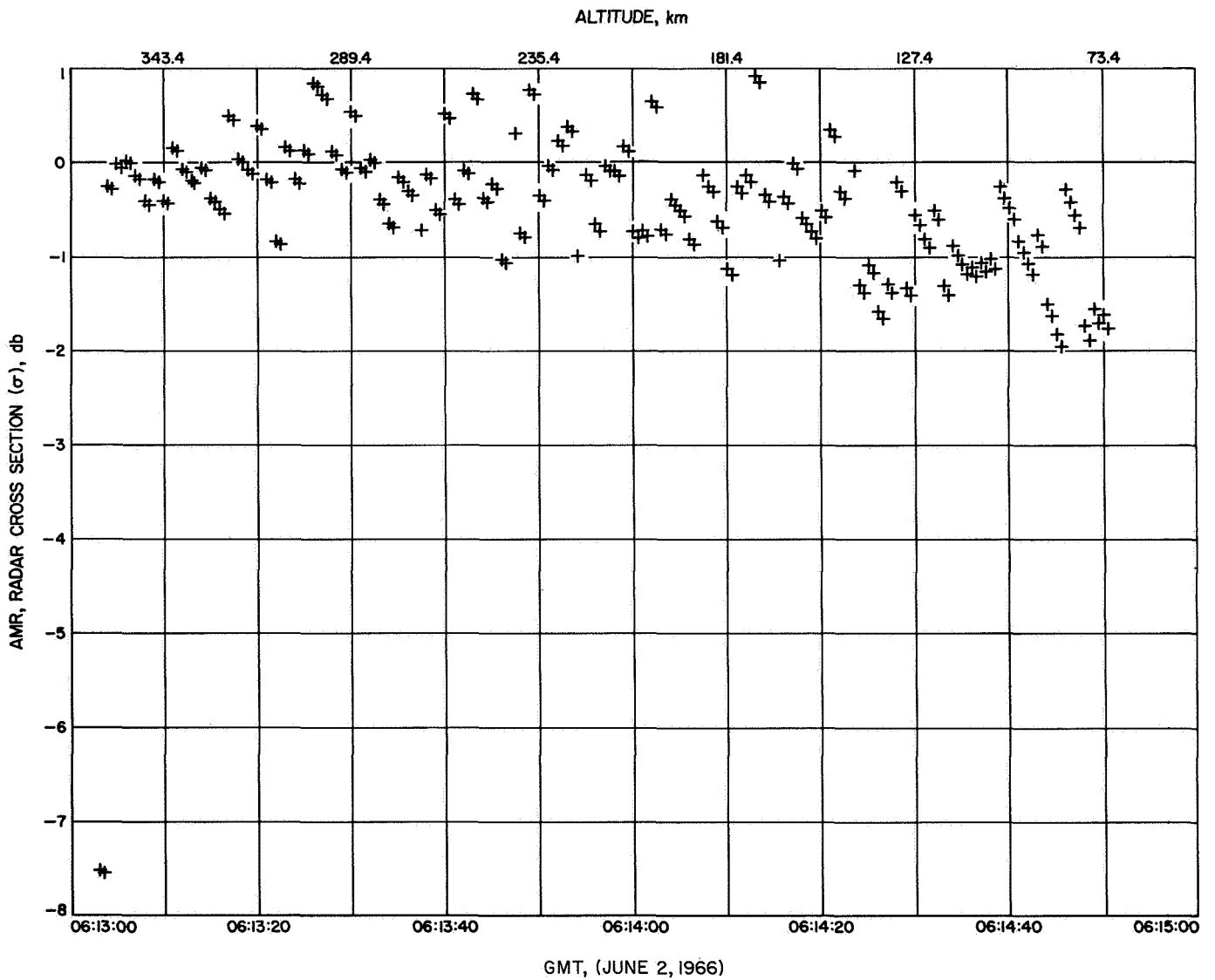
Fig. V-1. Radar cross section from AMR
