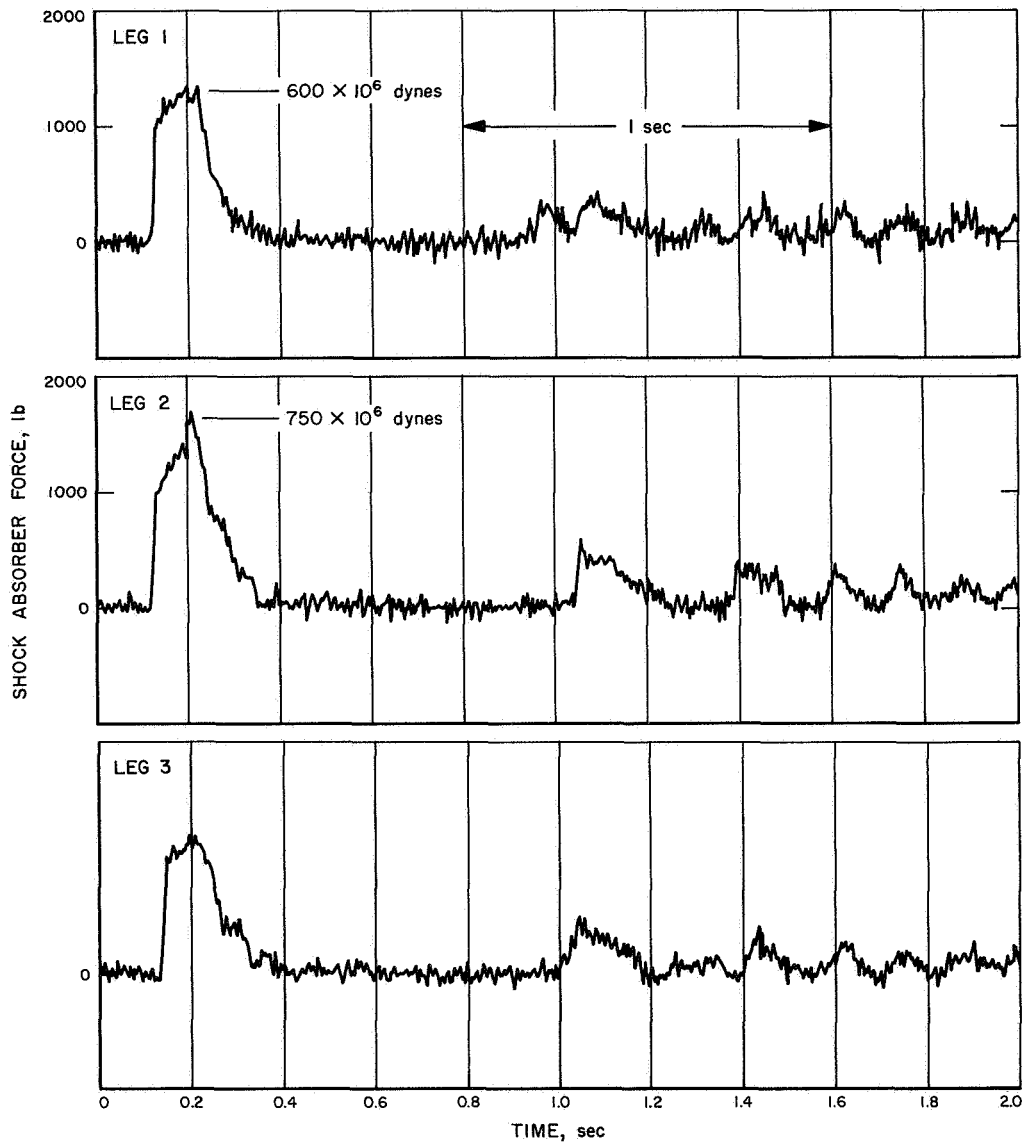
Fig. VI-4. Axial shock absorber strain gage data. (Maximum force developed by shock absorber 3 is not shown because of uncertainties in No. 3 strain gage calibration.)
