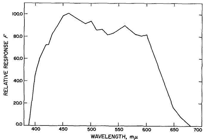
Fig. III-3. Spectral response curve of Surveyor I TV camera at clear position of filter wheel
