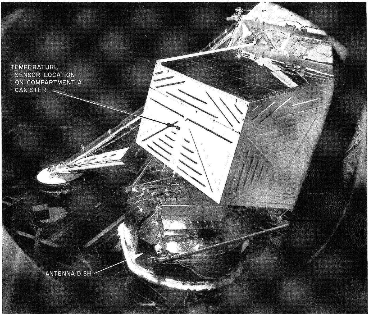
Fig. IV-4. Surveyor model showing compartment A
