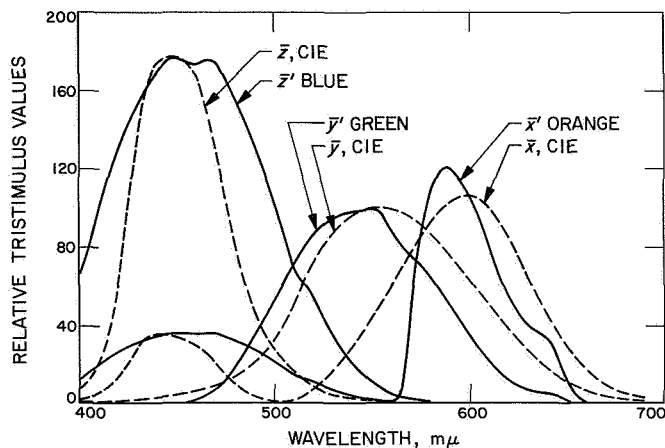
Fig. III-4. Overall camera-filter spectral response
