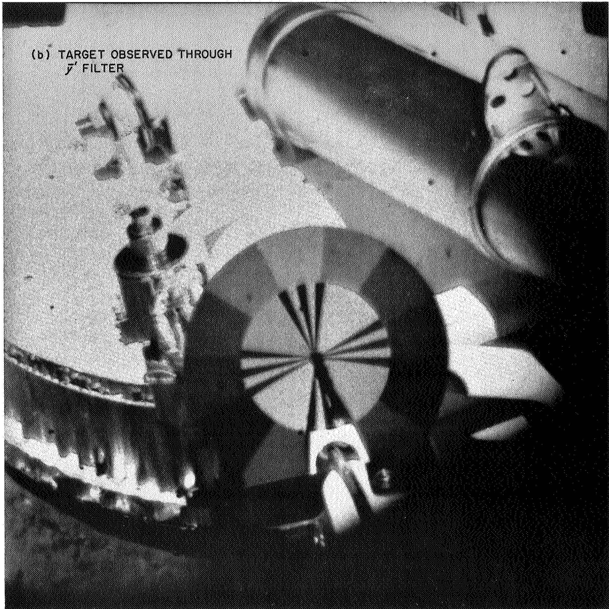
Fig. III-5. Photometric target on footpad 2 (cont'd)
