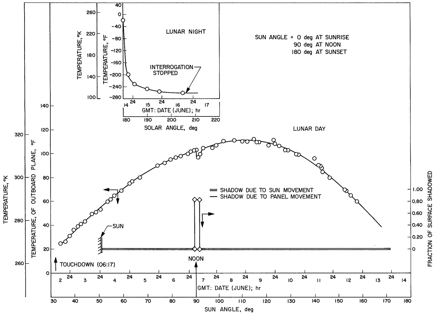
Fig. IV-8. Temperature and shadow of outboard face of compartment B during first lunar day and night
