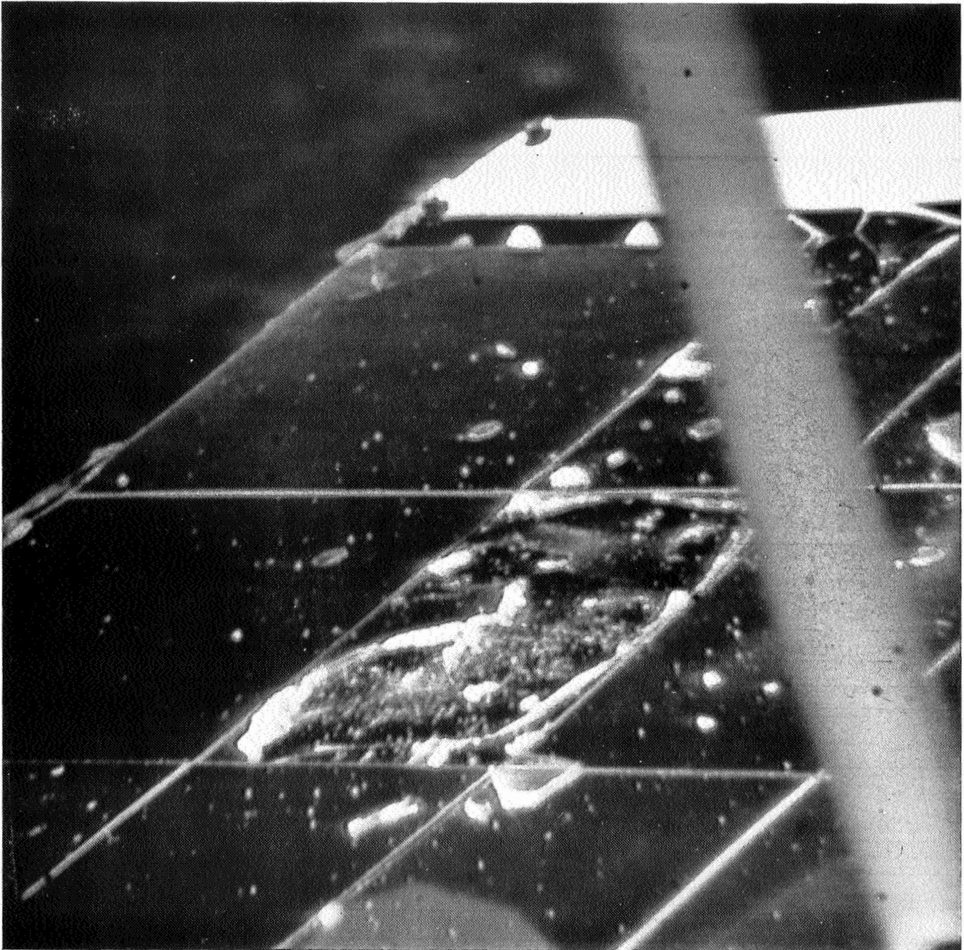
Fig. A-2. Compartment A on July 12, showing one segment of Vycor glass presumably shattered during lunar night
