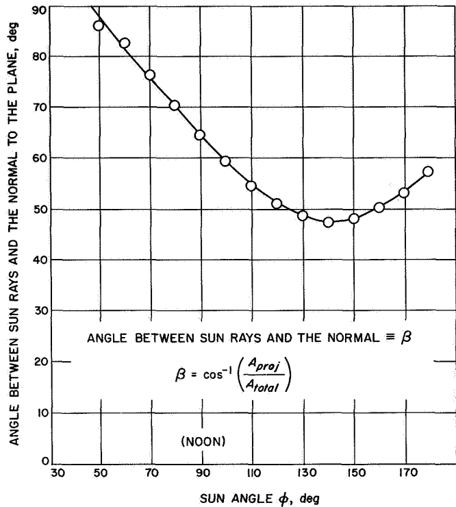
Fig. IV-10. Angle between sun rays and the normal to outboard plane of compartment B during first lunar day
