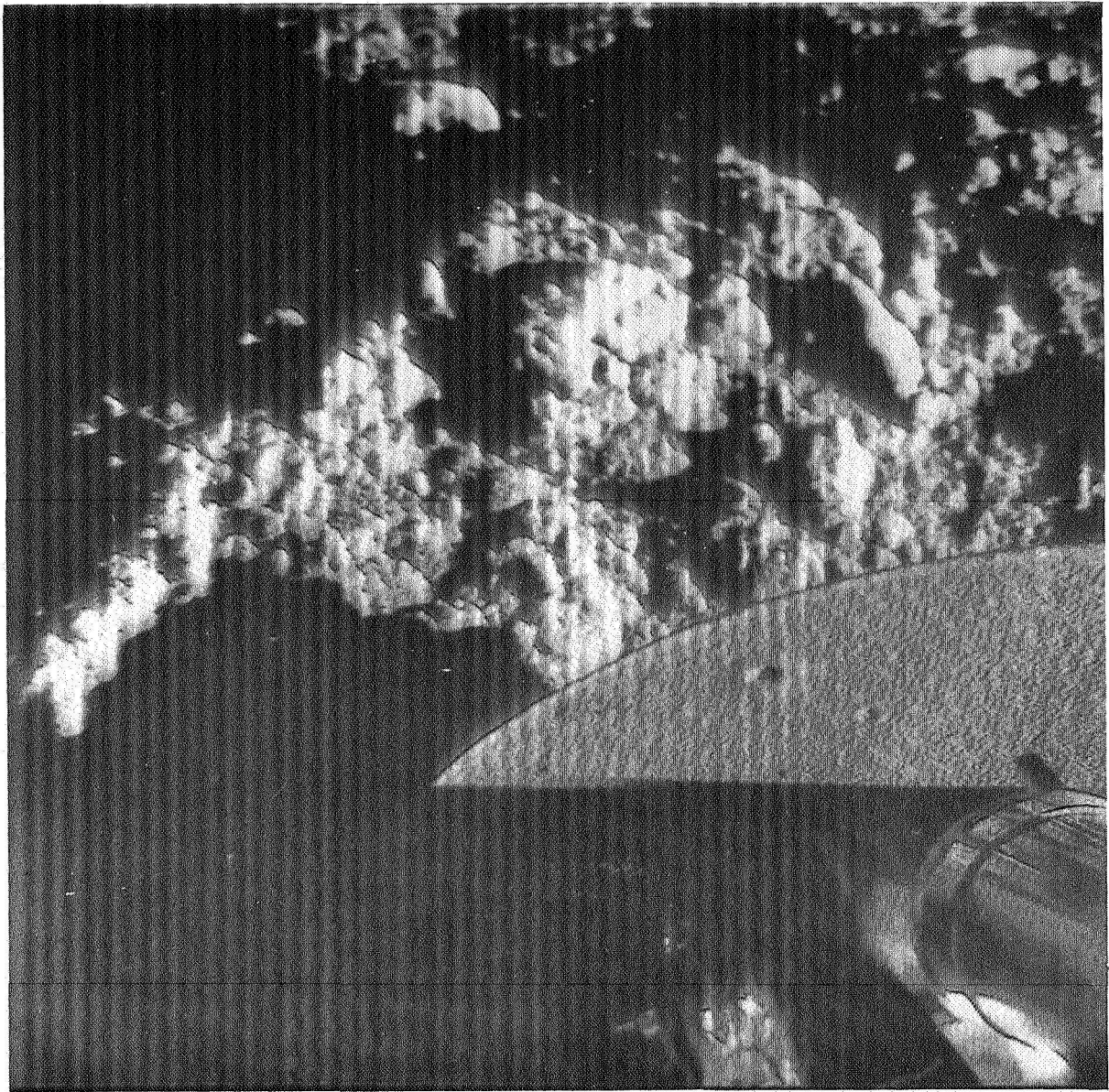
Fig. VI-10. Narrow-angle picture of footpad 2. (Sun angle is 6^\circ above horizon; texture on pad top is unexplained.)
