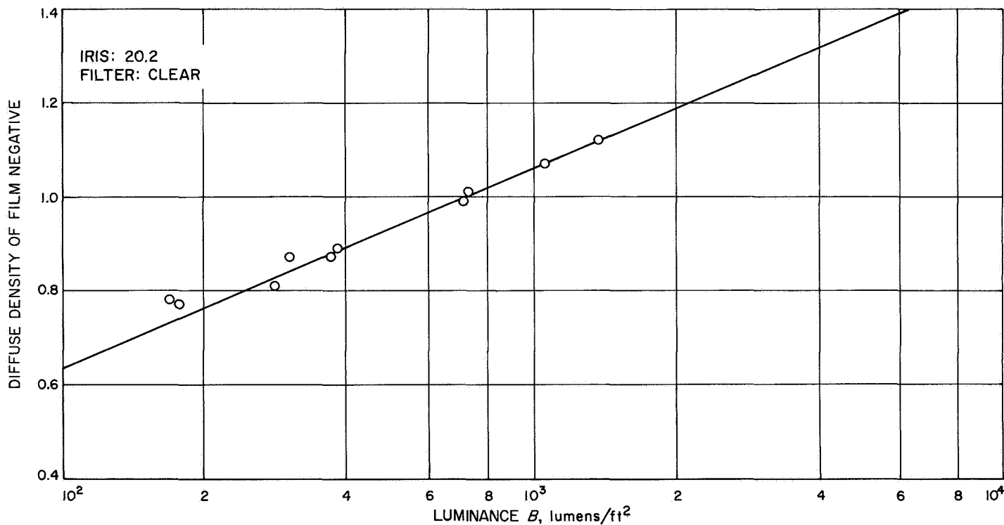
Fig. III-26. Total TV system transfer characteristic function
