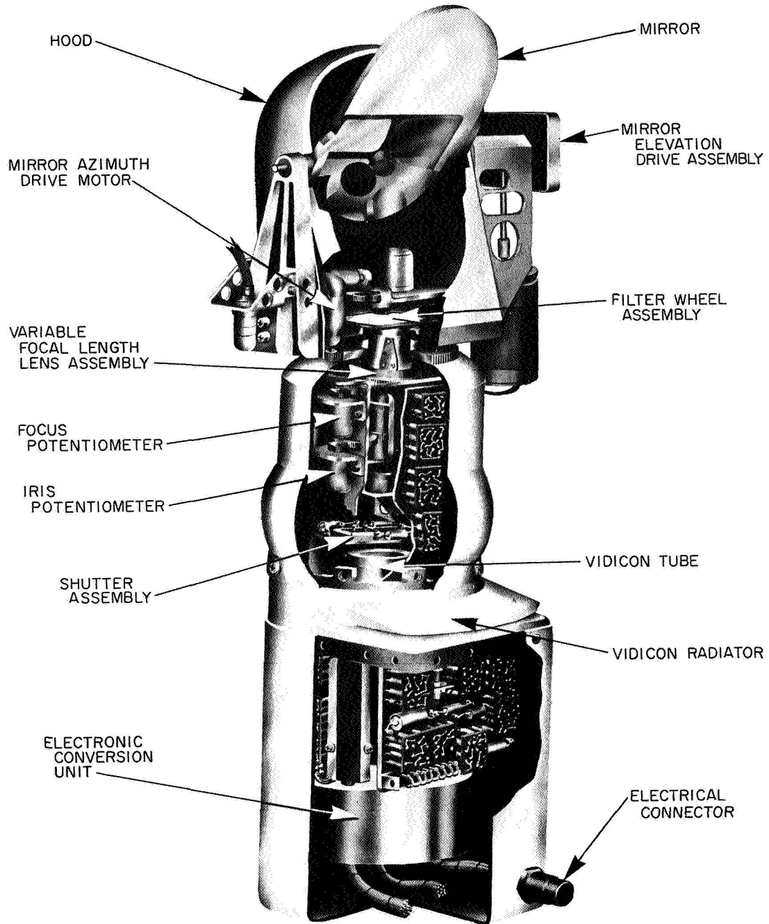
Fig. II-2. Surveyor TV camera
