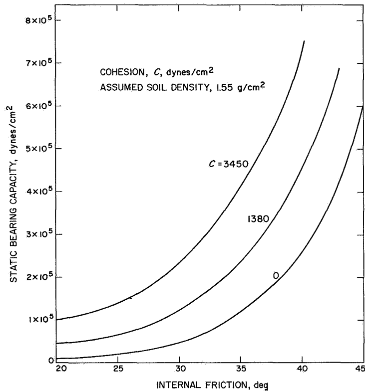
Fig. VI-15. Possible static bearing capacity of a 30.5-cm-diameter footing on moon
