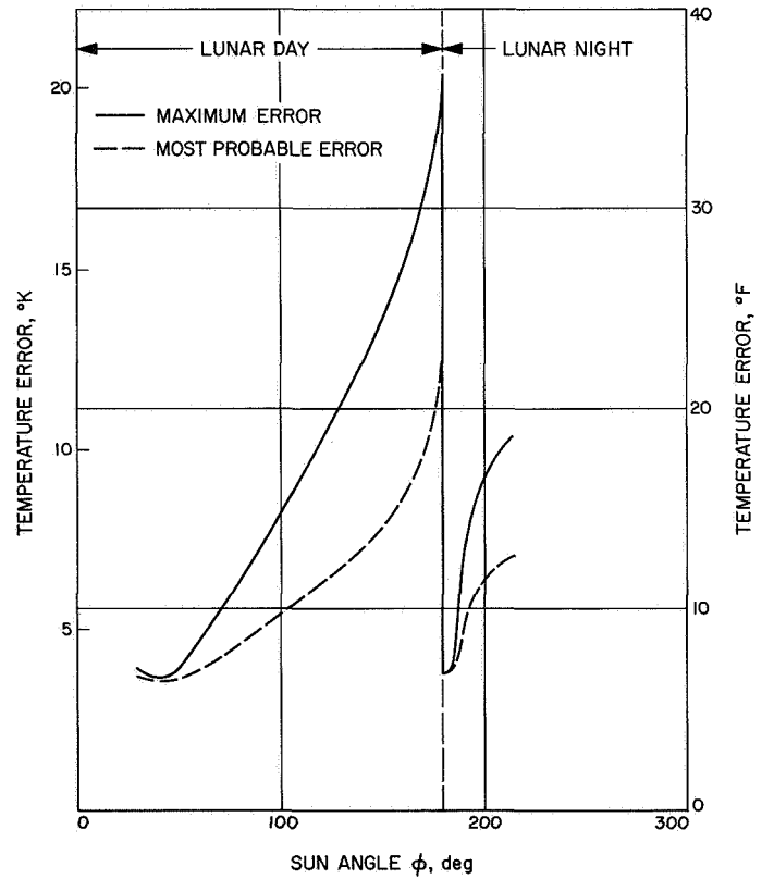
Fig. IV-13. Errors in lunar surface brightness temperature determination based on compartment B data
