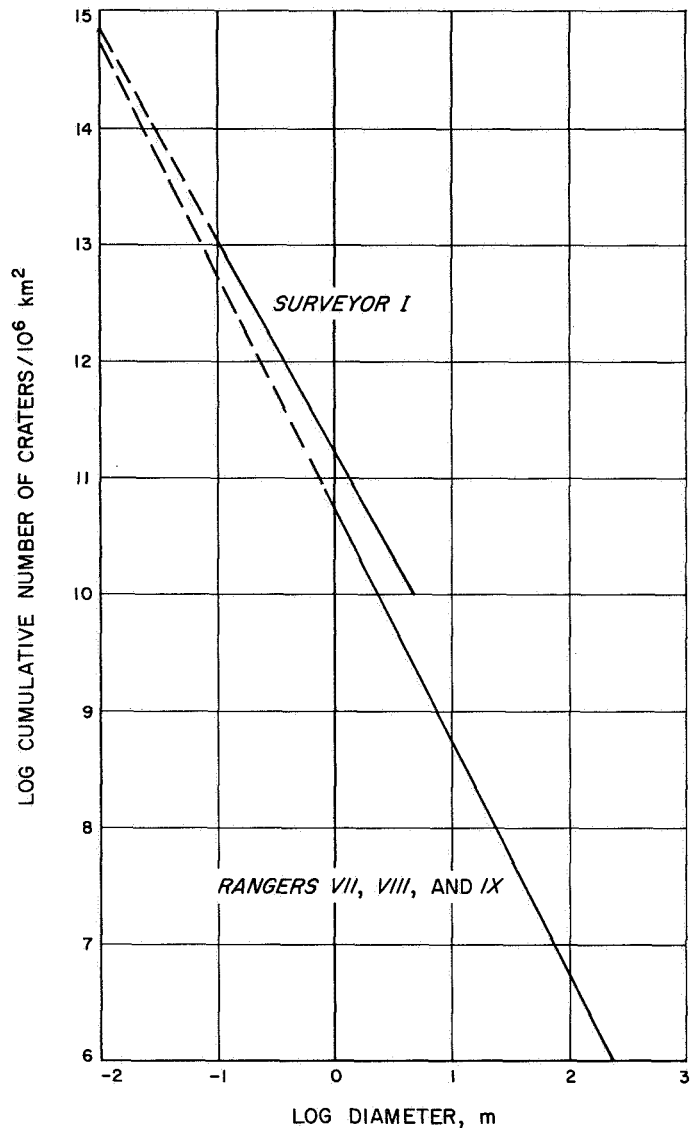
Fig. III-19. Cumulative size-frequency distribution of craters on lunar surface determined from Surveyor I pictures and from Ranger VII-IX pictures
