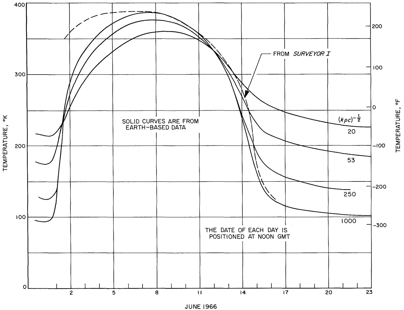
Fig. IV-2. Lunar surface brightness temperature at Surveyor I site
