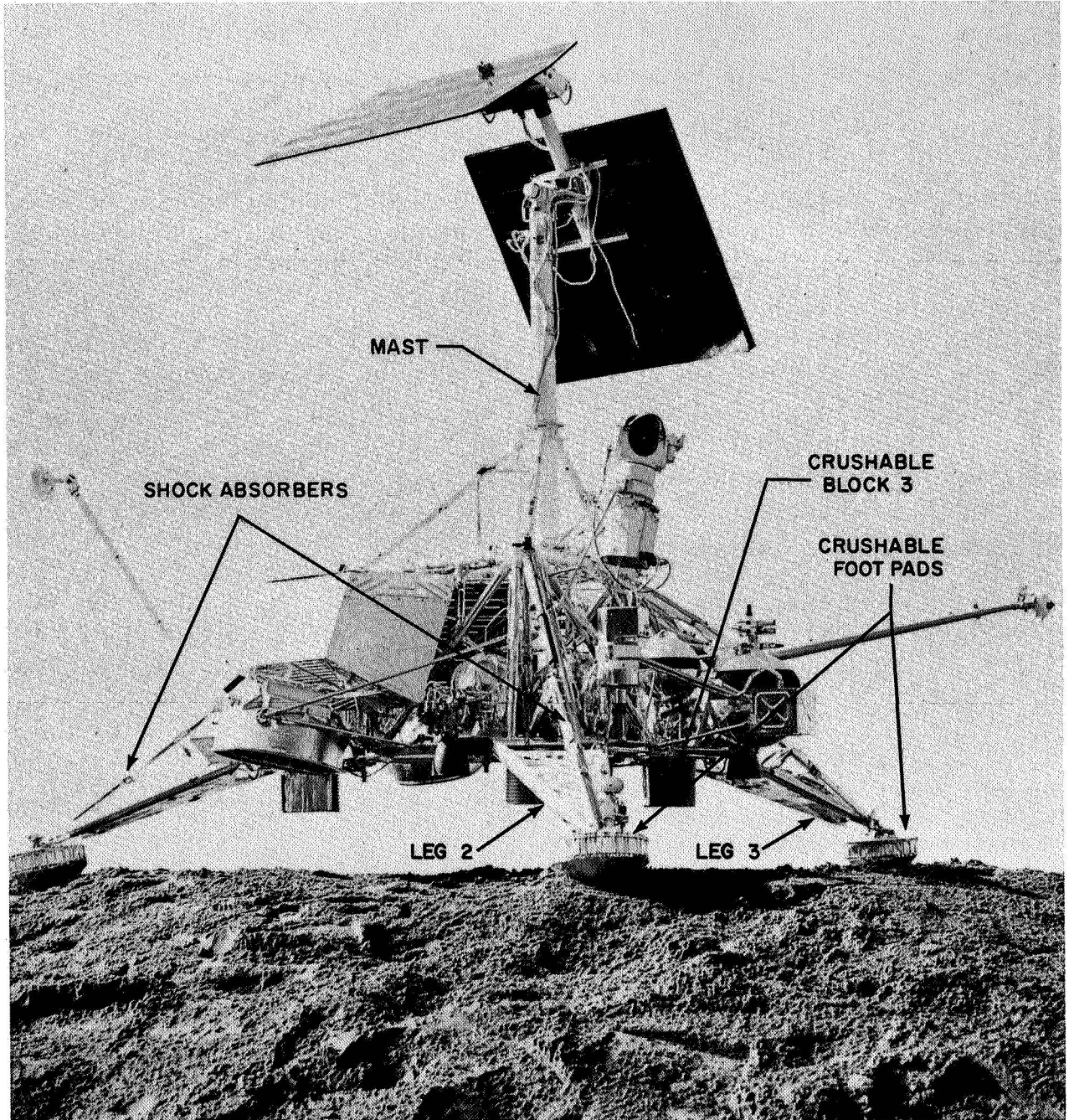
Fig. VI-1. Surveyor spacecraft
