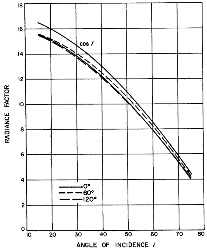
Fig. III-27. Photometric chart calibration
