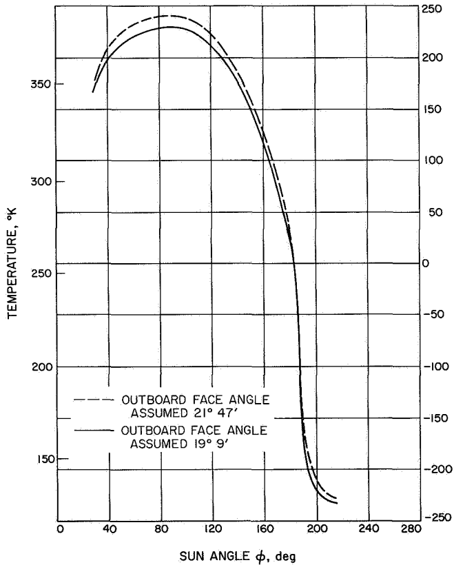
Fig. IV-12. Lunar surface brightness temperature derived from measurements of compartment B sensor
