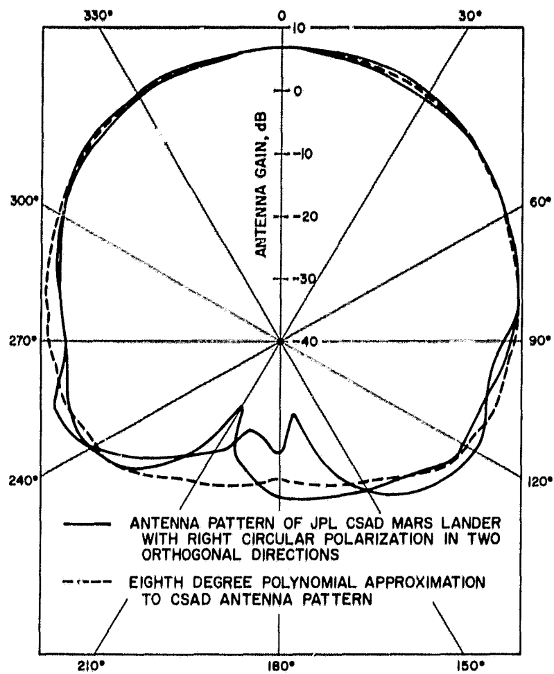
Fig. B-2. Antenna gain characteristics
