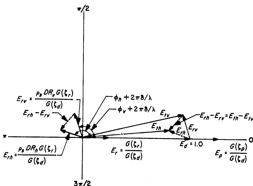
Fig. 3. CSAD lander radio electric field vector phase diagram
