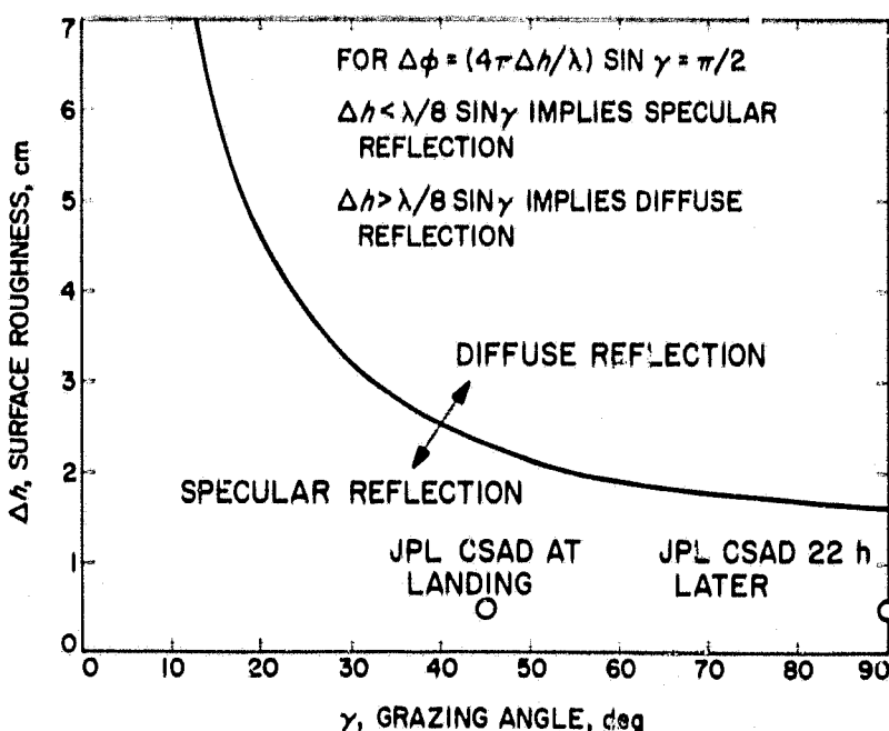
Fig. A-1. Rayleigh criterion for specular reflection at S-band (13 cm)
