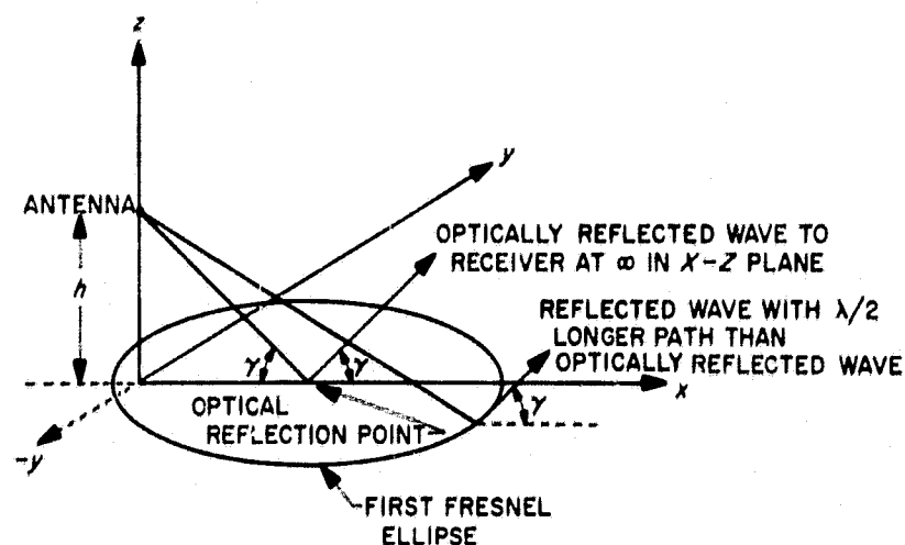
Fig. A-2. Fresnel zone calculation geometry
