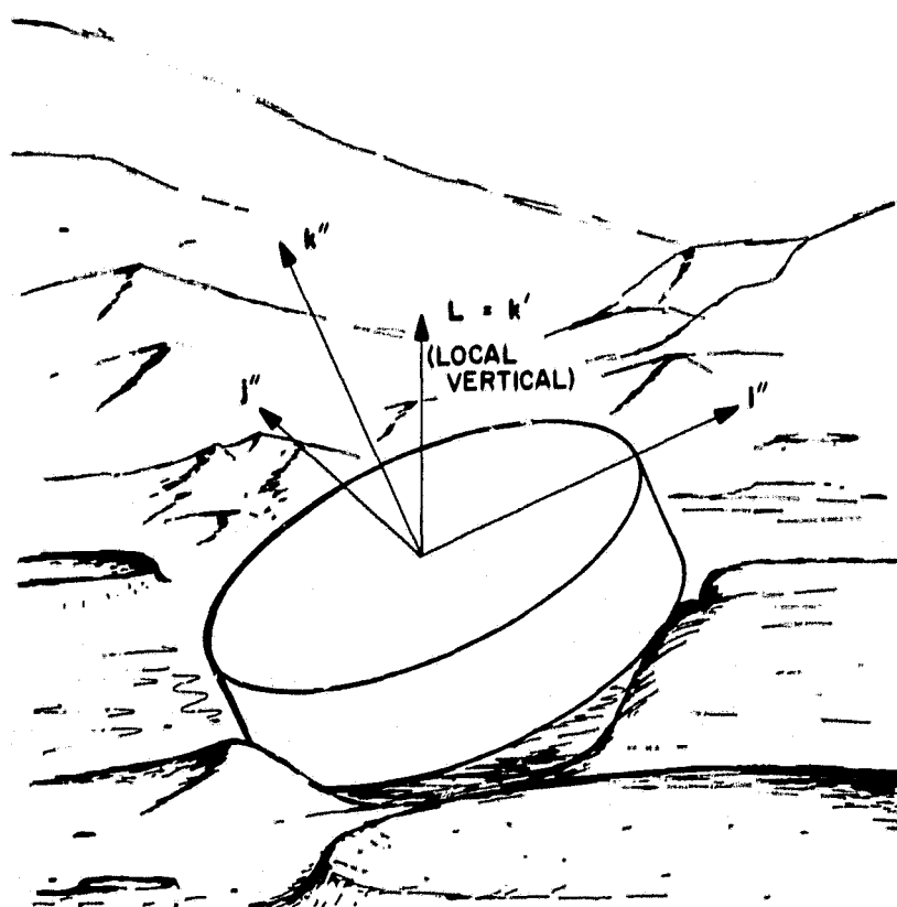
Fig. 6. Lander-centered coordinate system
