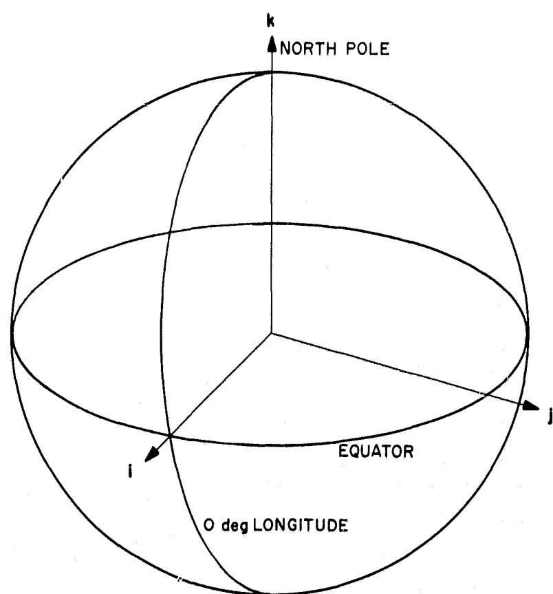
Fig. 4. Mars-centered coordinate system
