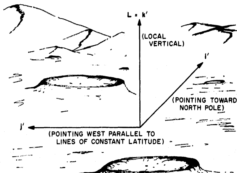
Fig. 5. Landing-site-centered coordinate system
