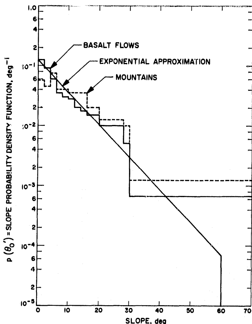
Fig. B-1. Probability density functions of Martian slopes
