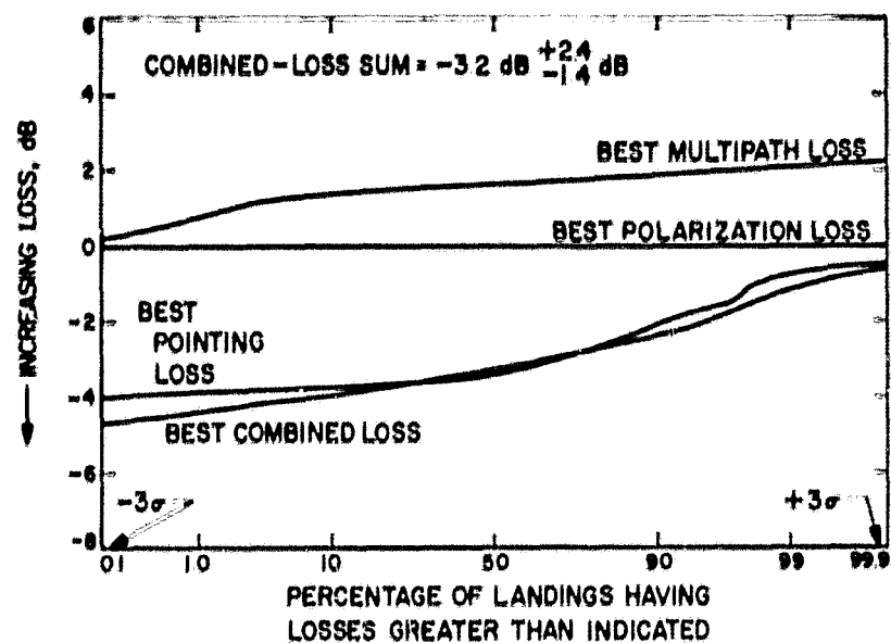
Fig. 8. Pointing, multipath, polarization, and combined loss distributions for circular polarization 21.3 h after landing
