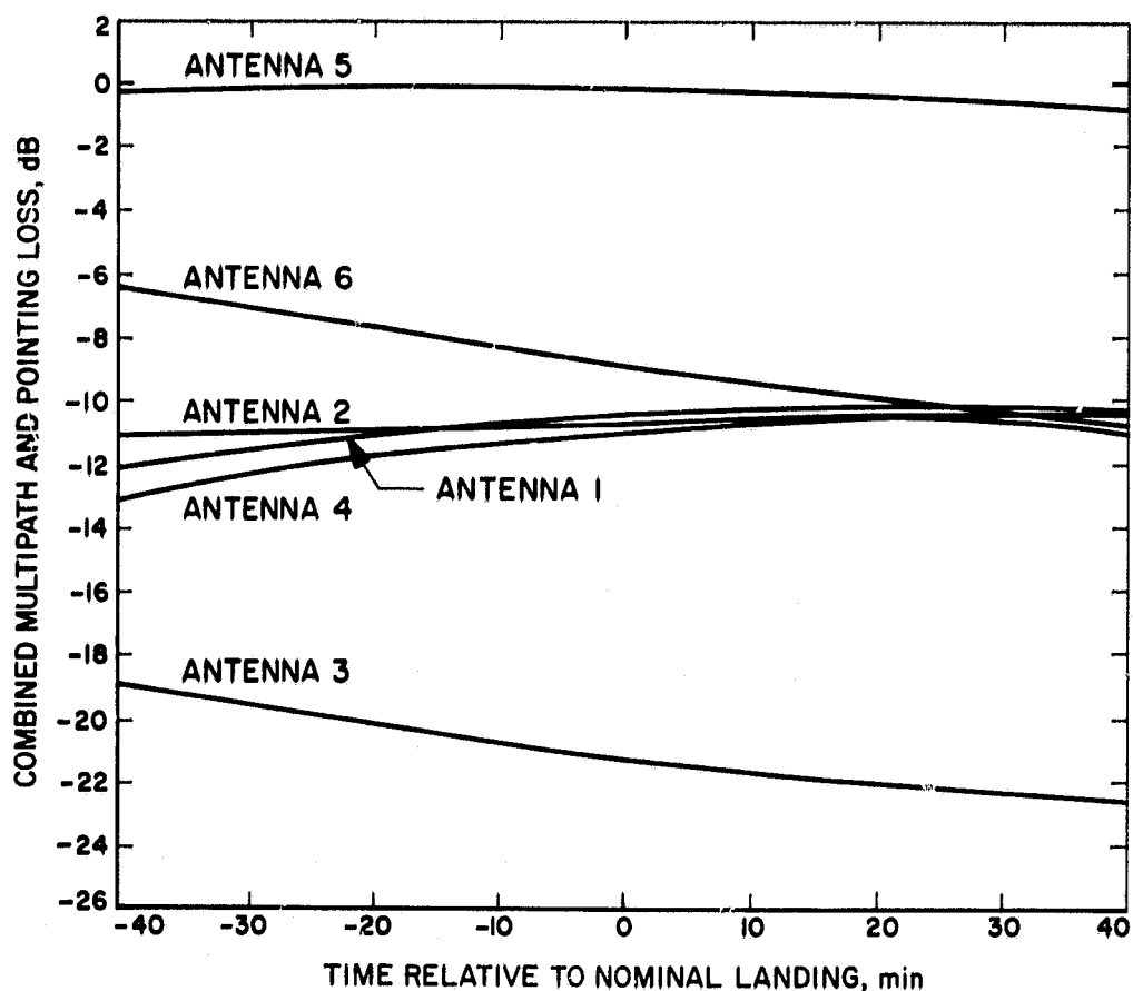
Fig. C-1. Multipath and pointing losses vs planet rotation
