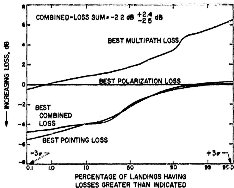
Fig. 7. Pointing, multipath, polarization, and combined loss distributions for circular polarization at landing
