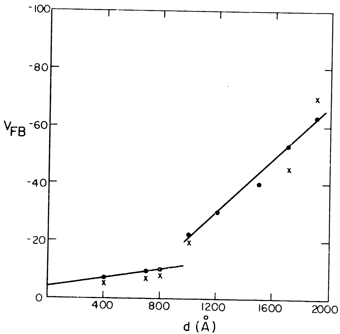
FIG. 34 V_{FB} vs thickness for step-etched sample.
