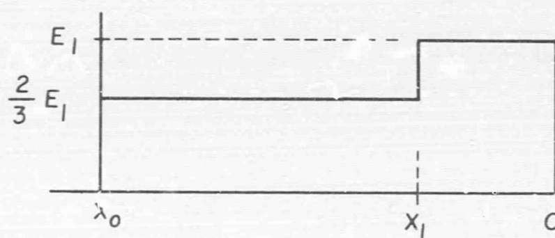
FIG. 26 Initial field distribution in memory capacitor.
