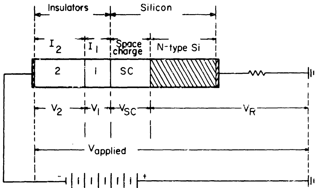
FIG. A-1 Potential drops across RC_{MI_2I_1S} circuit.
