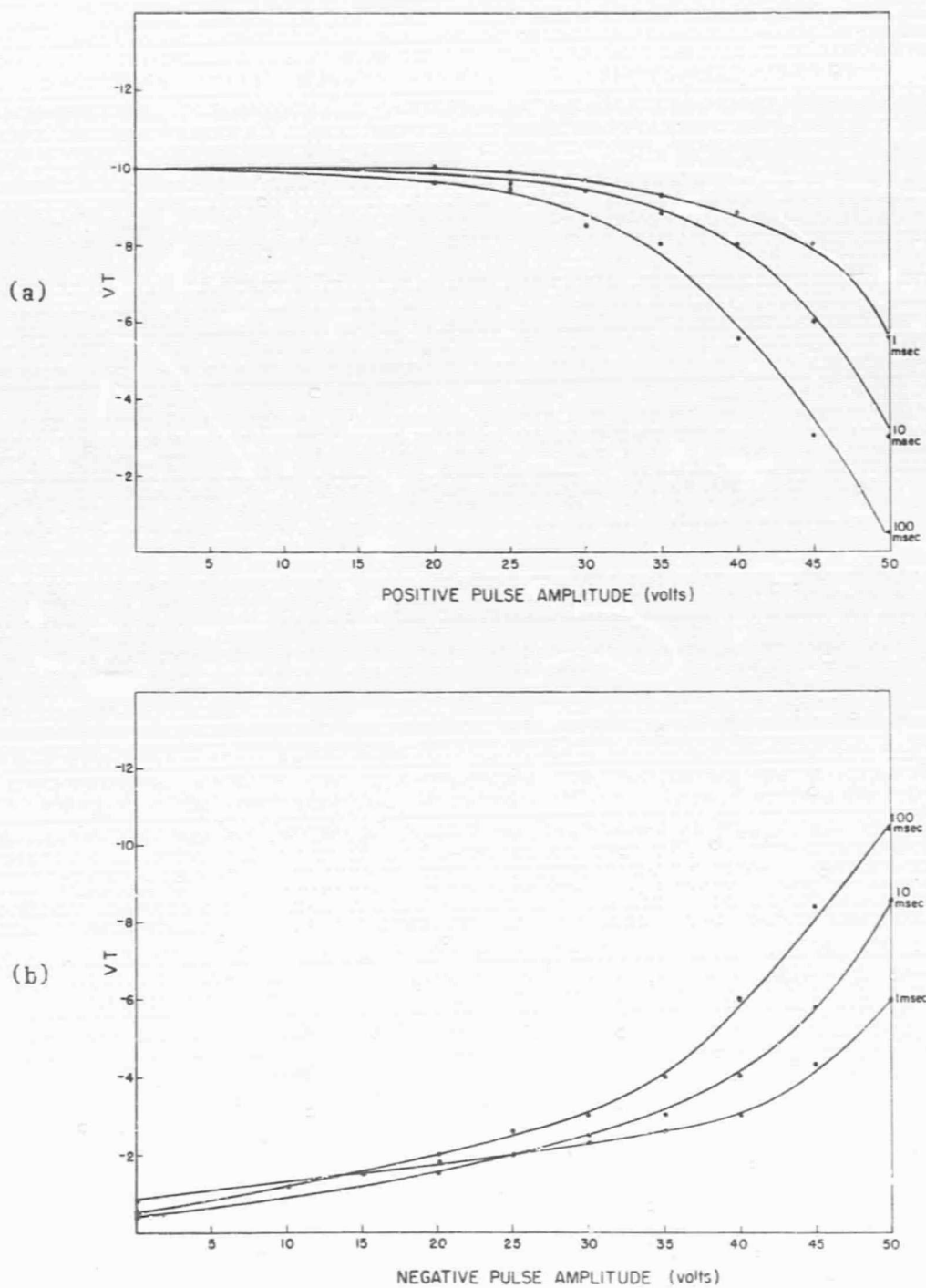
FIG. 8 (a) Threshold voltage V_T of MNS-VTT as a function of positive pulse amplitude and length. (b) Threshold voltage V_T of MNS-VTT as a function of negative pulse amplitude and length.
