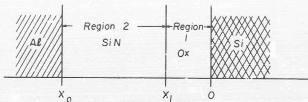
FIG. 25 Structure of memory capacitor.
