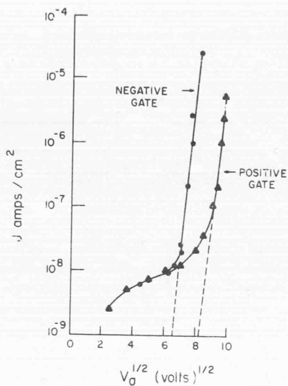
FIG. 16 Current vs voltage plot taken from MNS capacitor. Note the linear portion of \log J vs V^{1/2} .
