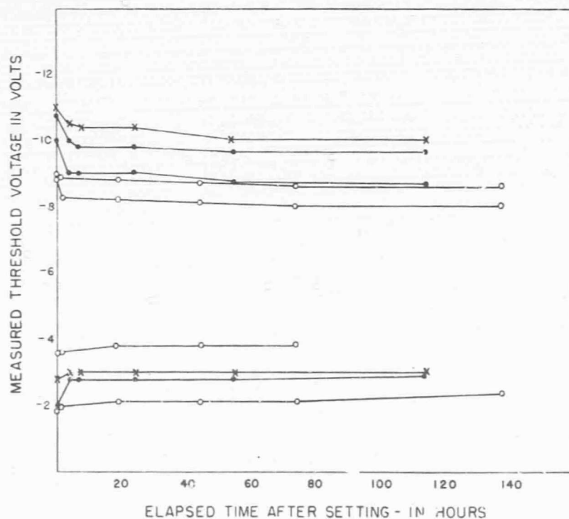
FIG. 10 Persistence of stored information: \circ 25°C, no bias on gate; \times +125°C, no bias on gate; \bullet +125°C, constant -5V bias on gate.
