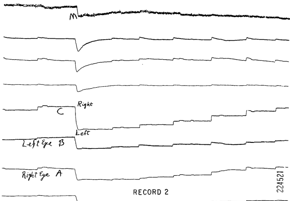
FIG.2 ELECTRO-OCULAR RECORDINGS
