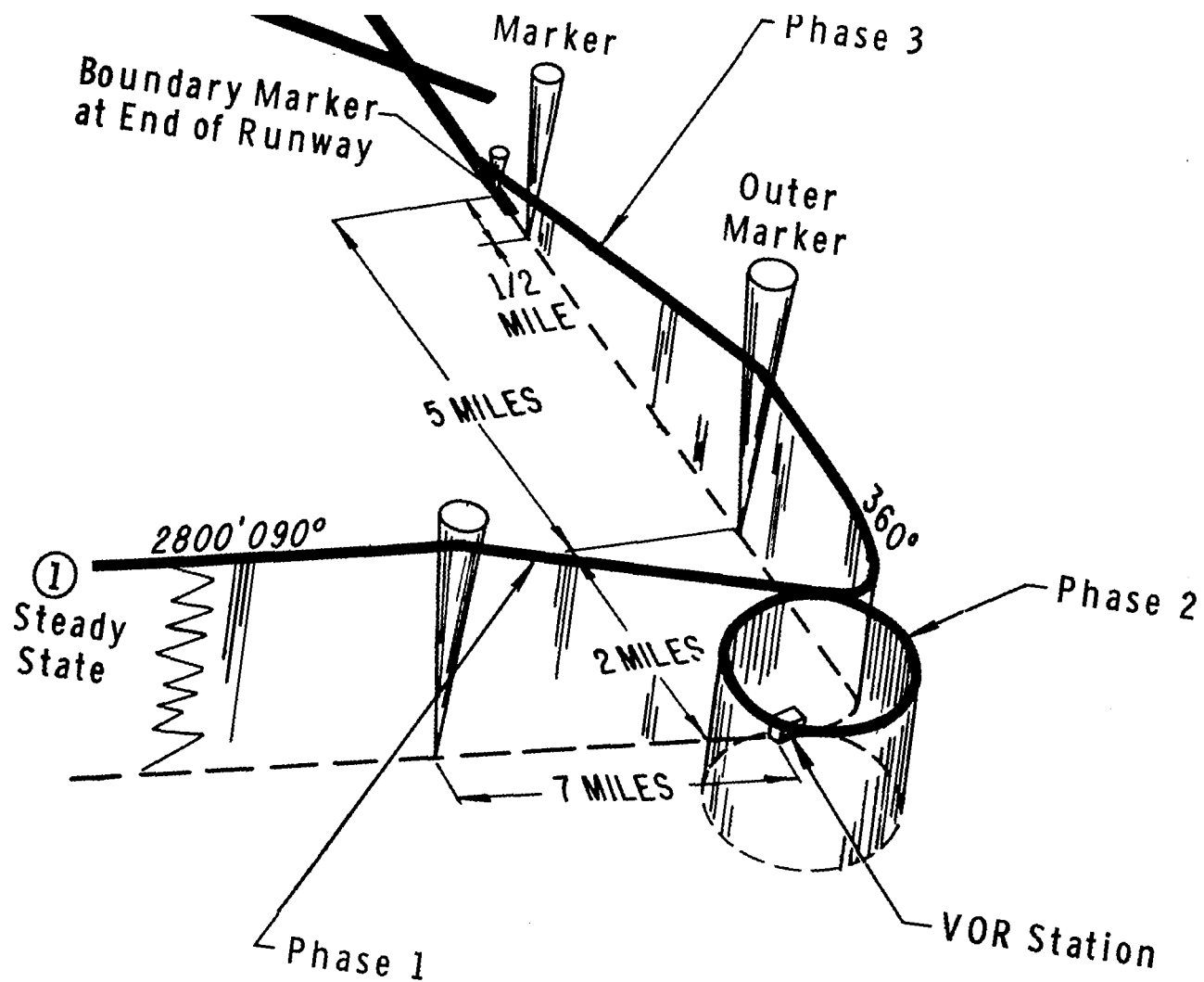
FIG. 3 FLIGHT PLAN
