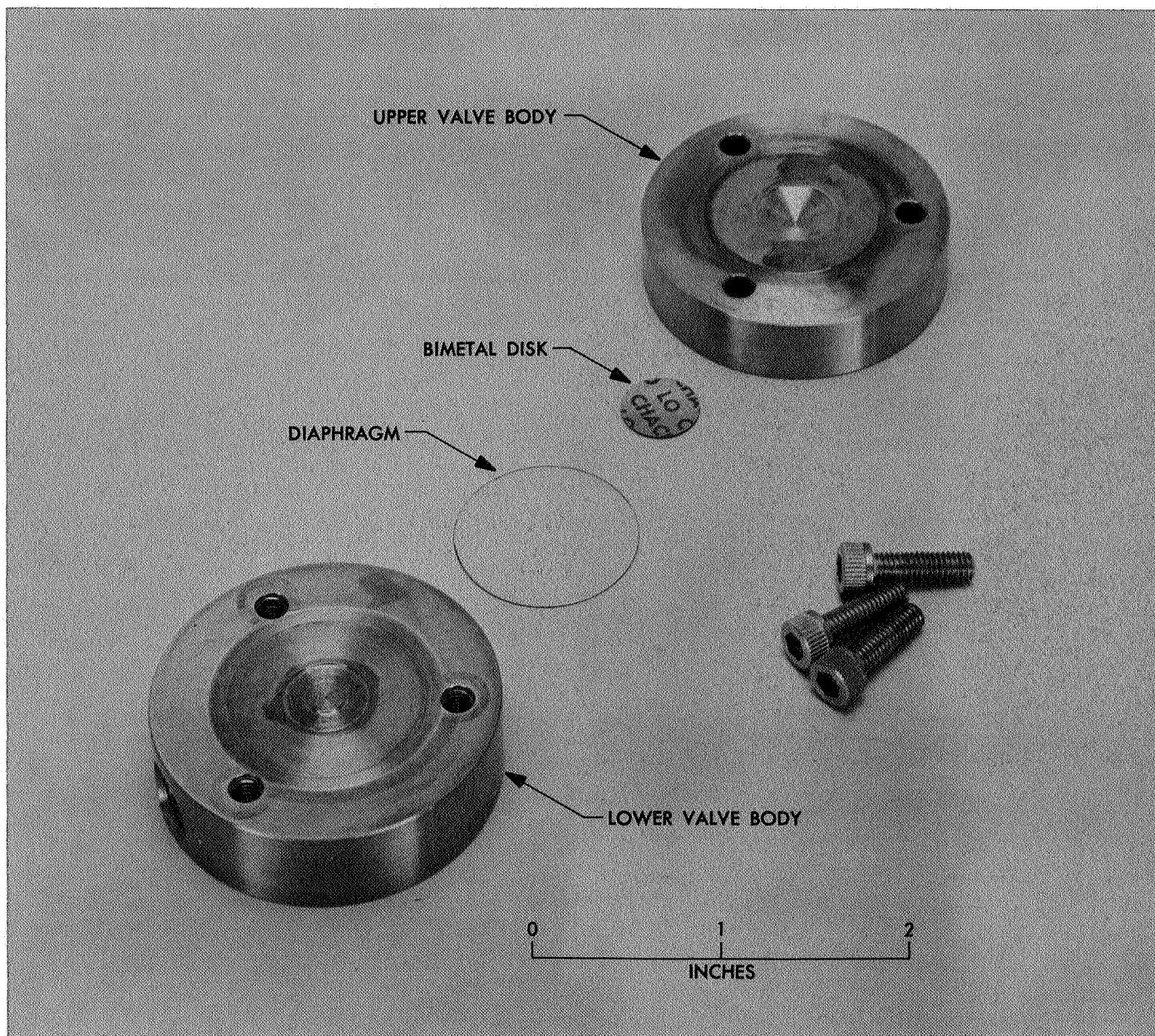
Fig. 3. Alternate temperature sensing and metering valve, disassembled
