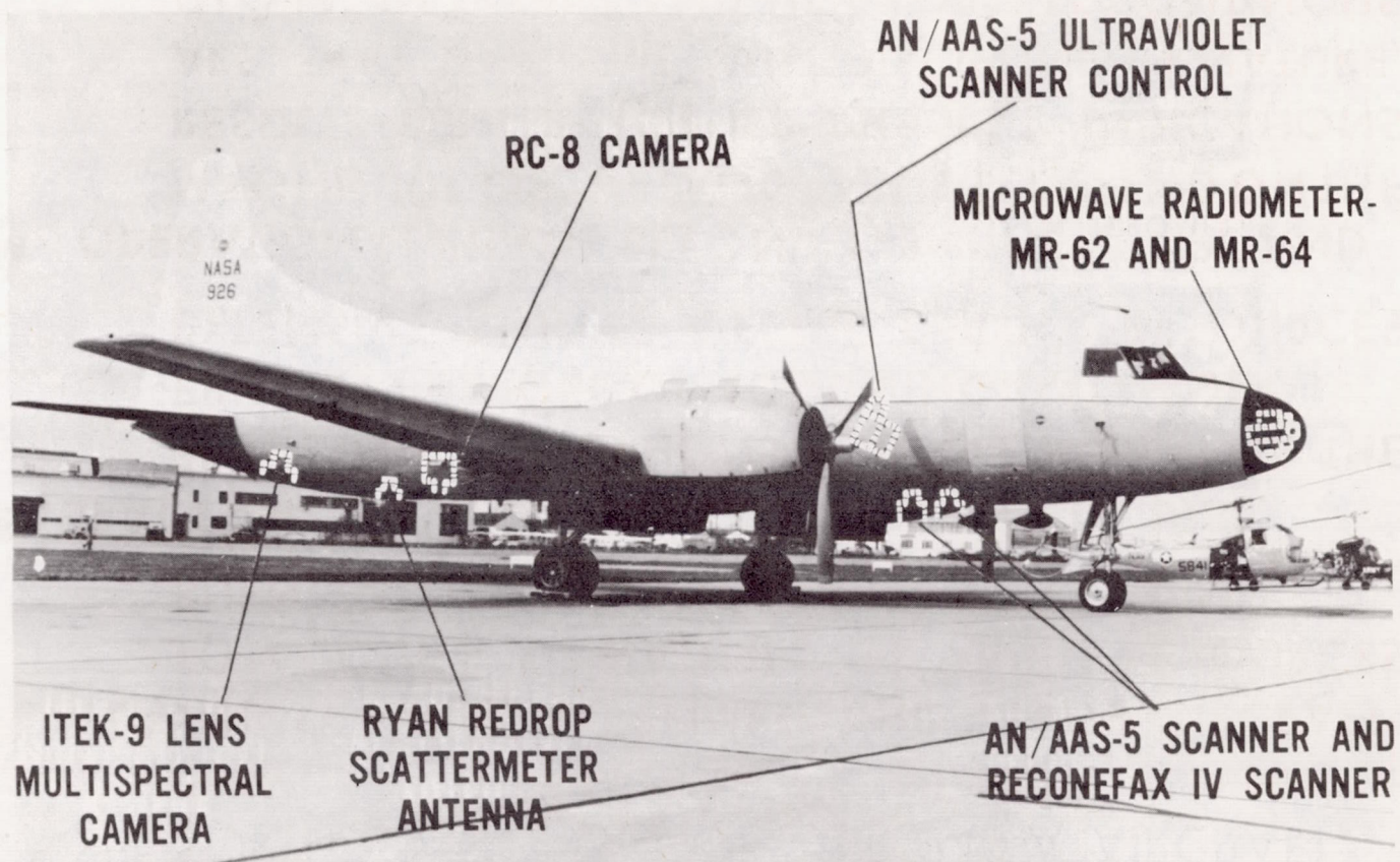
Figure 4.- Instrument locations on aircraft.
