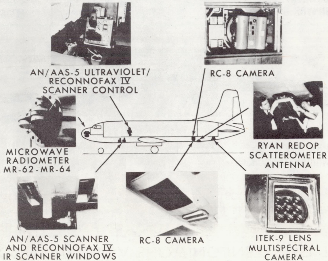
Figure 5.- Sensor locations.
