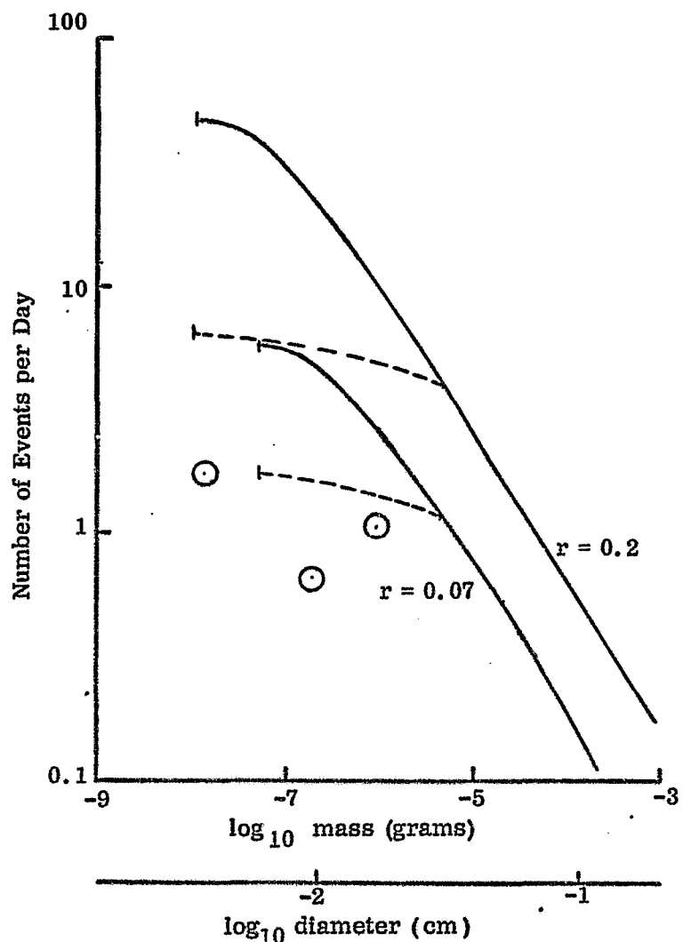
Figure 3. Data Return Rate
