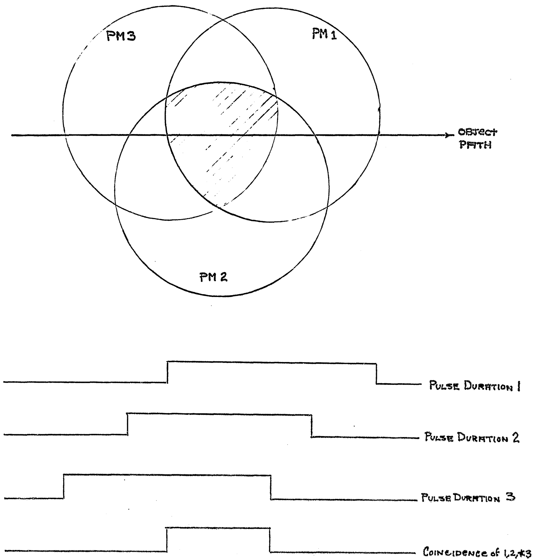
FIGURE 1. Method of Particle Detection
