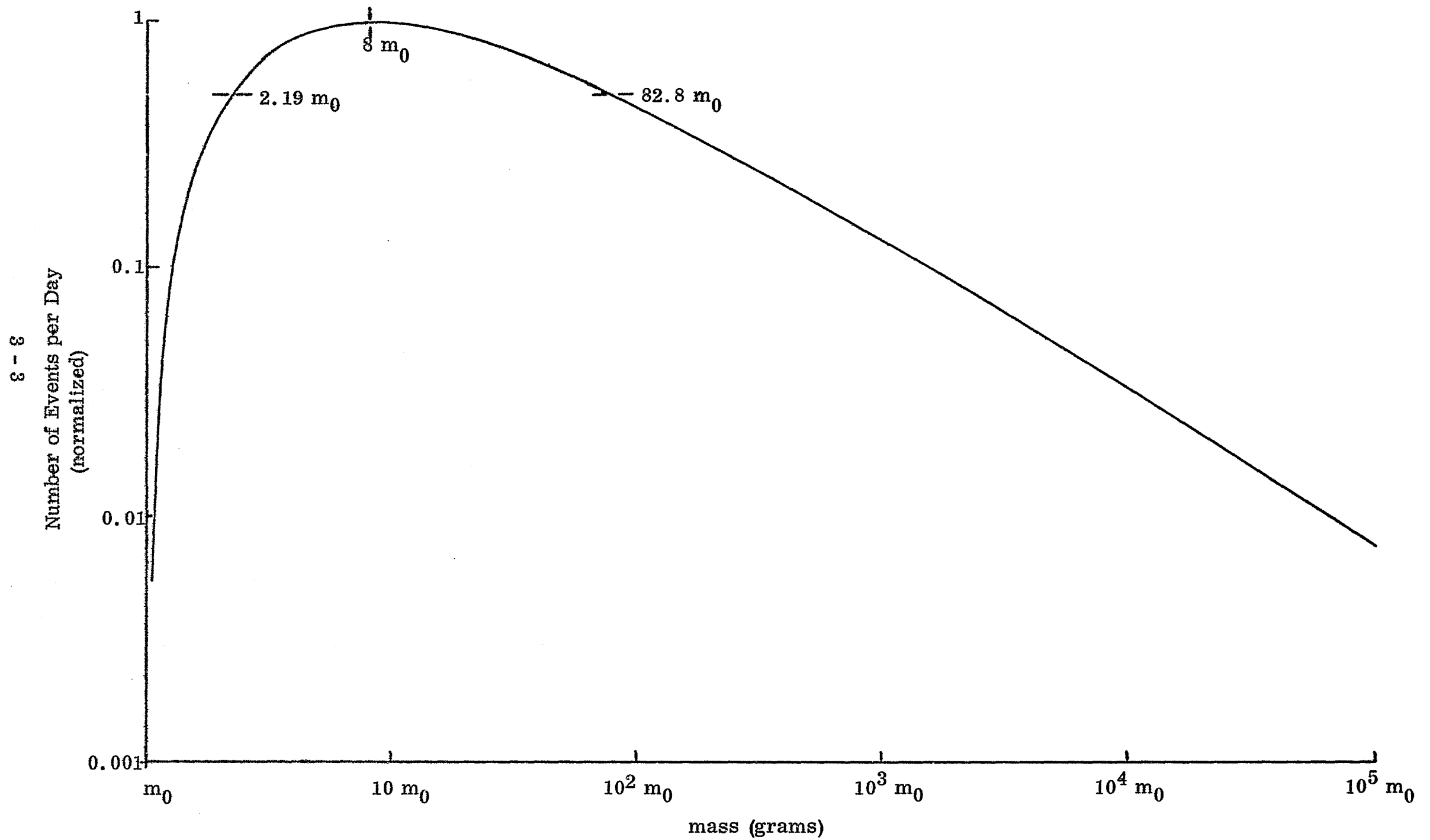
Figure 1. Sisyphus count rate vs. mass for an assumed meteoroid flux.
