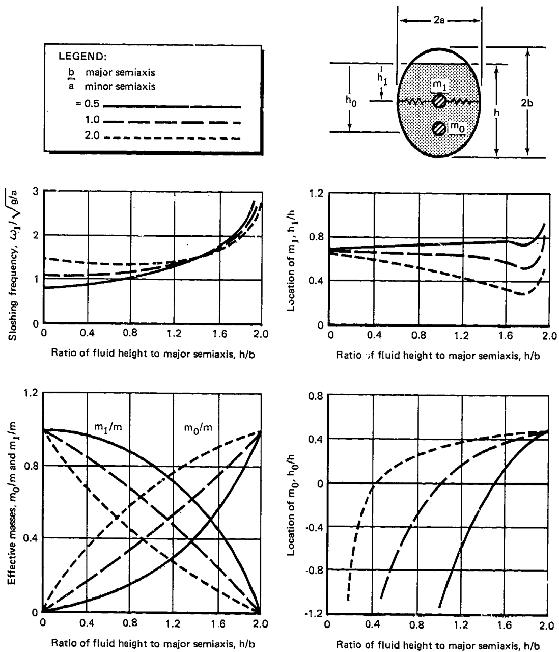
Figure 2 shows the mechanical model parameters for first-mode sloshing in an axisymmetric ellipsoidal tank for height-to-width ratios b/a of 2, 1 (spherical tank), and 0.5.
