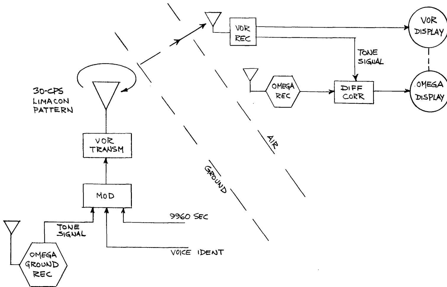
USE OF VOR LINK TO AIRCRAFT FOR TRANSMISSION OF OMEGA DIFFERENTIAL SIGNALS PROVIDING COMBINED RADIAL-PARALLEL OBLIQUE GRID REFERENCED TO VOR STATION COORDINATES
