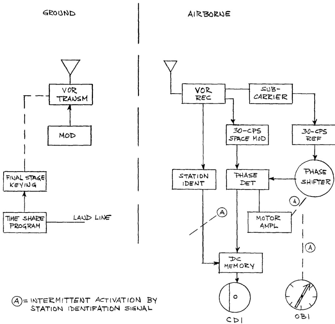
STORAGE OF INTERMITTENT VOR BEARINGS USING SERVO MEMORY AND/OR DC MEMORY
