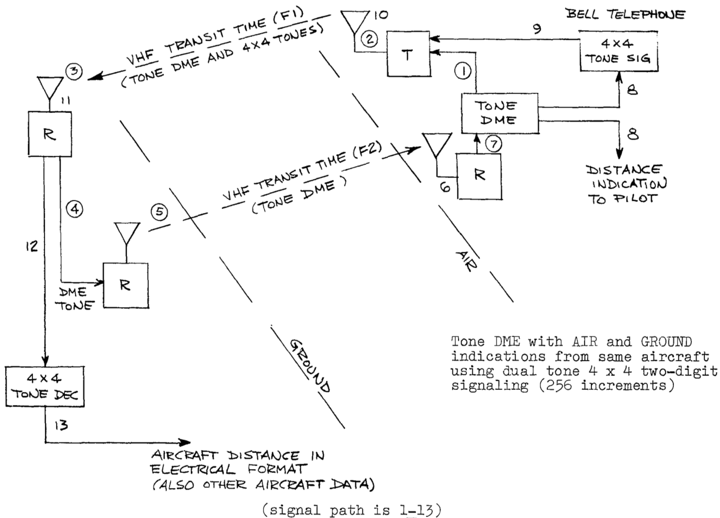
TONE DME WITH AIR AND GROUND OUTPUTS
