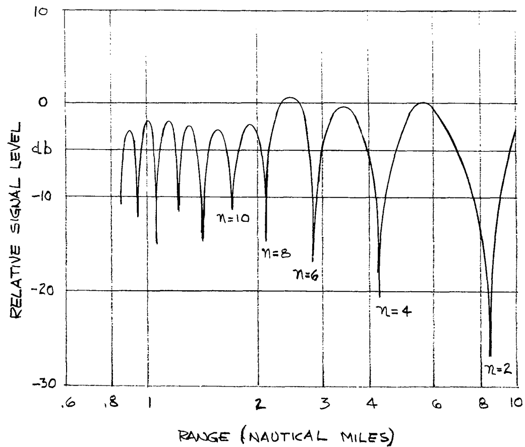
POSITION AND DEPTH OF VERTICAL NULLS FOR ANTENNA 26 FEET ABOVE GROUND
