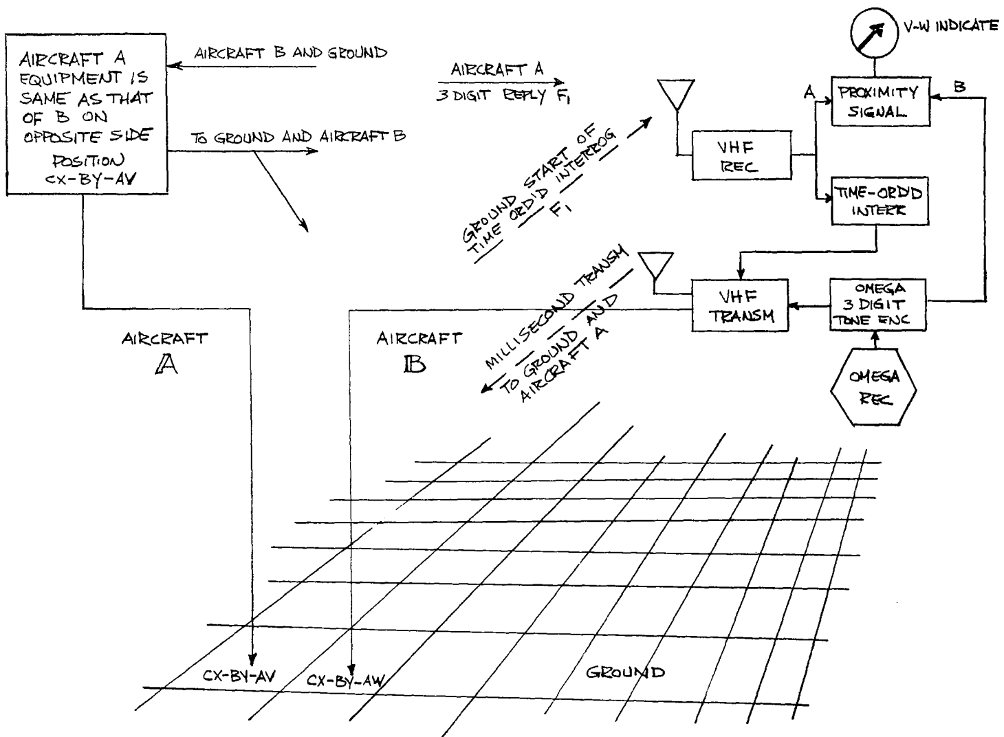
POSSIBLE INTEGRATION OF TIME-ORDERED POSITION REPORTING OF OMEGA COORDINATES FOR GROUND DISPLAY, PROCESSING, AND PROXIMITY SIGNALING TO AIRCRAFT IN ADJACENT POSITION
