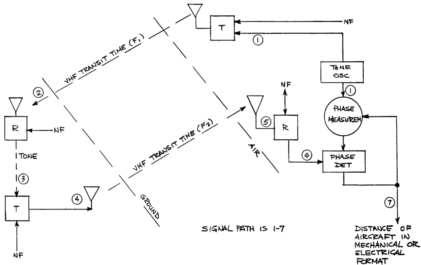
TONE DISTANCE MEASUREMENT (OUTPUT AT AIRBORNE SOURCE)
