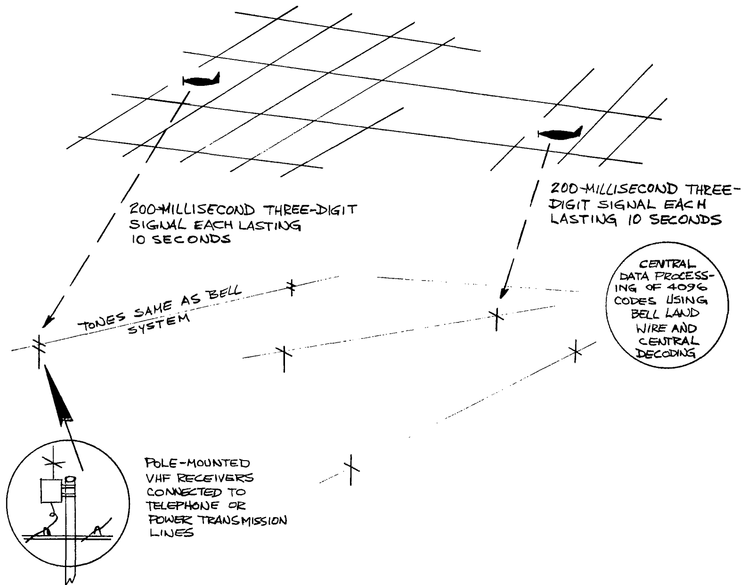
AUTOMATIC POSITION REPORTING USING BELL DUAL-TONE SIGNALING SYSTEM ON NATIONAL BASIS (LOW-COST GENERAL AVIATION AIRCRAFT ONLY)
