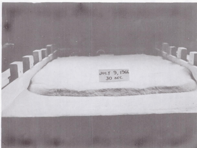
Fig. 62 View of Intersection of Failure Surface with Surface of Backfill - 18 in. High Wall, Dense Test
