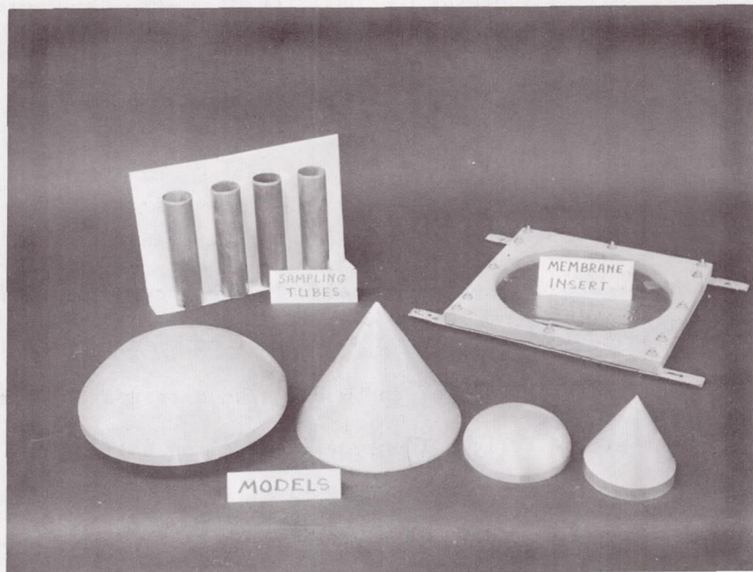
Fig. 31 View of Models, Sampling Tubes, and Lateral Soil Support - Phase III
