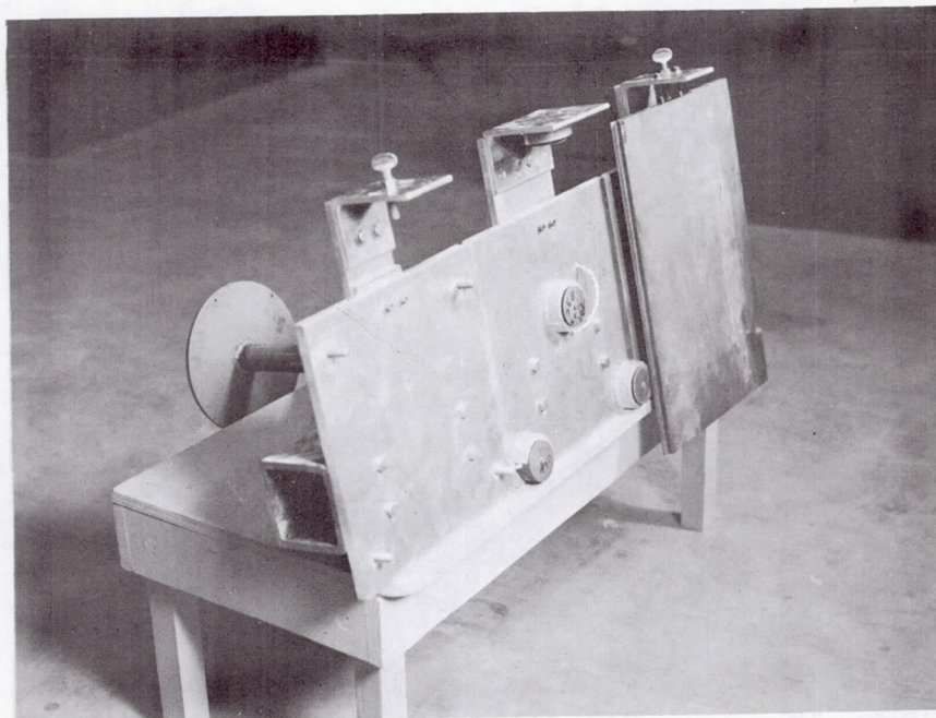
Fig. 22 View of Loading Frame and Plate Supports - Phase II
