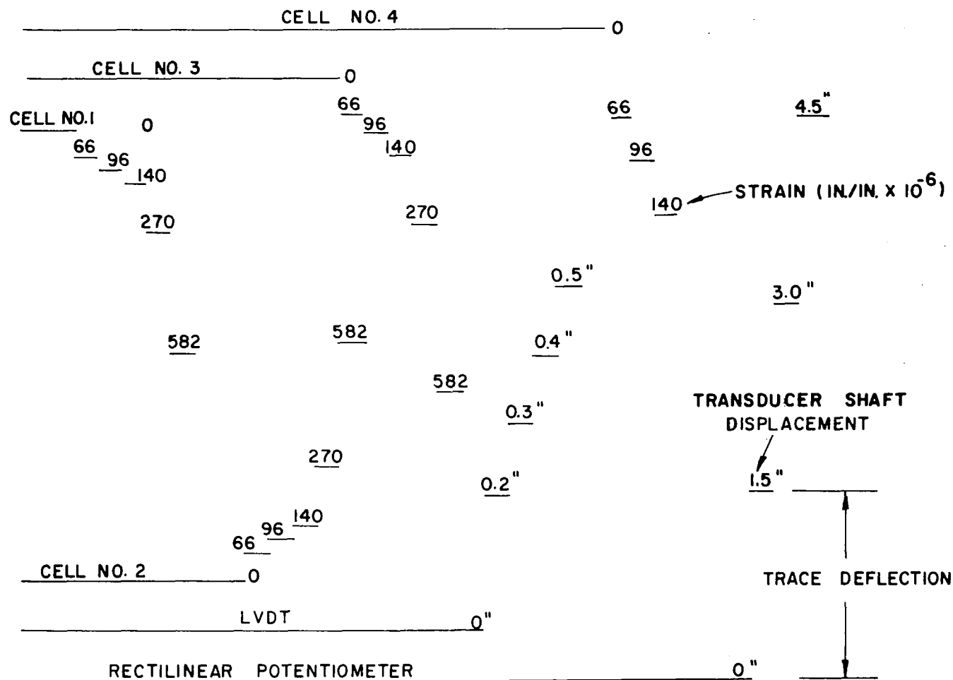
FIG.34 TYPICAL CALIBRATION DATA OUTPUT -PHASE II
