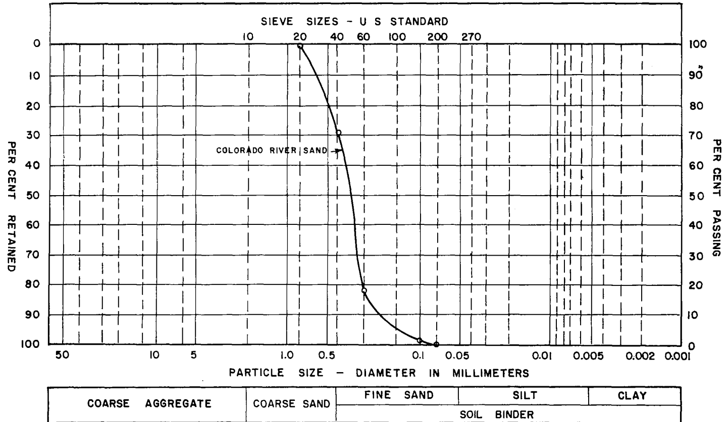
FIG.38 MECHANICAL ANALYSIS GRAIN SIZE ACCUMULATIVE CURVE
