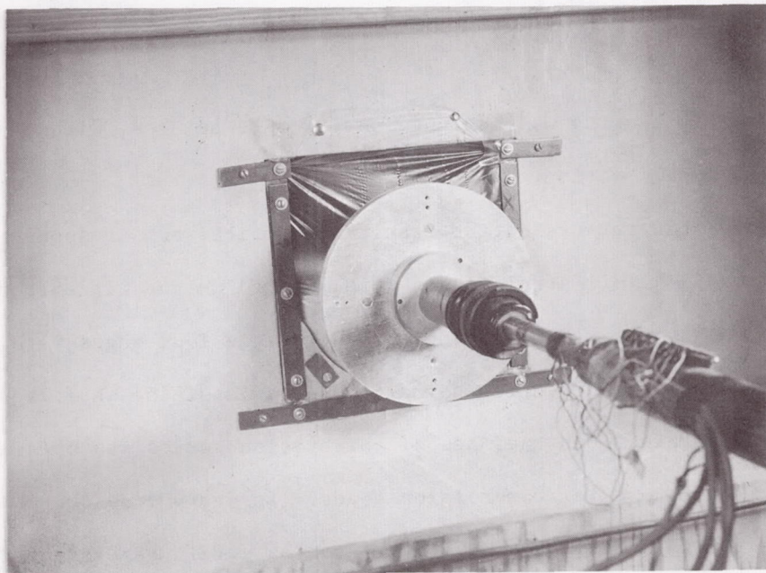
Fig. 32 Rear View of Instrumented Shaft and Spherical Segment in Initial Test Position - Phase III
