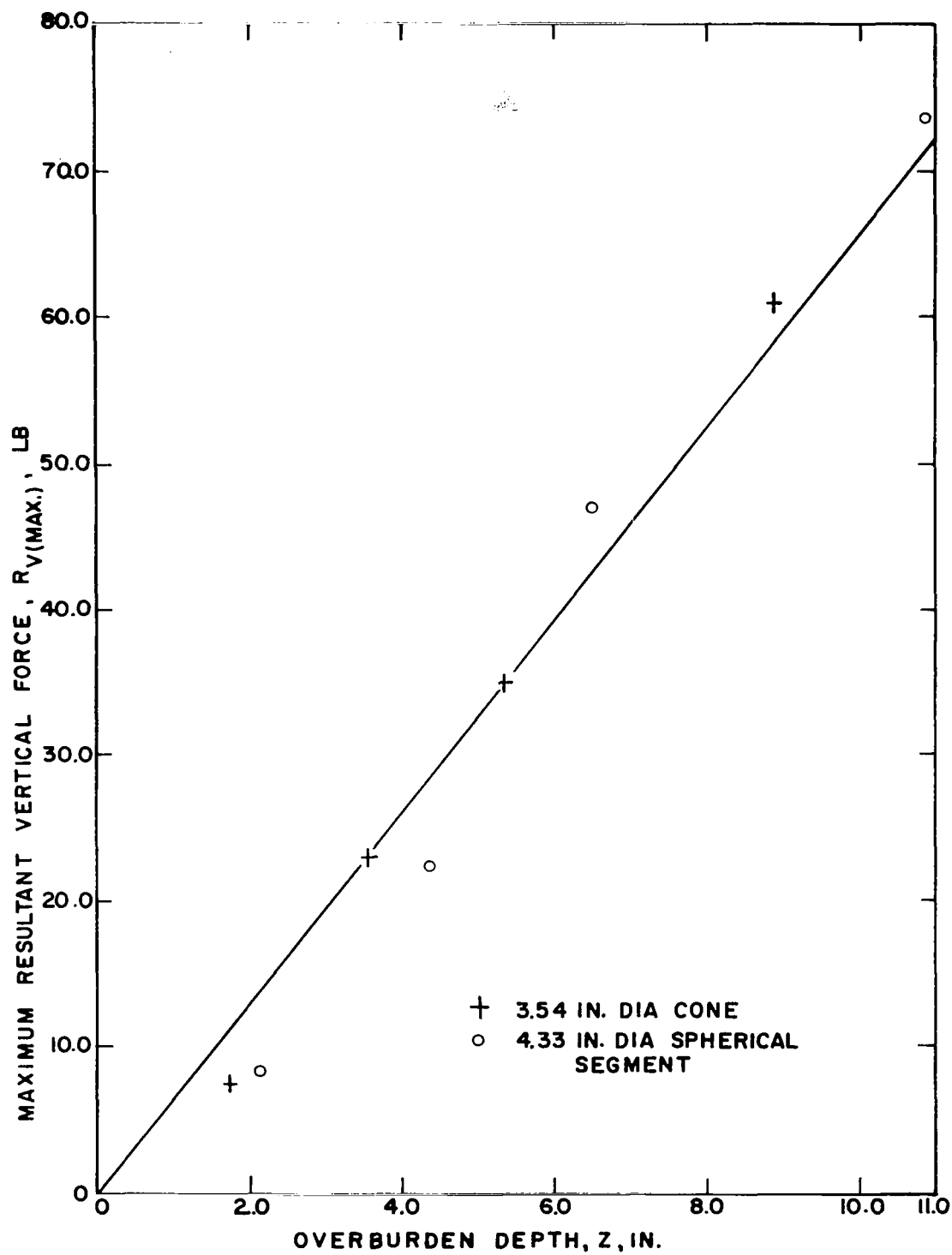
FIG.84 EFFECT OF OVERBURDEN DEPTH ON THE MAXIMUM DEVELOPED RESULTANT VERTICAL FORCE-DENSE CASE
