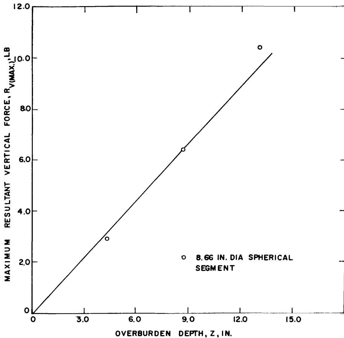
FIG.87 EFFECT OF OVERBURDEN DEPTH ON THE MAXIMUM DEVELOPED RESULTANT VERTICAL FORCE-LOOSE CASE
