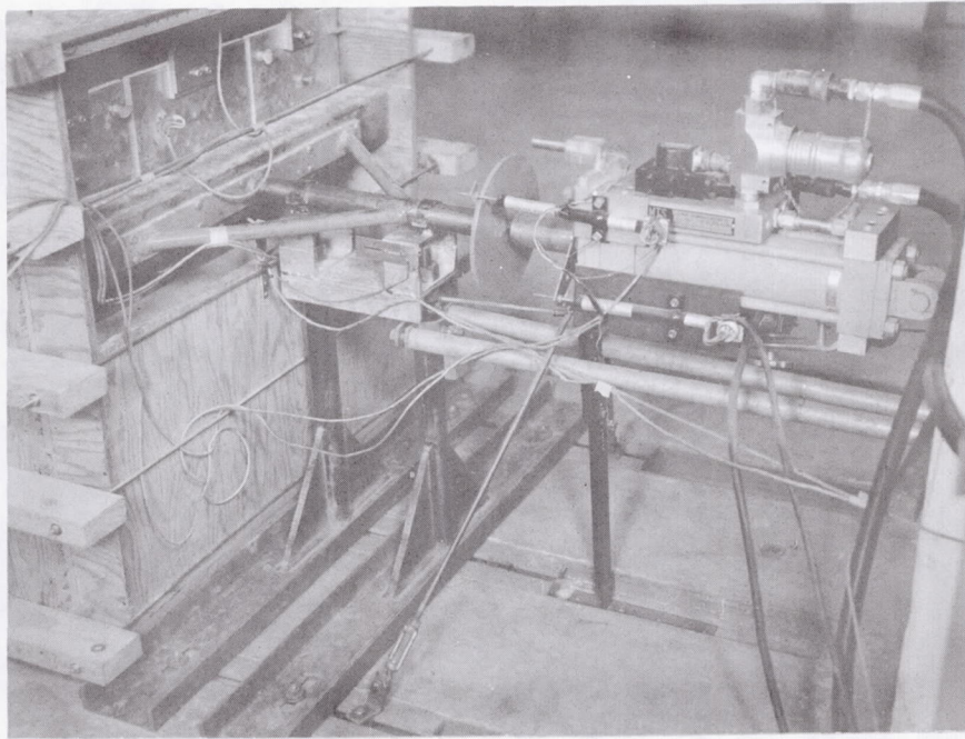
Fig. 27 Detail View of Loading Frame Restraint and Deflection Transducer Mountings
