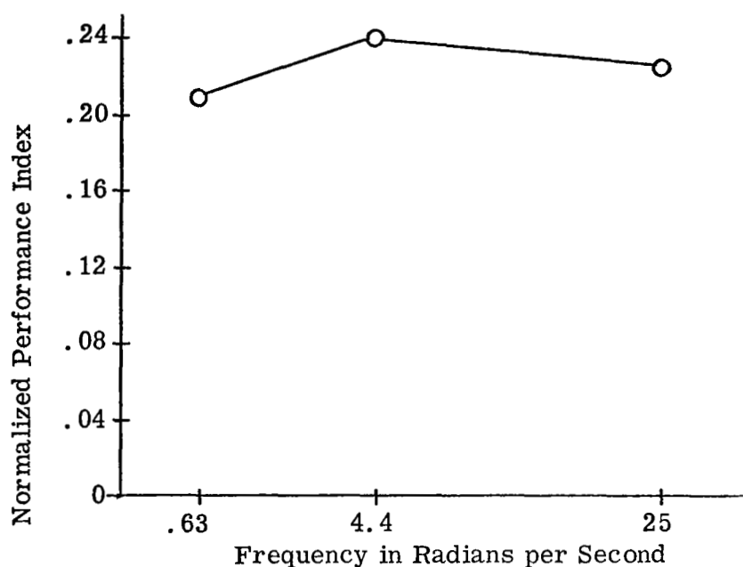
Figure 3.3.3 Tracking Performance as a Function of Sinusoidal Variation of the Spring Constant.
