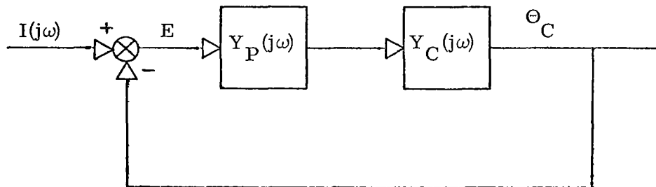
Figure 2.2.2 Generalized Control System as Used in Table 2.2.1.
