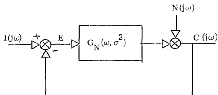
Figure C.3 Inclusion of Remnant Noise to Account for Uncorrelated Power in the Output Signal
