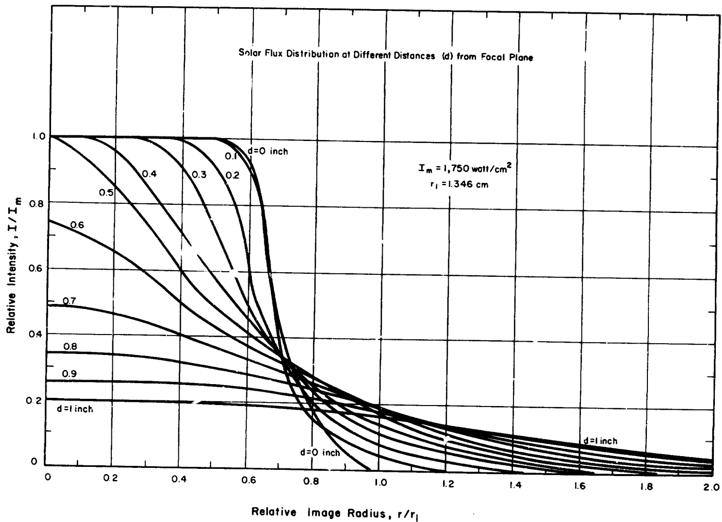
Figure B-1. Solar Flux Distribution at Different Distances from Focal Plane.
