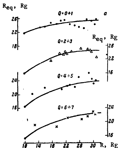
Fig.1. Dependence of the equatorial semiaxis R_{eq} of magnetosphere tail's cross-section on the geocentric distance R .
