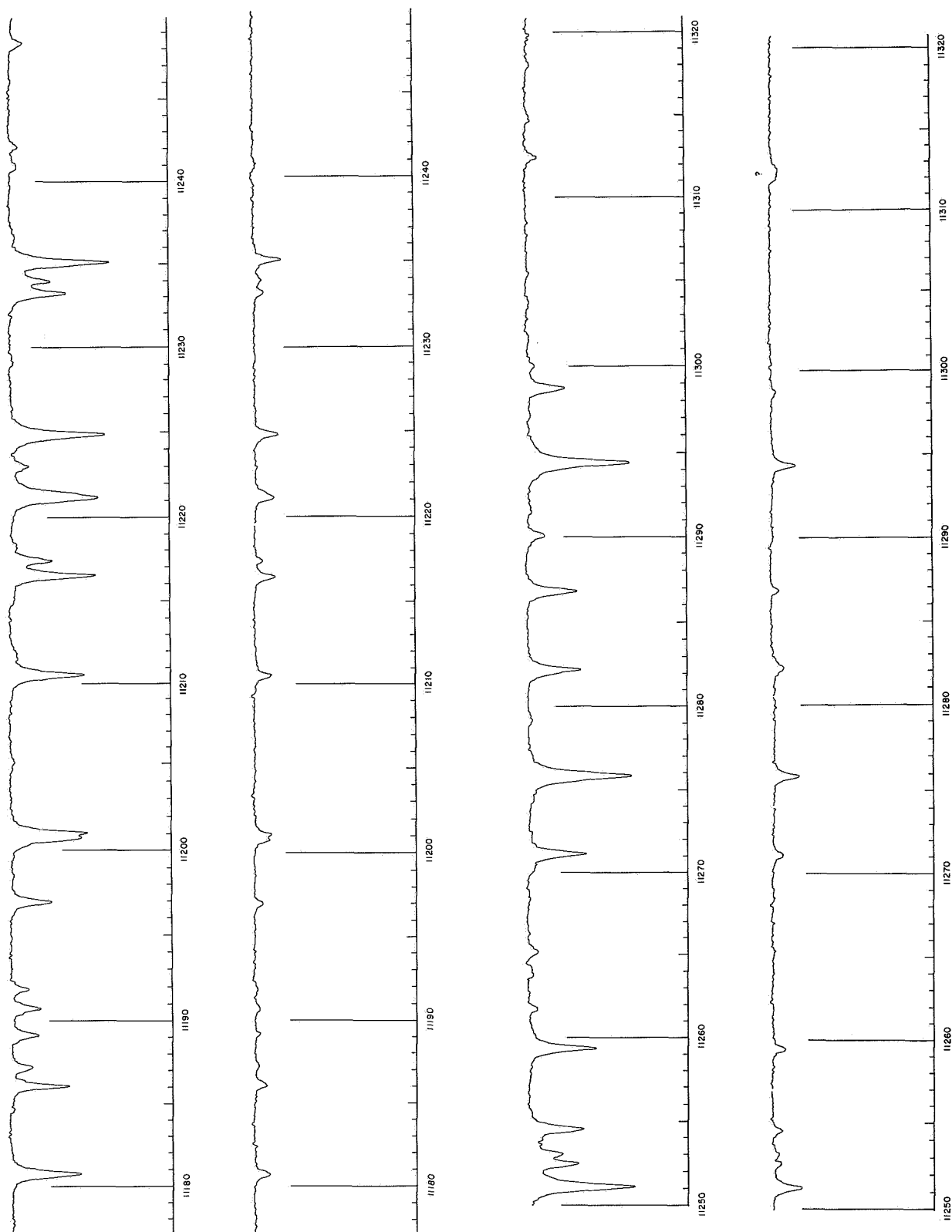
Fig. 2A Laboratory spectrum of water vapor, \lambda\lambda 11177–11321 Å.
