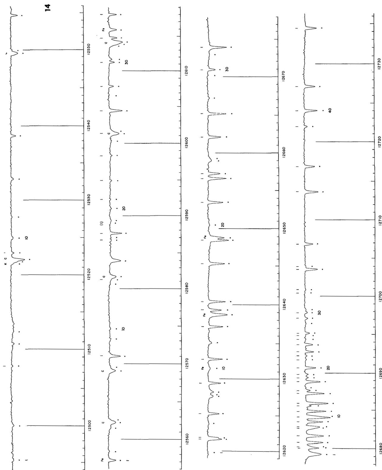
Fig. 8 Solar Spectrum \lambda\lambda 12494–12736, in four strips (cf. Table 1).
