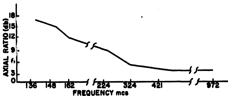
Fig. 13 HEMI SPIRAL AXIAL RATIO
