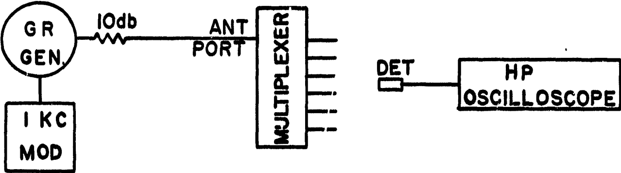
Fig. 20 MEASUREMENT DURING VIBRATION TEST
