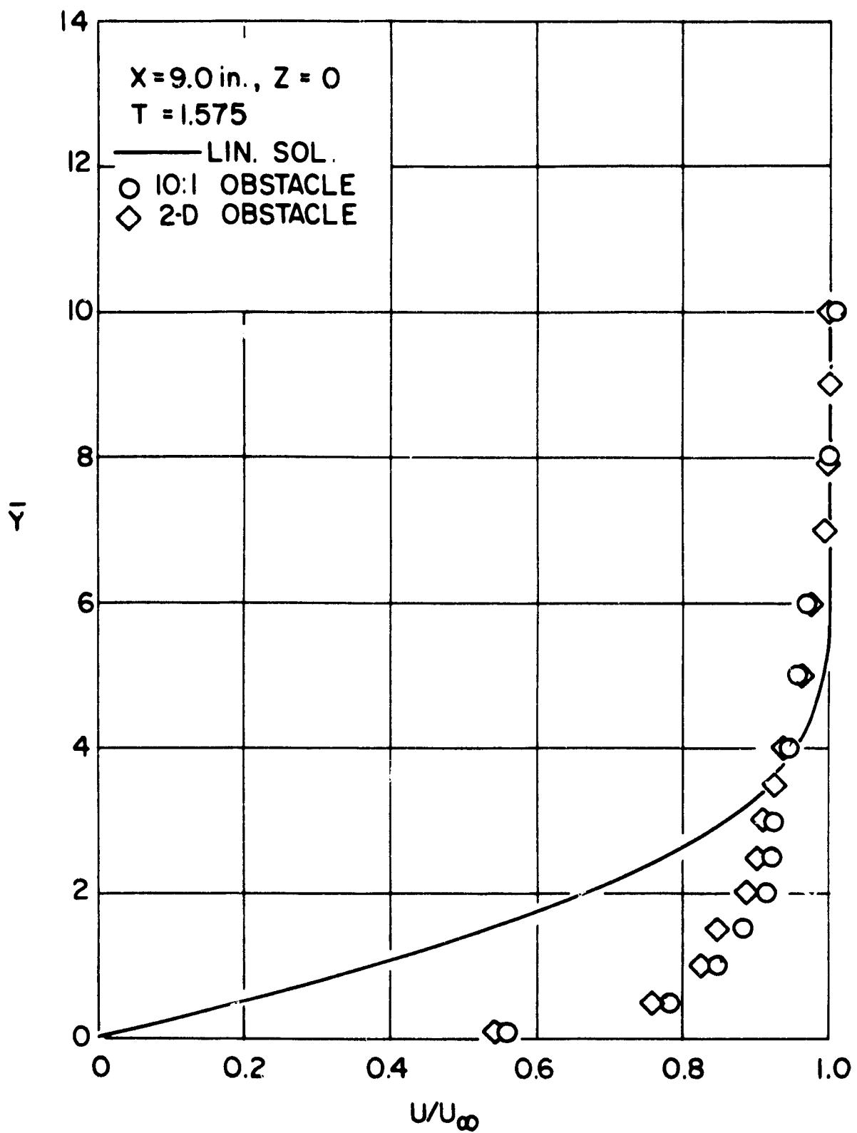
FIG. 24 NORMAL PROFILE AT X = 9.0 \text{ IN.} COMPARED TO LINEARIZED THEORY
