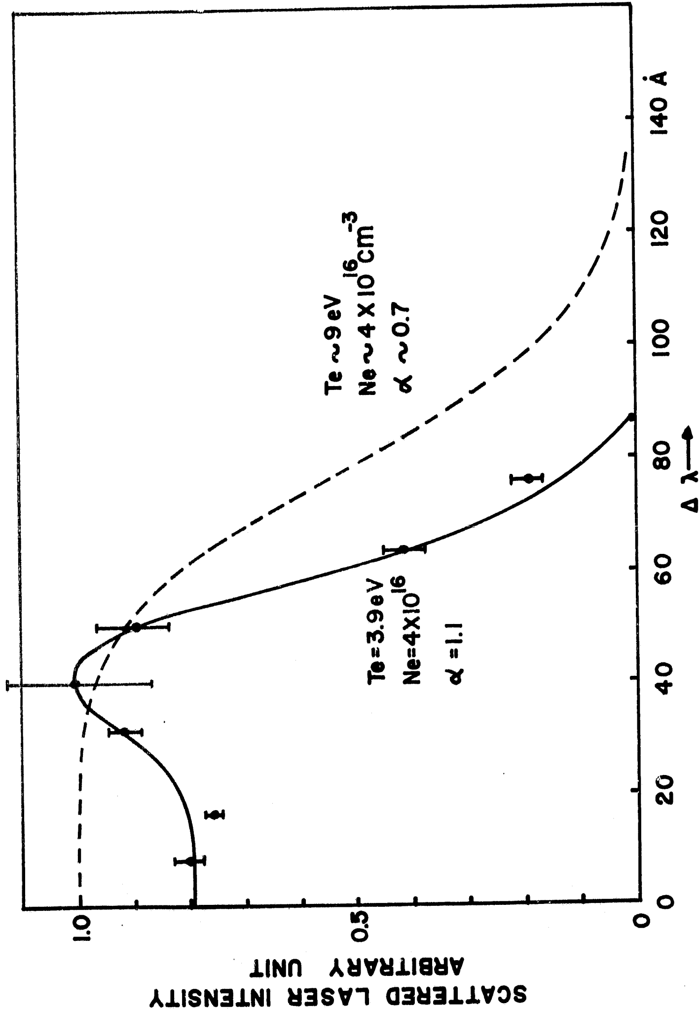
FIG. 5 SPECTRUM OF SCATTERED LASER RADIATION BEHIND THE INCIDENT SHOCK AT t = 1.0 \mu\text{sec} , \text{He} at 1 TORR
