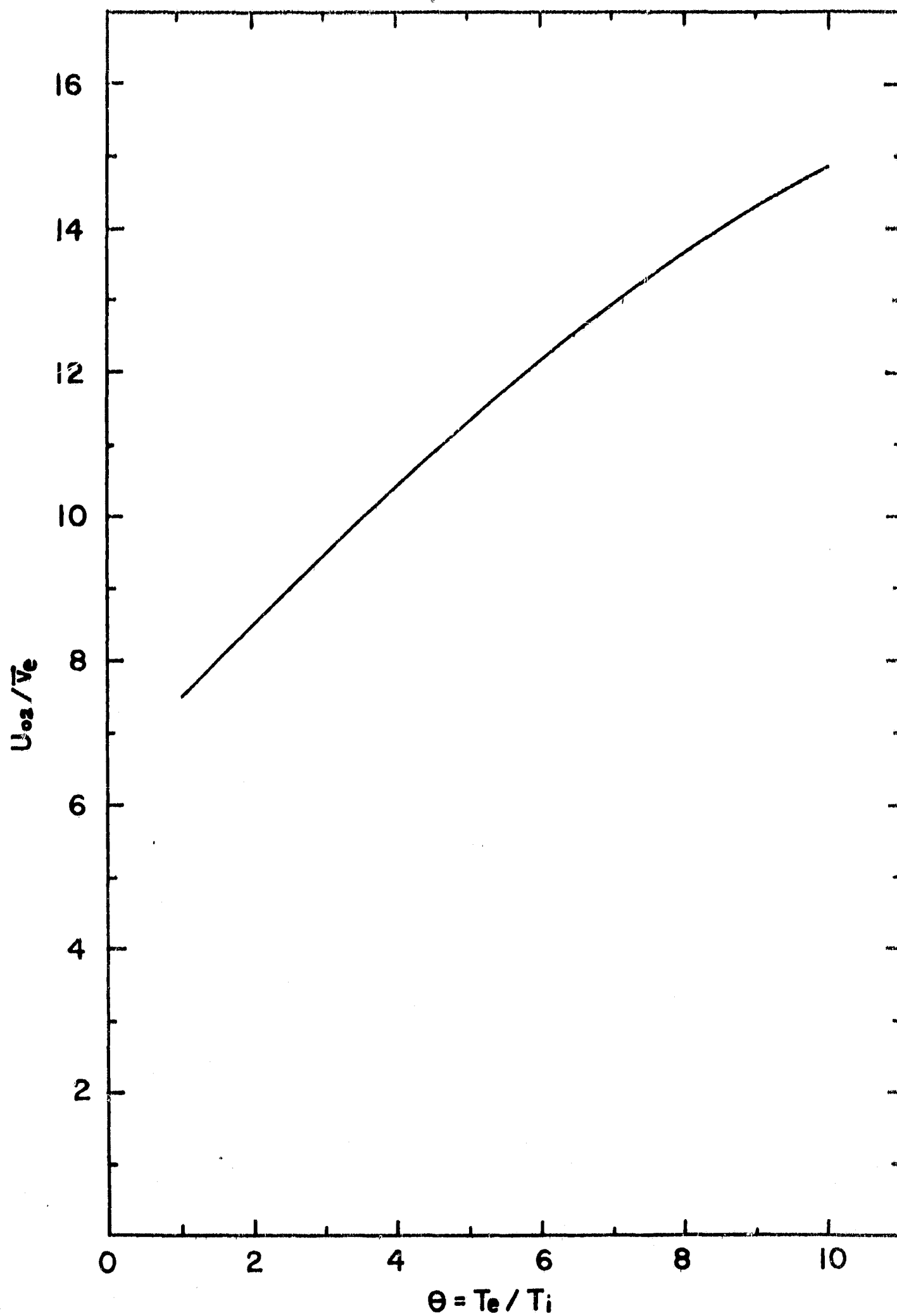
FIG. 15 SAME AS FIG. 14 EXCEPT FOR THE NORMALIZED UPPER VELOCITY THRESHOLD U_{02}/\bar{v}_e
