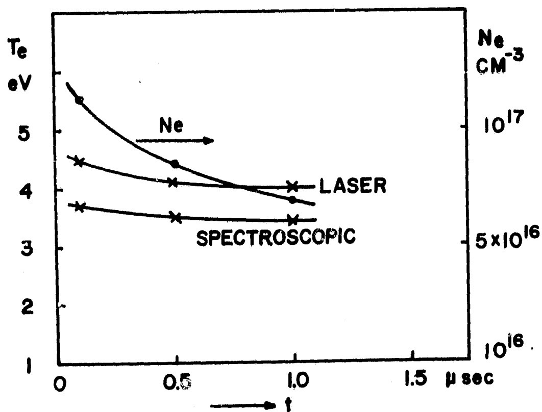
FIG. 11 ELECTRON DENSITY AND TEMPERATURE BEHIND THE REFLECTED SHOCK
