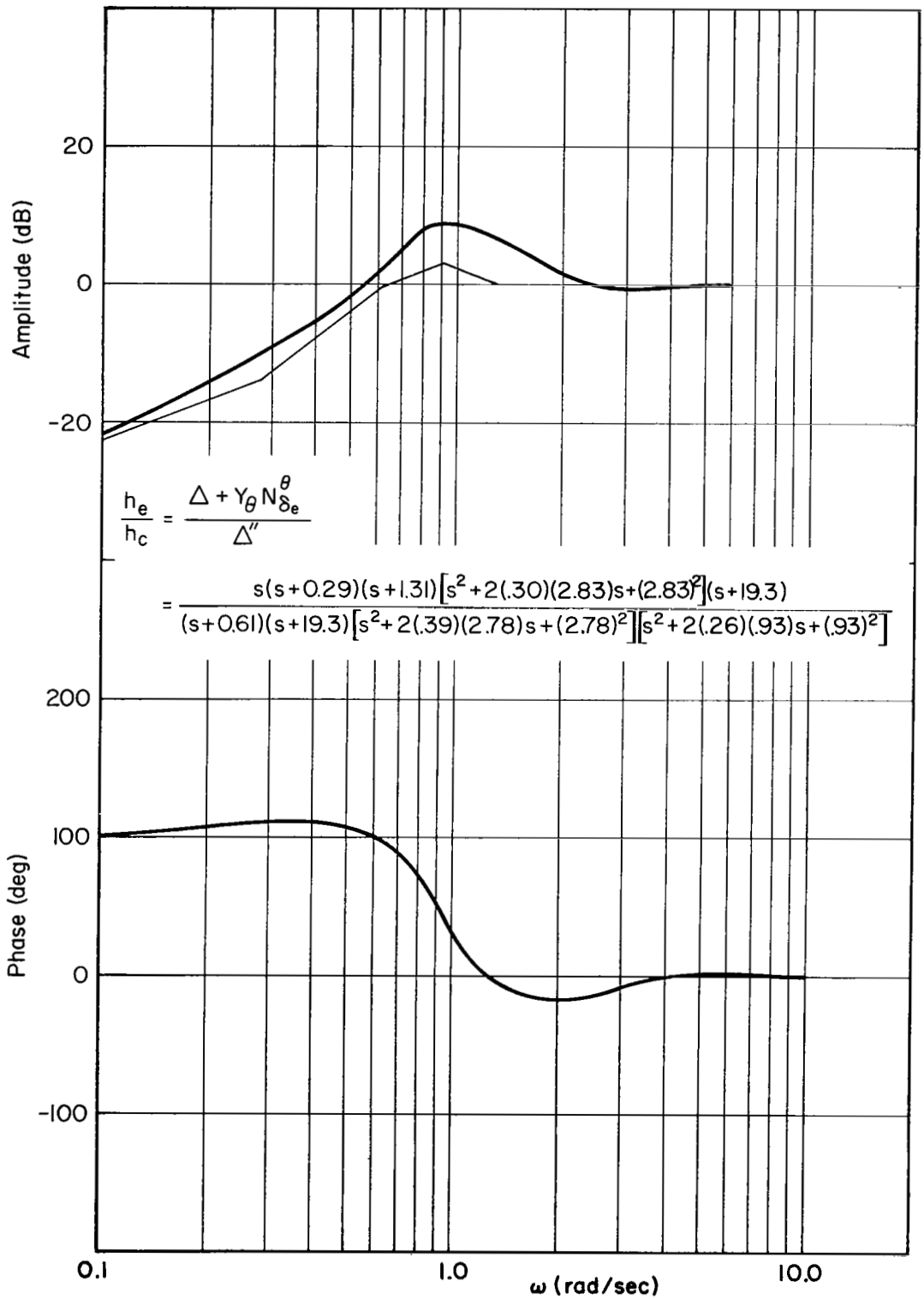
Figure C-9. Predicted Closed-Loop Response, h_e/h_c
