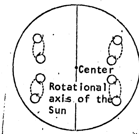
Figure 2. Illustration of the Kinematics of Sunspots. Instantaneous Position of the Vortex Tubes (According to Bjerknes) in a Section Through the Axis of Rotation. The Slow Meridional Circulation Postulated, Which Leads the Vortex Tubes About Each Other in 2 \times 11 Years, is Shown by Broken Lines.
