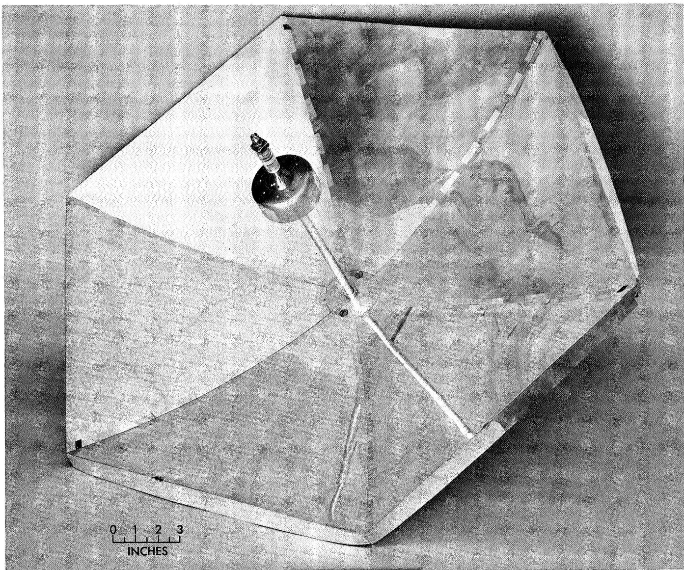
Fig. 2. Six-rib model erectable reflector
