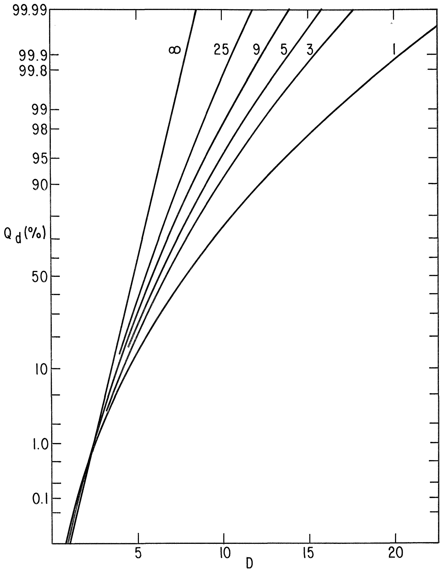
Fig. 6. Probability Q_d of detection versus signal-to-noise ratio N_s/\sqrt{N'M'} for various values of N'M' . Q_o = 10^{-6} .
