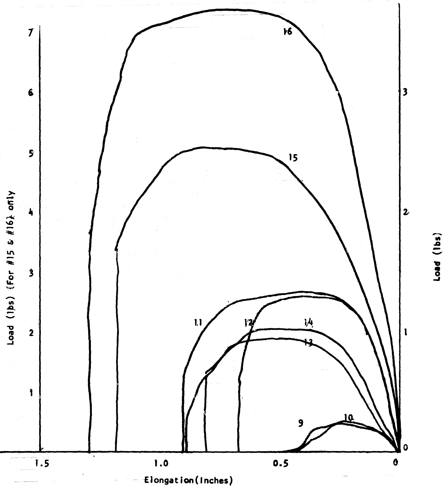
Figure 33. Tensile-Elongation Curves for Teflon-Bonded Matrices
