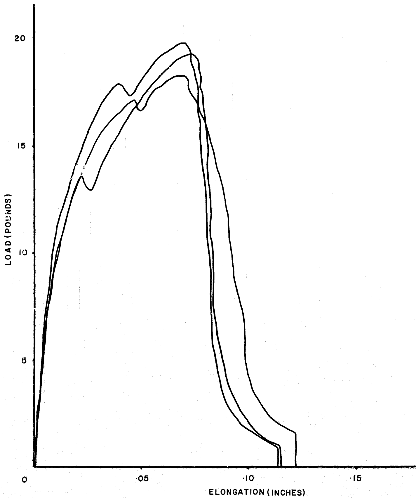
Figure 9. Tensile-Elongation Curves for 60 Mil Fuel Cell Asbestos Board (no. 2702) Stress Applied Transverse to Processing Direction.
