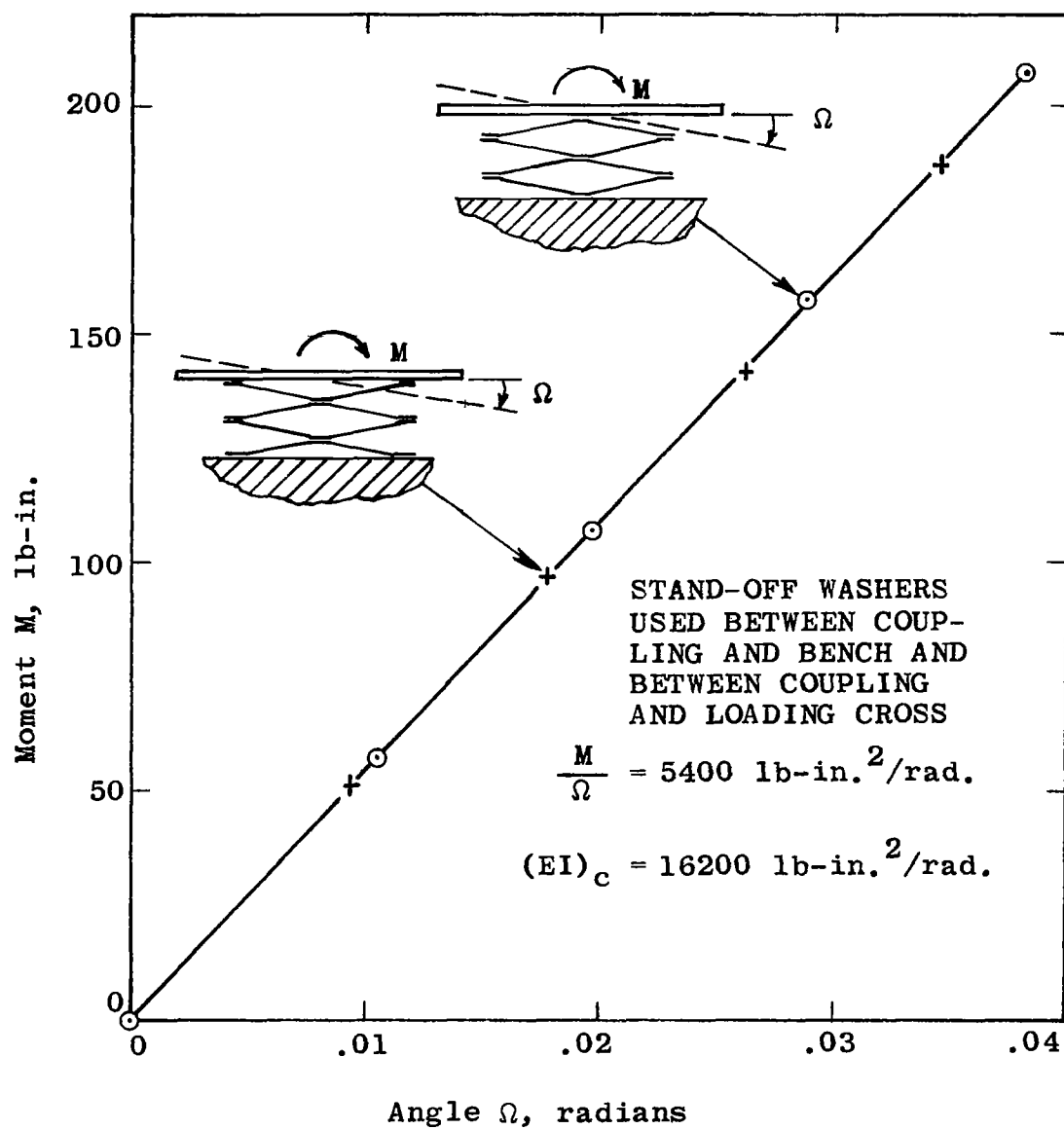
Figure 11. Experimental Moment-Rotation Curves
