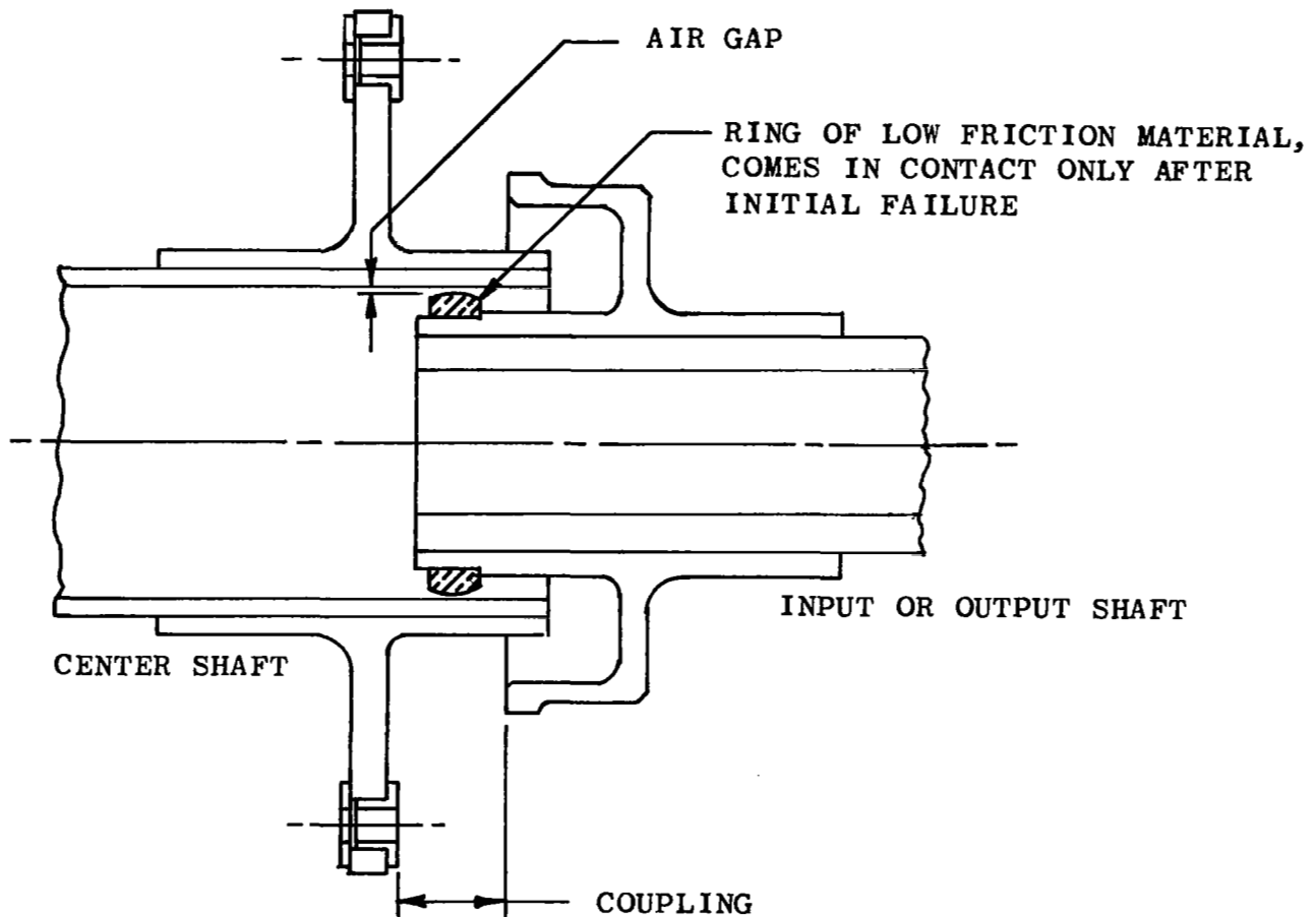
Figure 32. Fail-Safe Design
