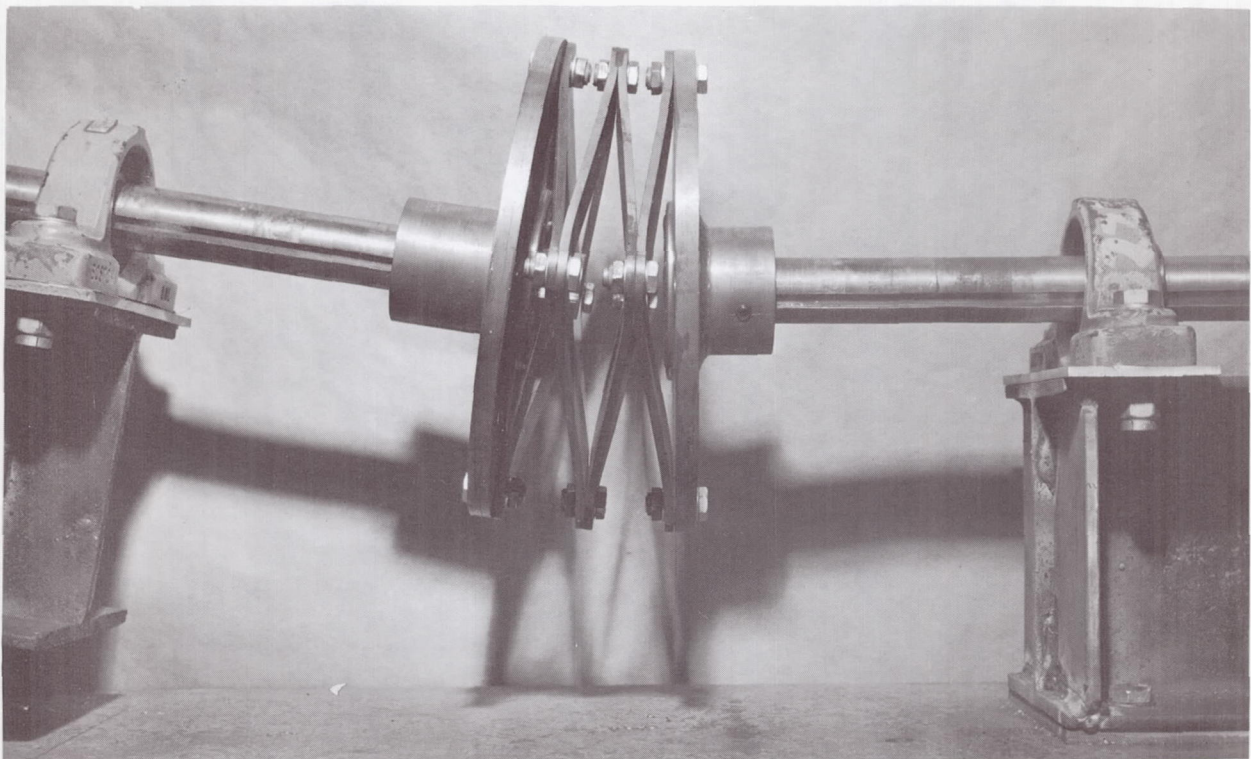
Figure 18. Fatigue Test
