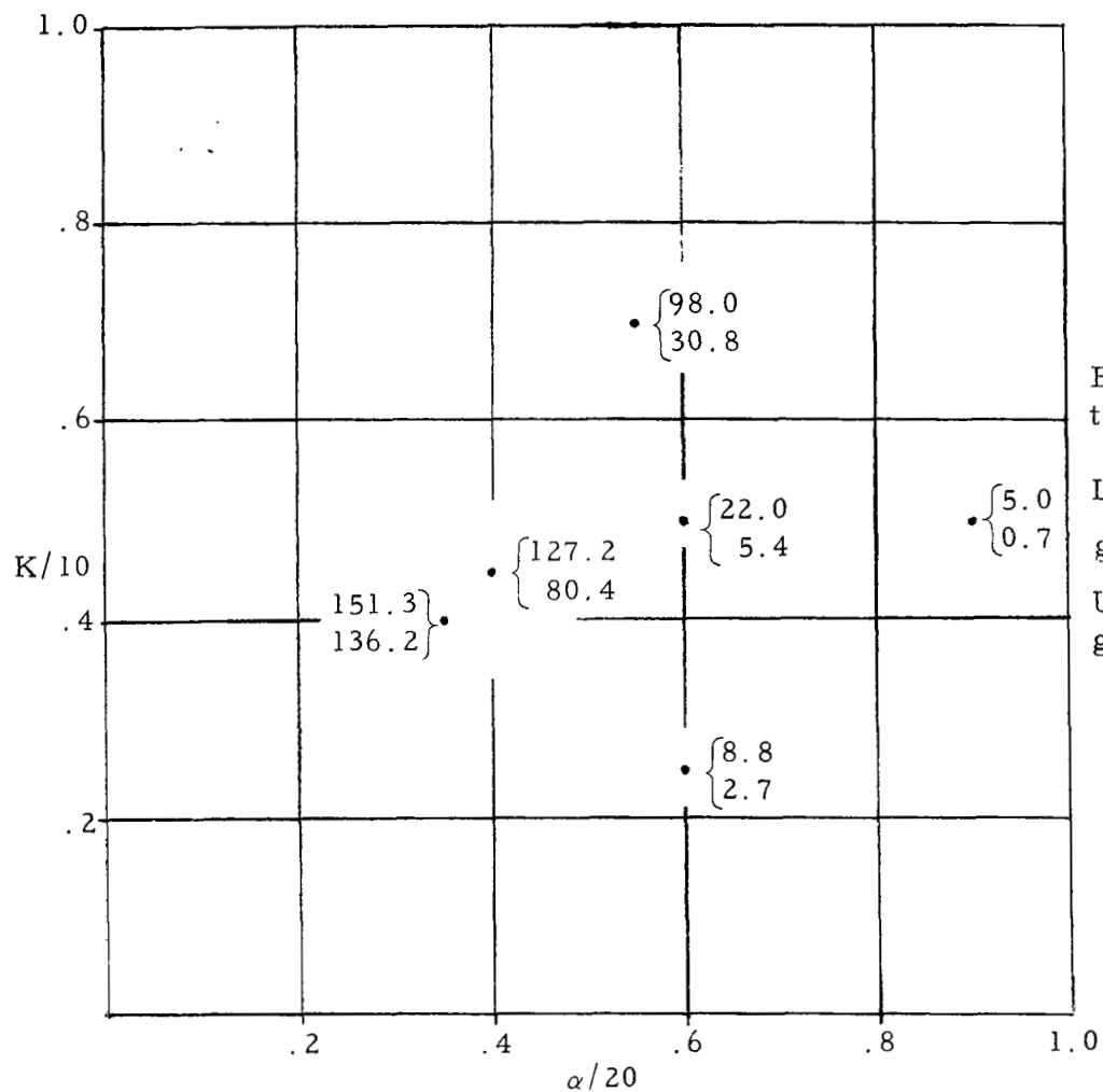
Figure 3.5-2 Comparison of Values of \int_0^T u_2^2 dt for Fixed Gain and Variable Gain on u_2(t)
