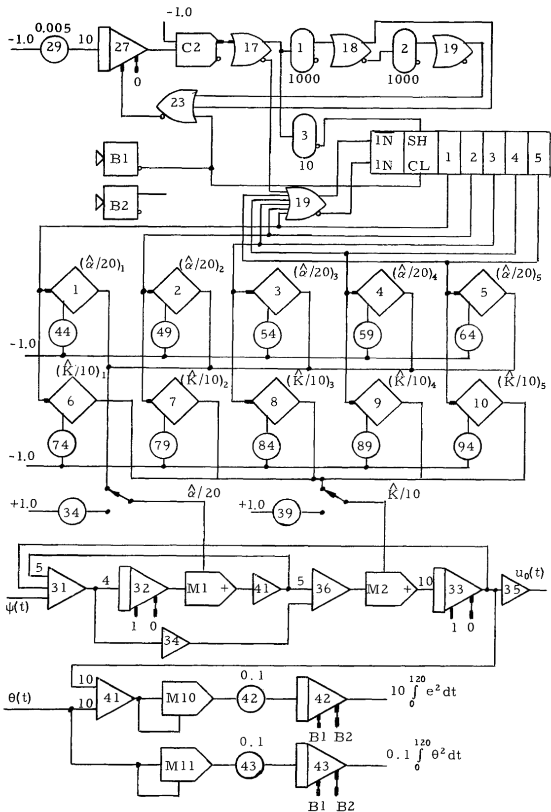
Figure A-15 Power Match Circuitry
