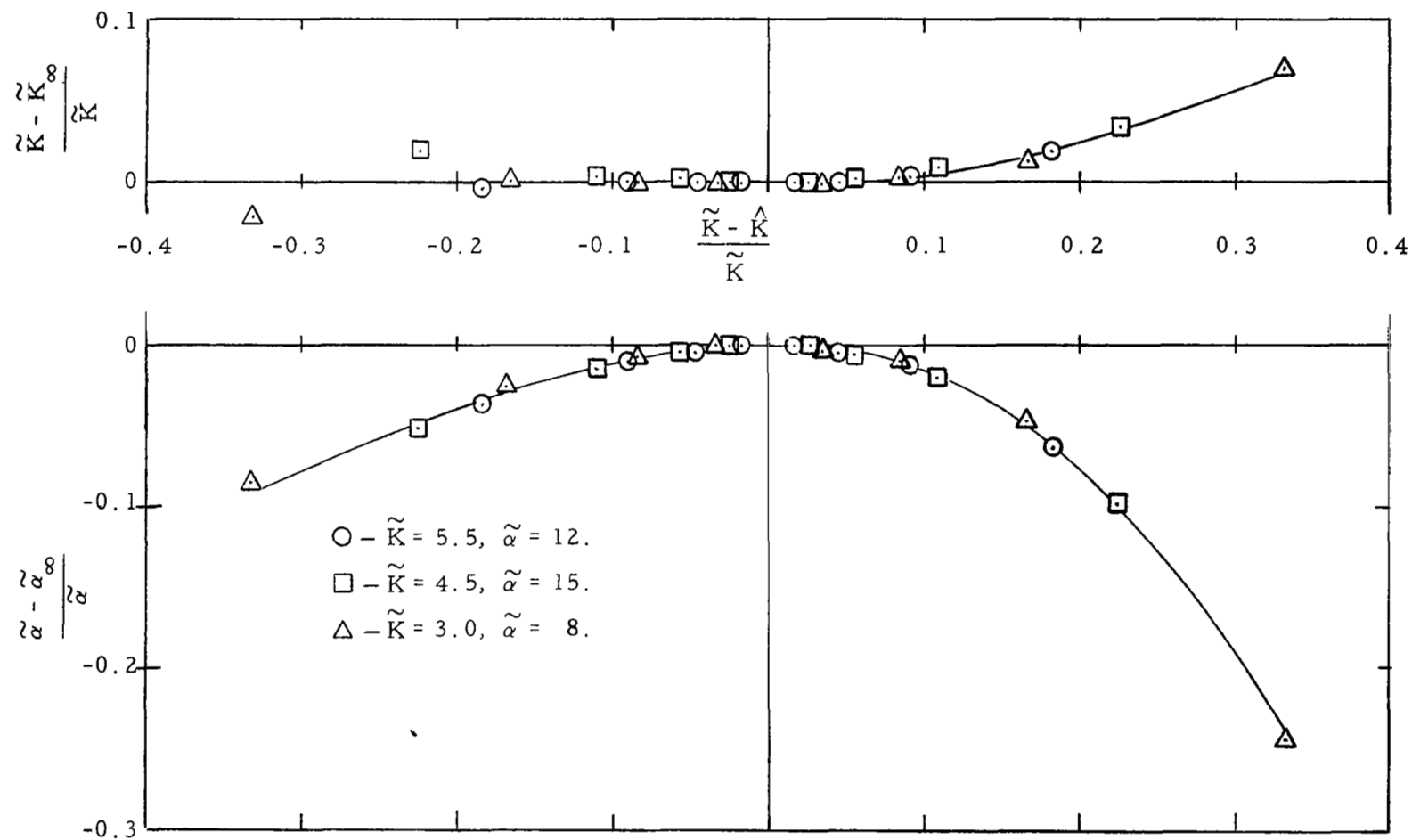
Figure 4.1-3 Results of Infinite Data Interval Analysis, \hat{\alpha} = \tilde{\alpha}
