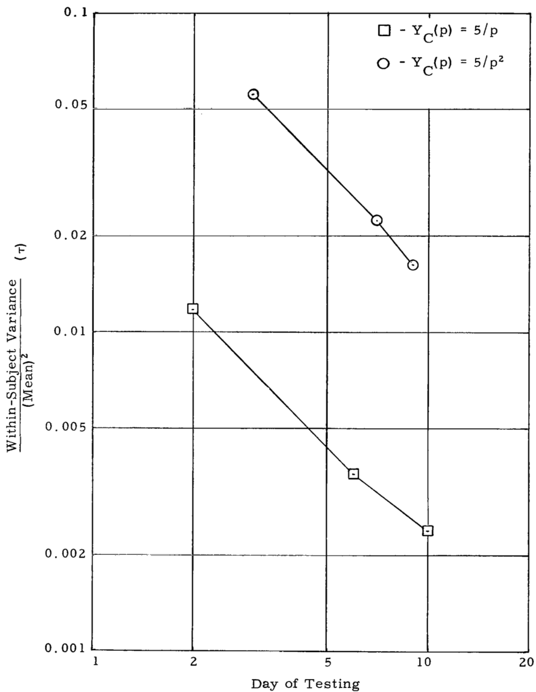
Figure 5.3-6 Within-Subject Variance of \tau
