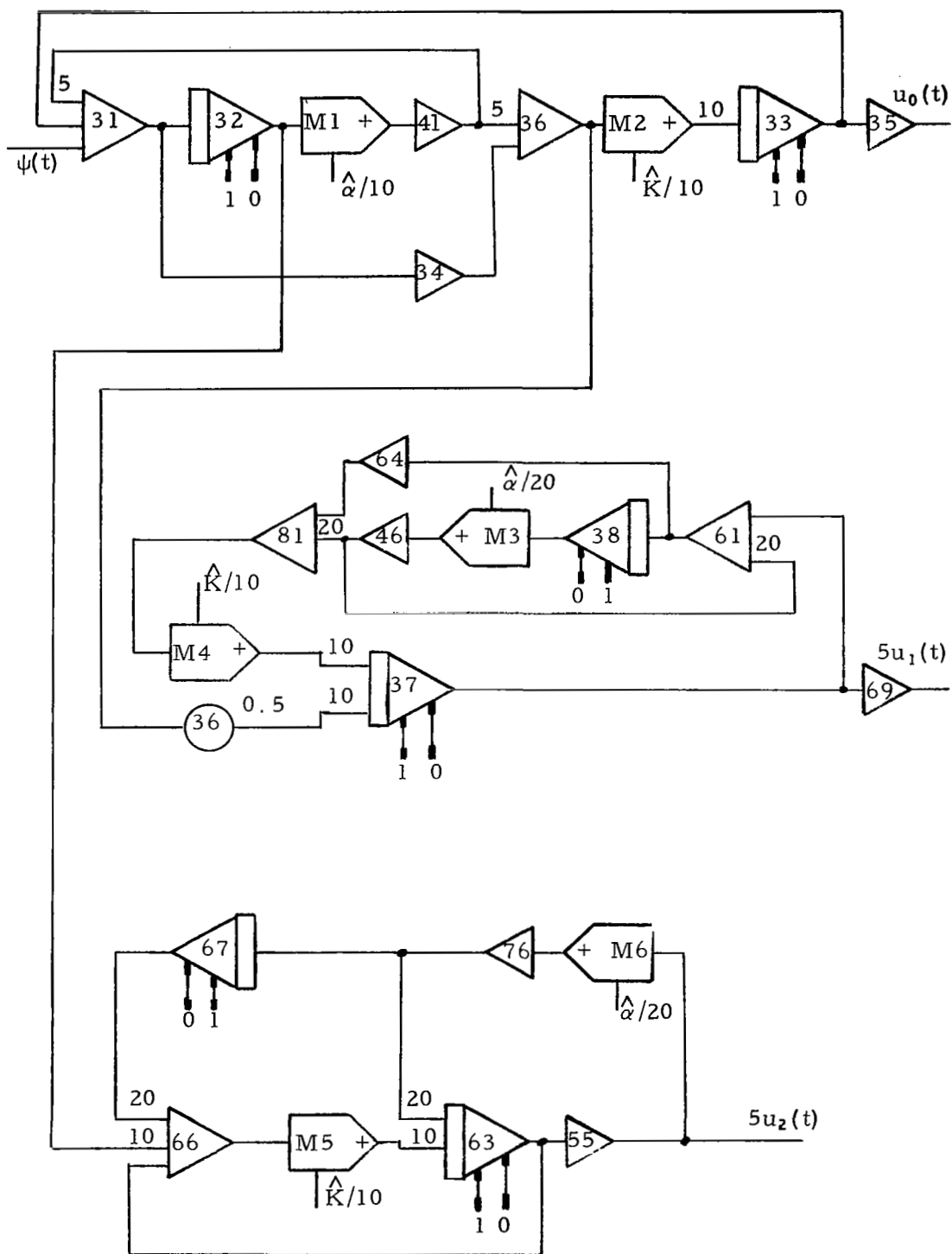
Figure A-2 Circuit Diagram for Crossover Model Implementation
