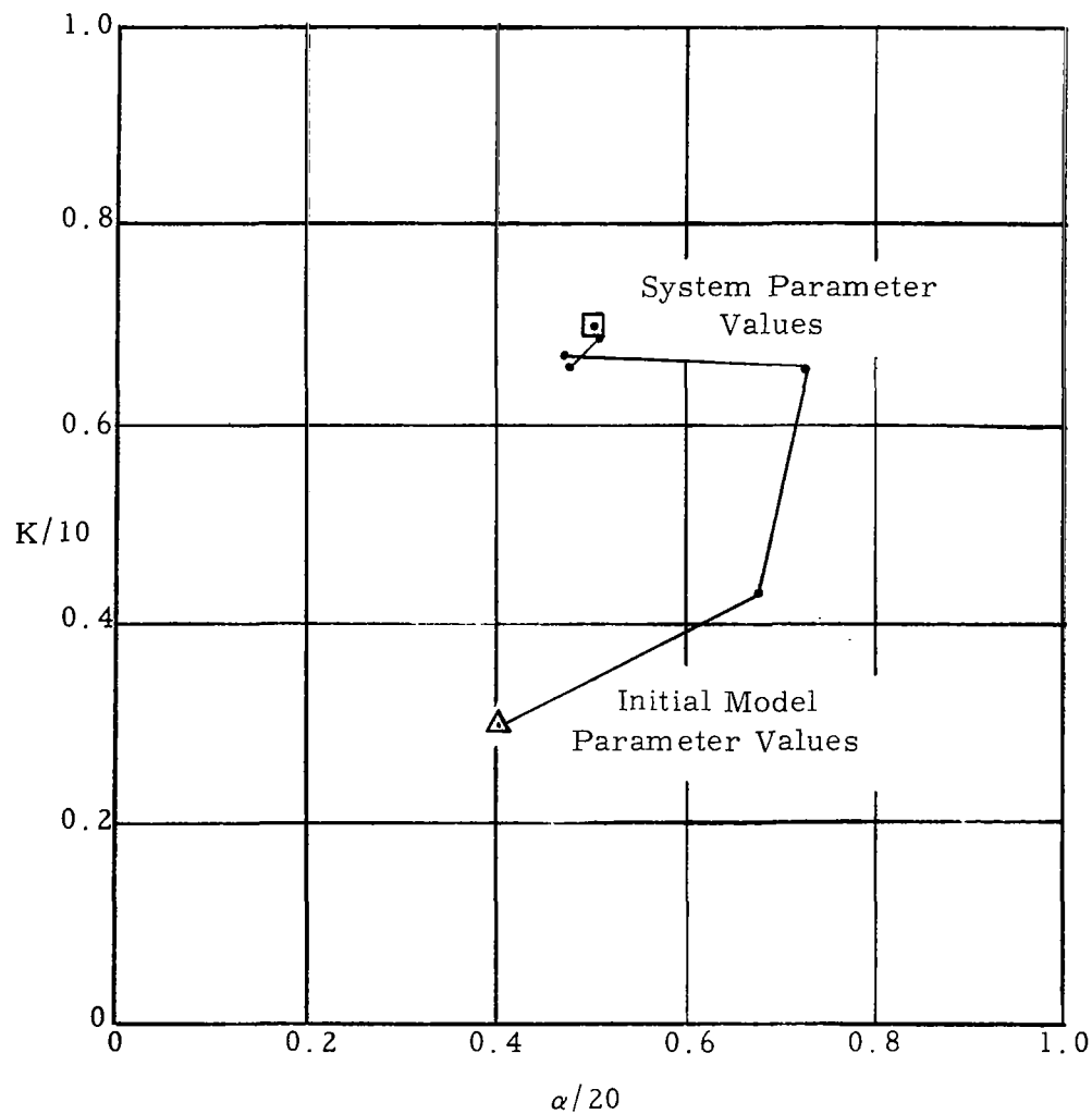
Figure 4.2-1 Convergence of Regression Analysis Technique
