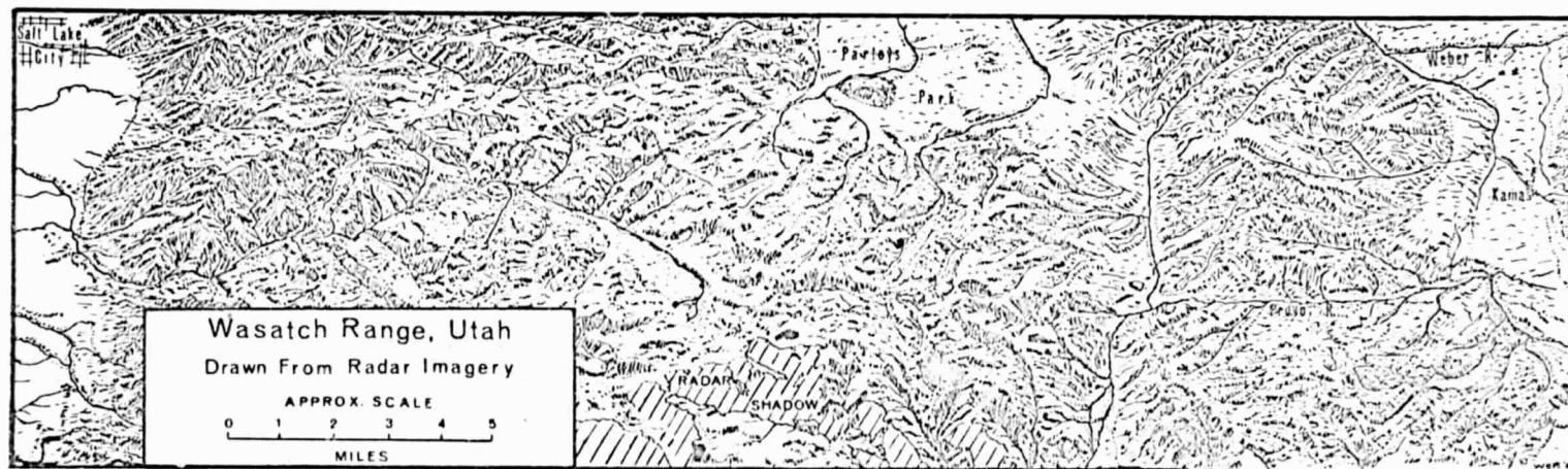
Figure 11. Physiographic Map of the Wasatch Range, Utah.
