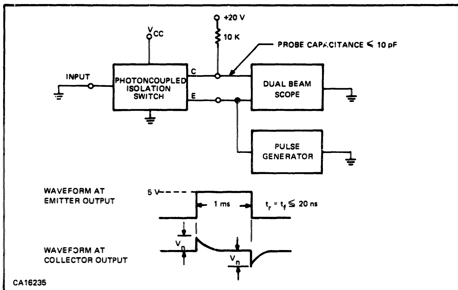
Figure 3. Noise Transmissibility Test
