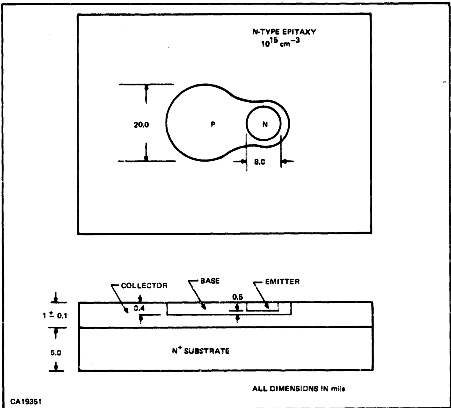
Figure 12. Basic Phototransistor-Diffusion Outline
