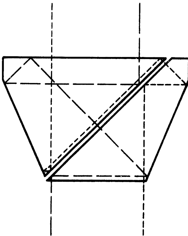
c. Pechan Prism
