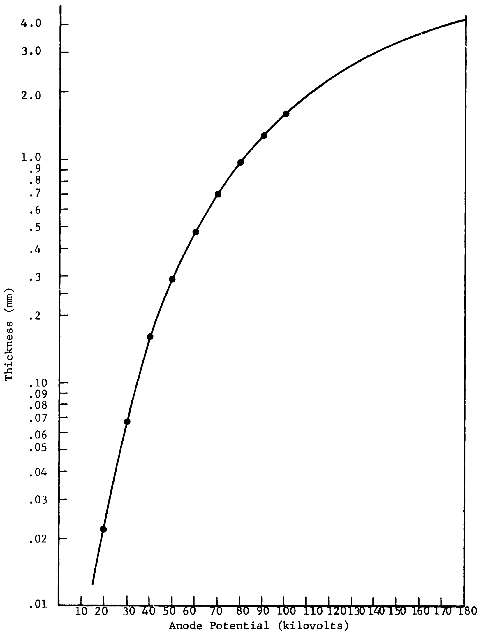
Figure III-B-1 THE 1/e X-RAY TRANSMISSION THICKNESS OF COPPER AS A FUNCTION OF ANODE VOLTAGE
