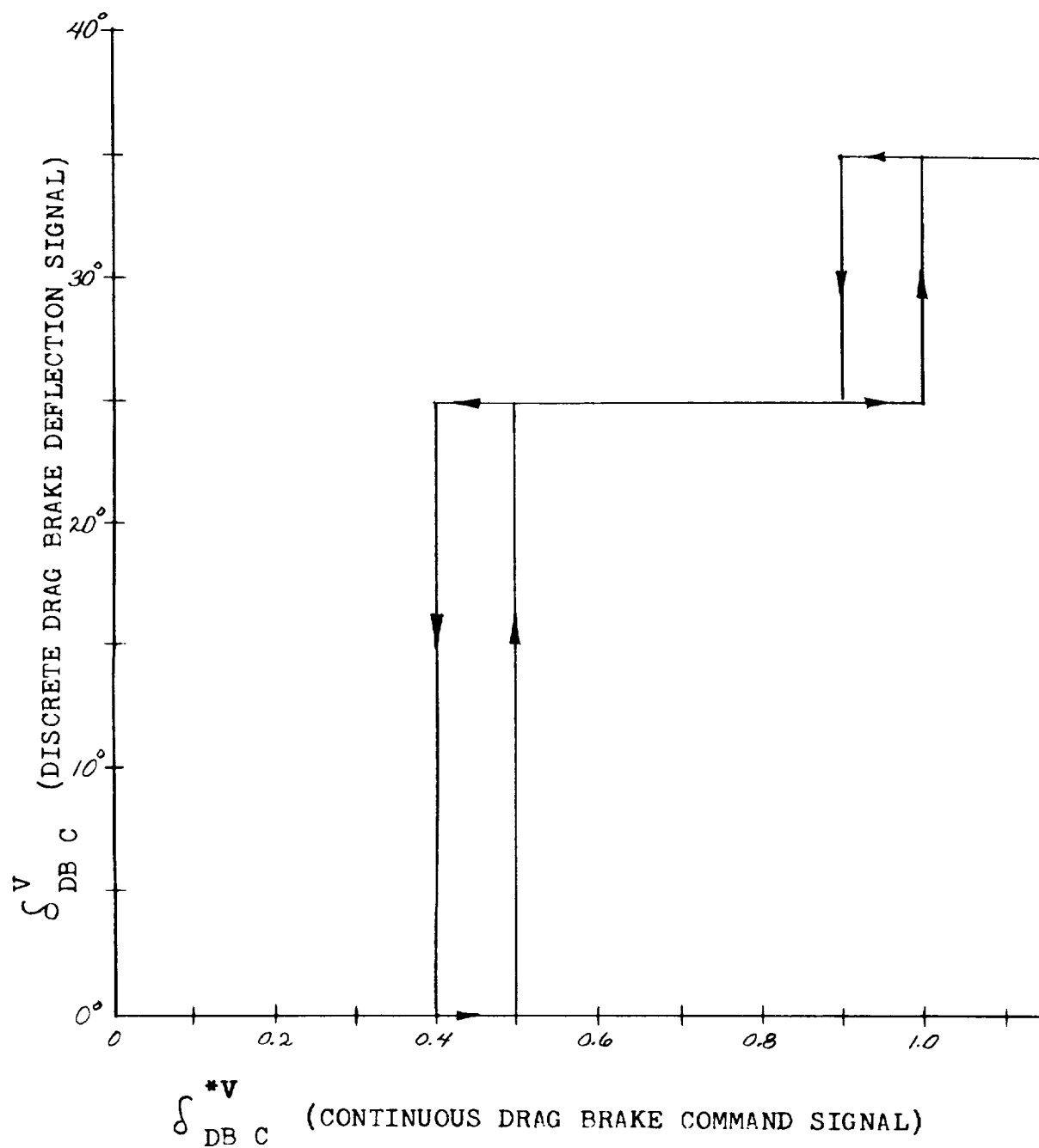
Figure 7.— Generation of discrete drag brake deflection signal.
