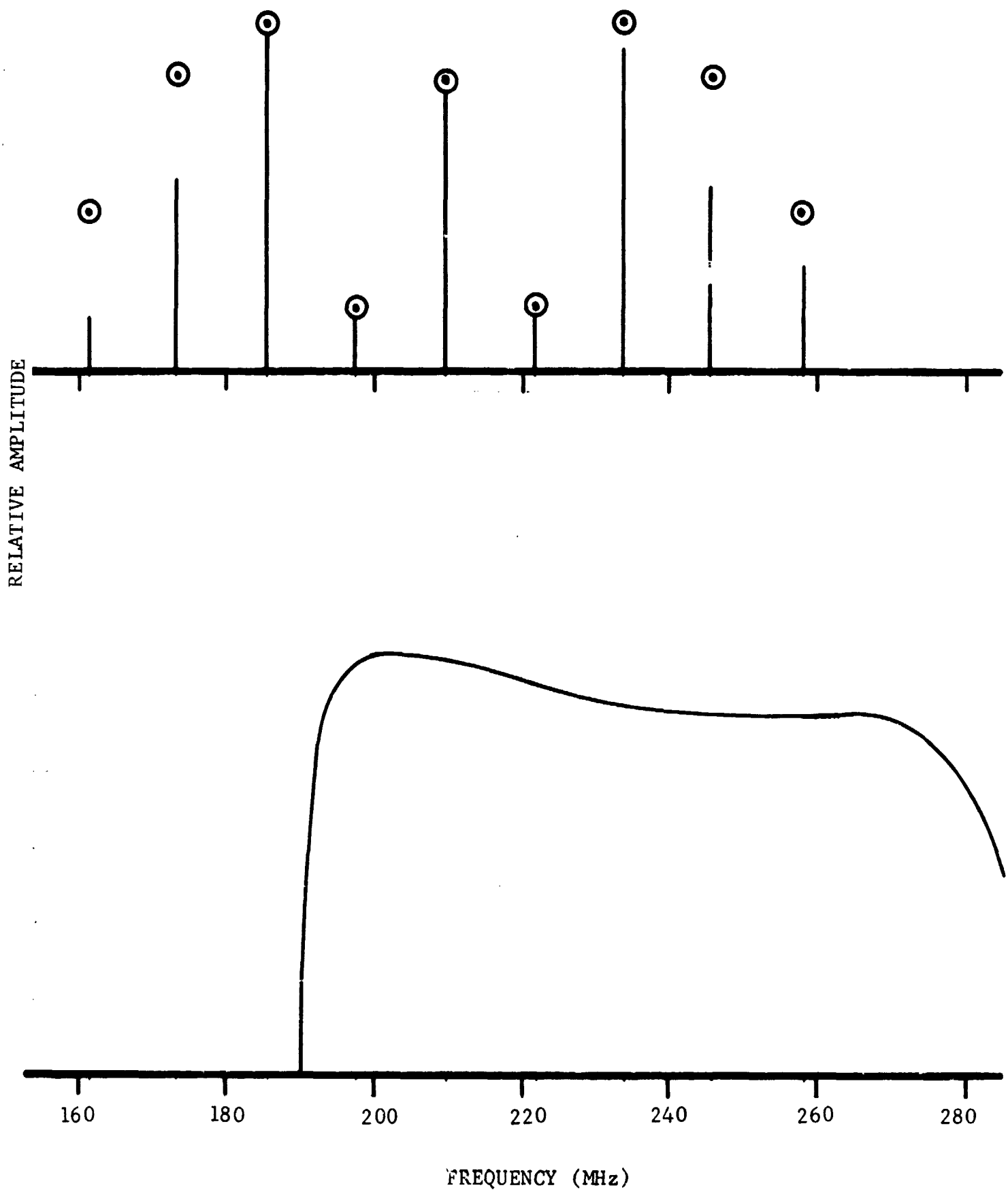
FIGURE 26. (a) SIDEBAND SPECTRA OVERLAPPING THE SUBCARRIER SWITCHING POINTS, \nu_{\text{mod}} = 12 \text{ MHz} , Bandwidth = 110 MHz. (b) CORRESPONDING DC RESPONSE.
