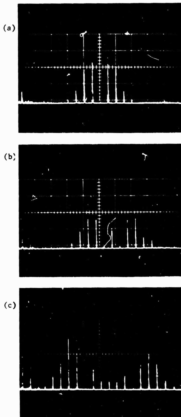
FIGURE 18. DPFM SIDEBAND SPECTRA AT 3.39\mu WITH A MODULATION FREQUENCY OF 3 MHz AND DRIVING VOLTAGES OF (a) 110\text{ V}_{\text{rms}} , (b) 170\text{ V}_{\text{rms}} , AND (c) 290\text{ V}_{\text{rms}}
