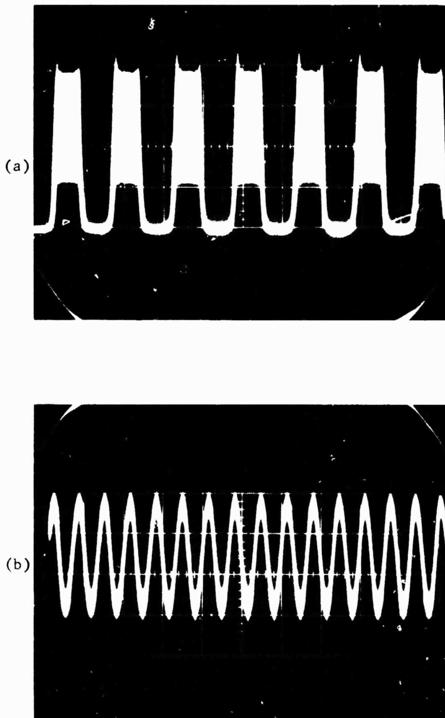
FIGURE 43. CO 2 LASER OUTPUT, AMPLITUDE MODULATED AT 1.53 MHz. MODULATOR DRIVE VOLTAGE = 14 V rms .
