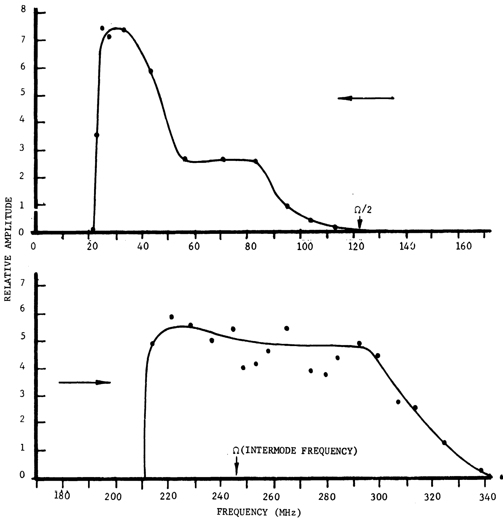
FIGURE 16. 1.15 μ SUBCARRIER AMPLITUDE
