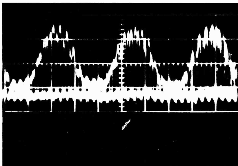
FIGURE 42. CO 2 LASER OUTPUT, AMPLITUDE MODULATED AT 60 Hz. MODULATOR DRIVE VOLTAGE = 120 V rms . DEPTH OF MODULATION \approx 85%. NOTICEABLE HARMONIC DISTORTION IS EVIDENT.
