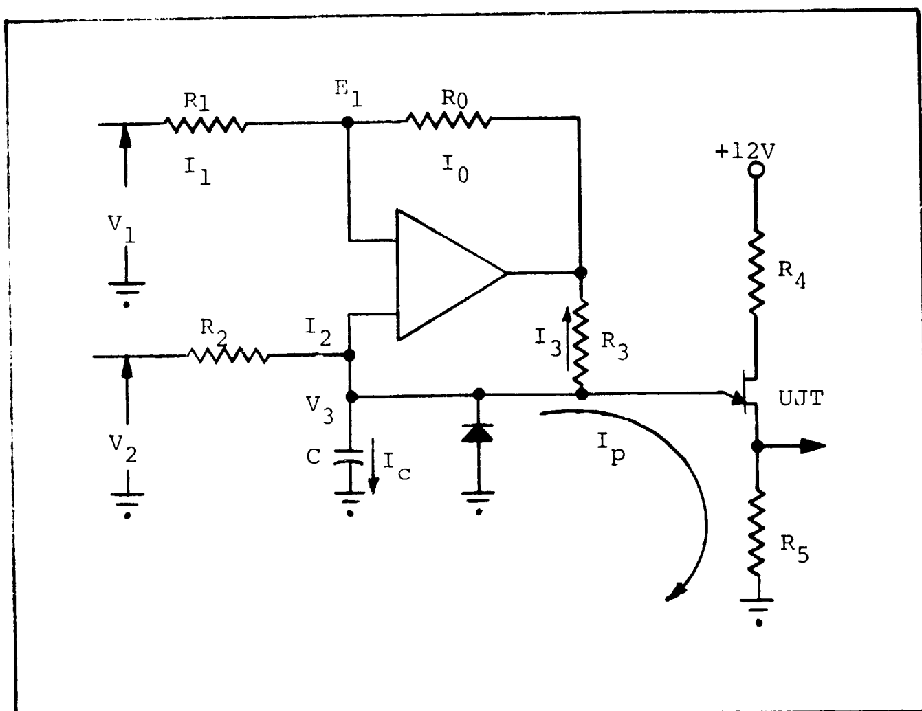
Figure 15. - Voltage-to-Frequency Pulse Generator
