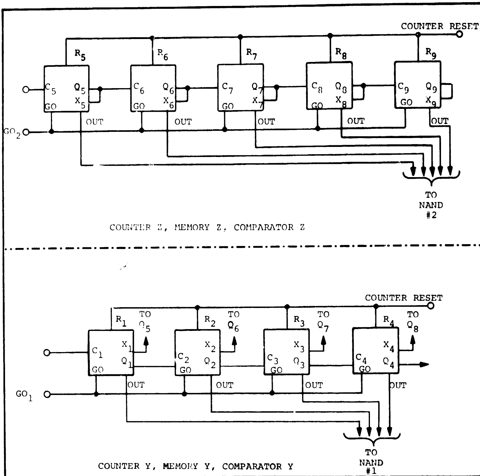
Figure 21. - Interstage Connections for Counters, Etc.
