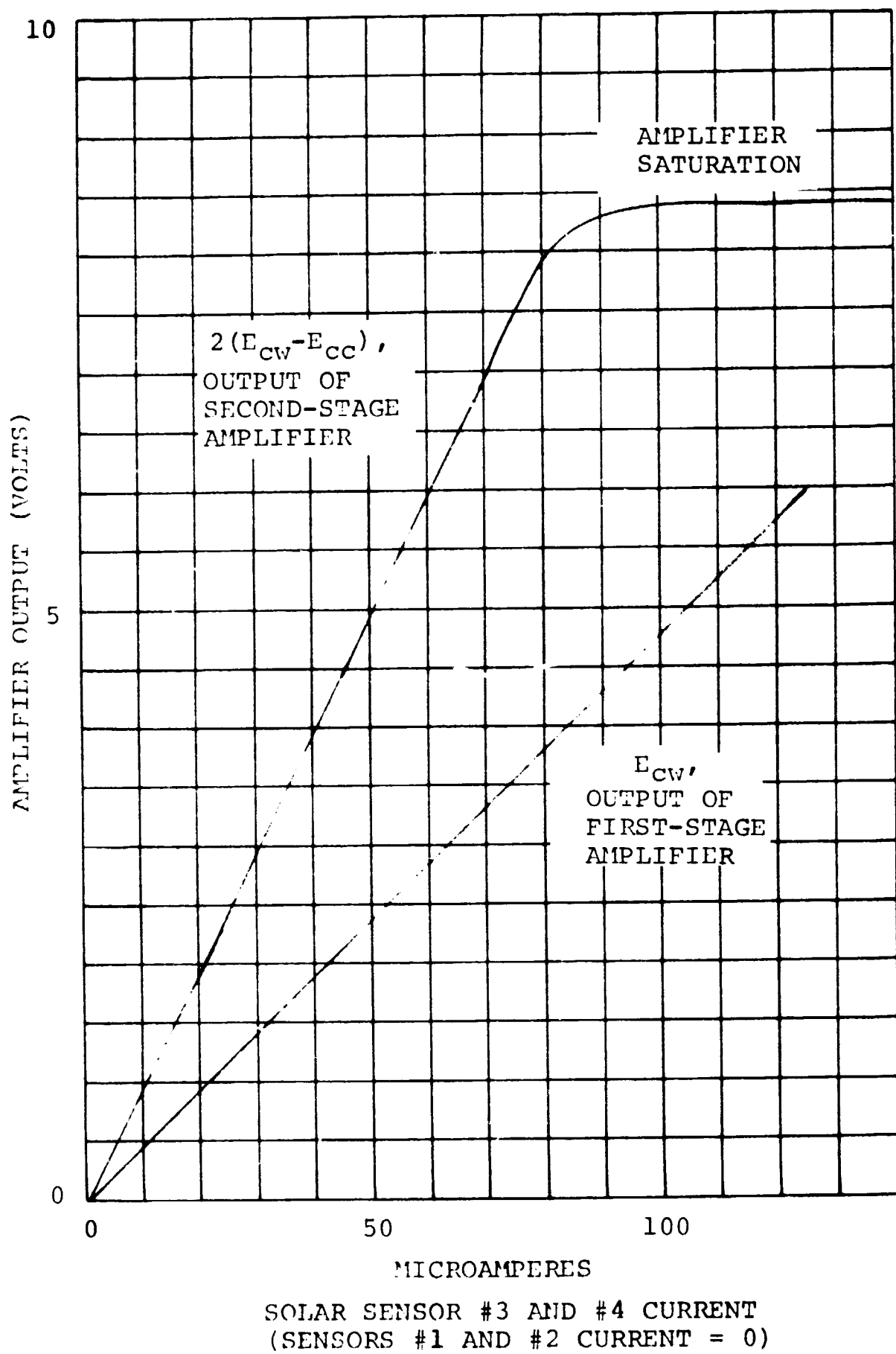
Figure 31. - Solar Sensor Amplifier Output Characteristics
