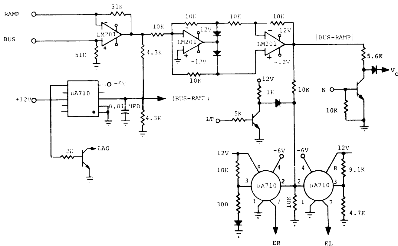
Figure 14. - Speed Control Amplifier Circuit
