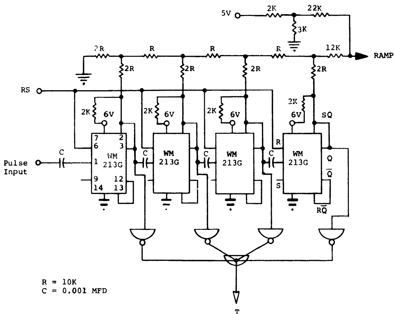
Figure 13. - Speed Reference Ramp Generator
