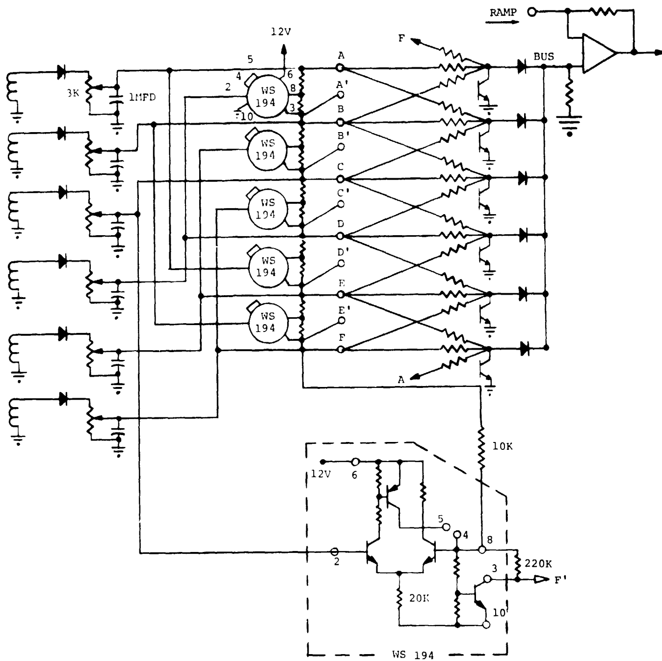
Figure 12. - Magnetic Sensor Signal Processing Circuit
