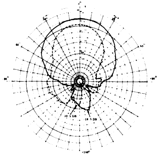
Figure 3.3-4. Feed Pattern in \phi = 90^\circ Plane Using 4-Turn Helix Feed; Axial Ratio = 2.5 DB for \psi = 0^\circ Direction, f = 7.5 GHz
