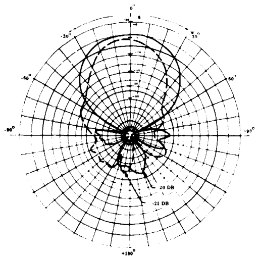
Figure 3.3-8. Feed Pattern in \phi = 90^\circ Plane Using 6-Turn Helix Feed; Axial Ratio = 1.9 DB for \psi = 0^\circ Direction, f = 7.5 GHz
