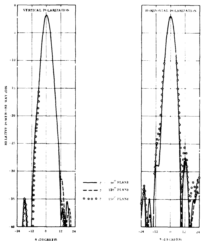
Figure D-4. Pattern Response of a Paraboloid in \phi = 90^\circ , 120^\circ , and 150^\circ Planes Using a 5-Turn Helix Feed
