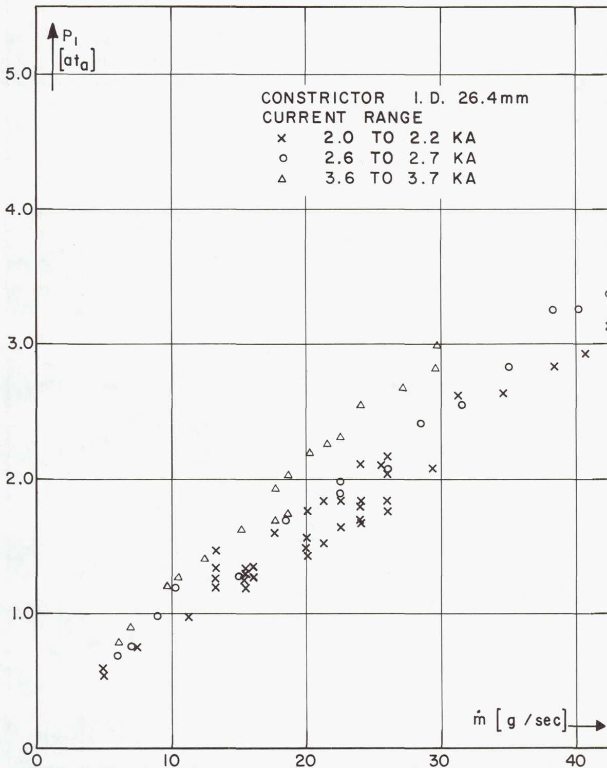
Fig. 15. Inlet pressure P_1 of constricted arc heater as function of nitrogen flow rate.
