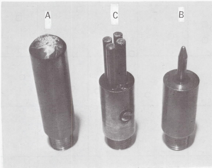
Fig. 23. Different cathodes tested with the pulsed arc.
