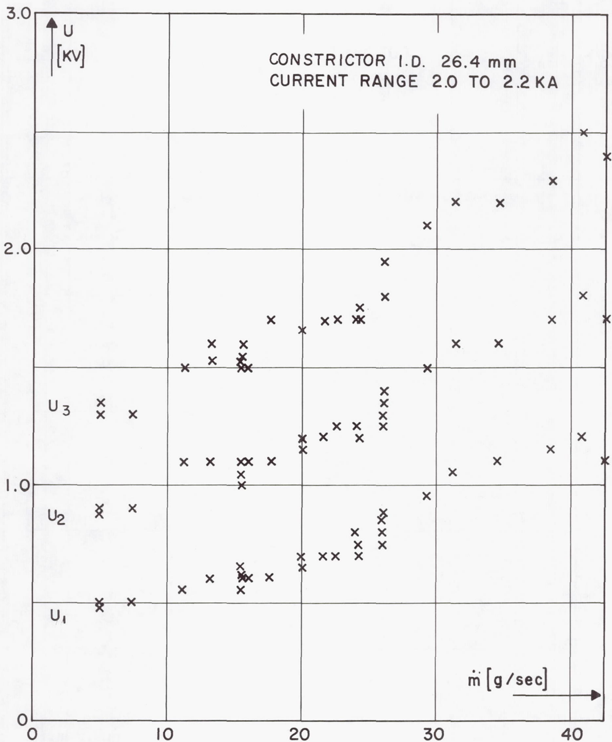
Fig. 16. Arc voltage U as function of nitrogen flow rate \dot{m} .
