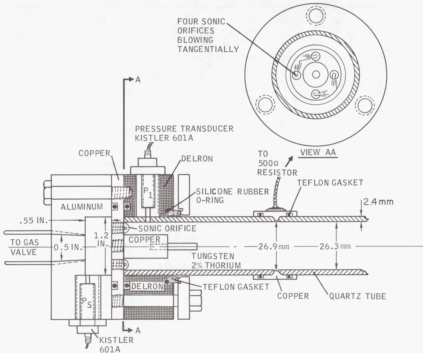
Fig. 4. Cathode assembly with sonic orifices and pressure transducers.
