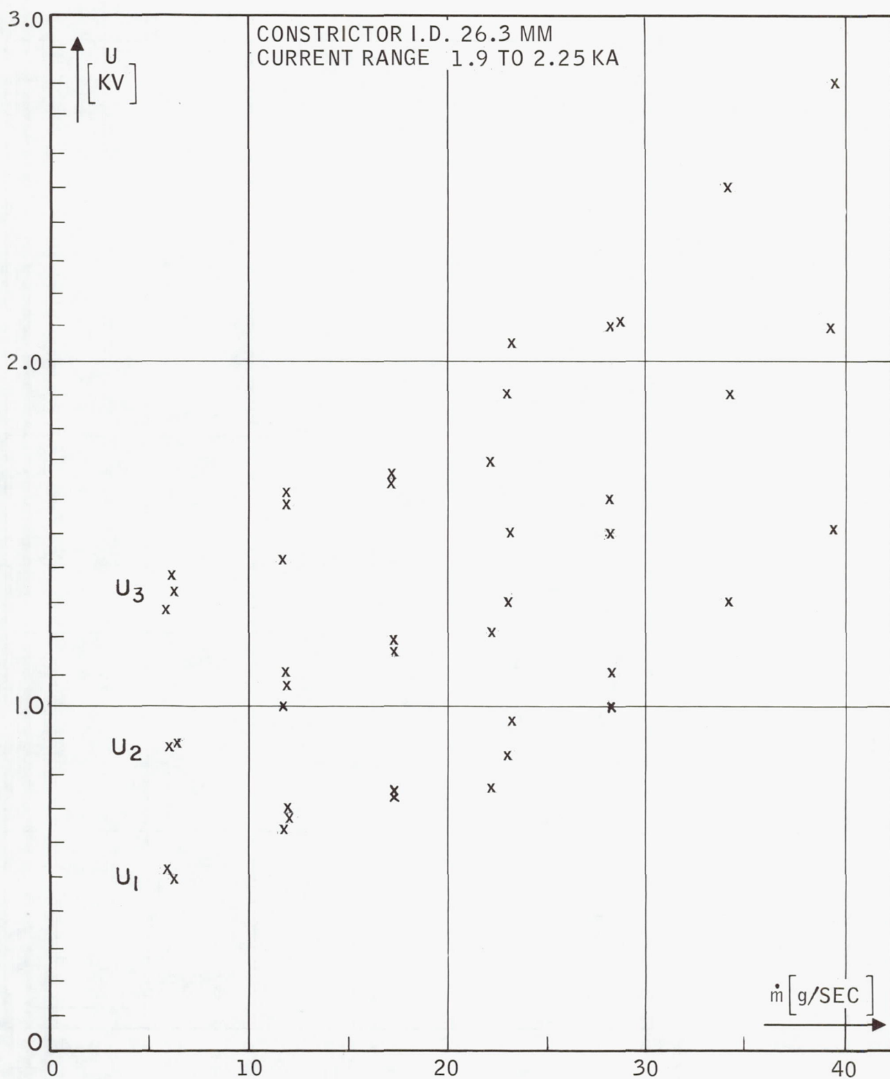
Fig. 13. Arc voltage U as function of nitrogen flow rate \dot{m} .
