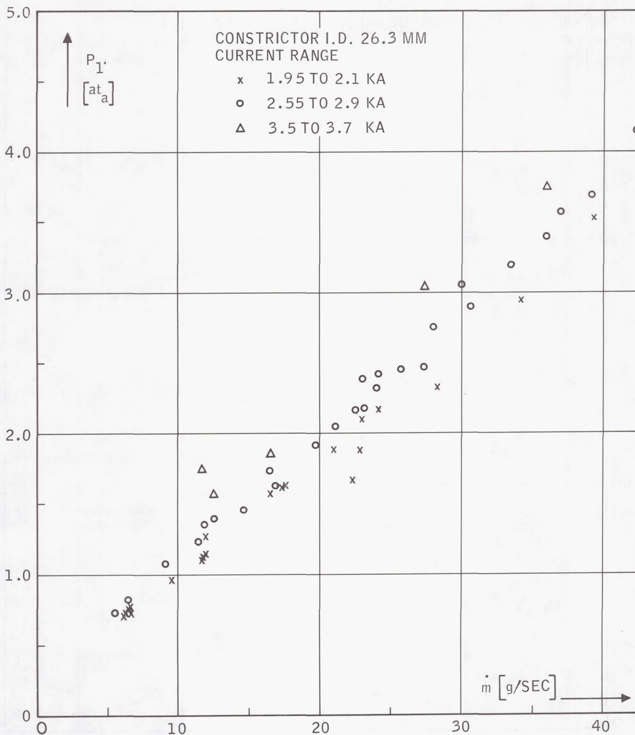
Fig. 12. Inlet pressure P_1 of constricted arc heater as function of nitrogen flow rate \dot{m} .
