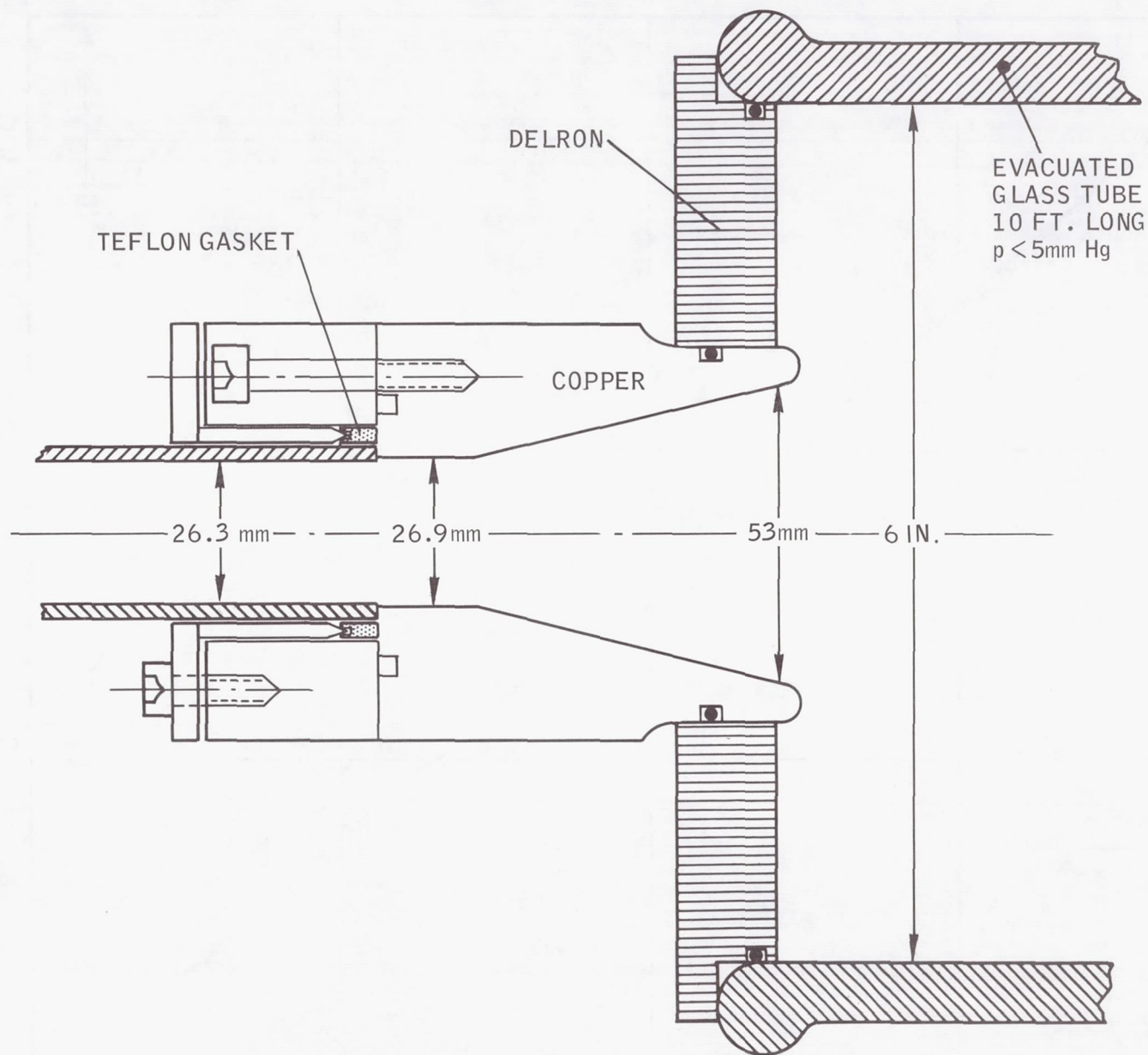
Fig. 6. Anode design for pulsed constricted arc.
