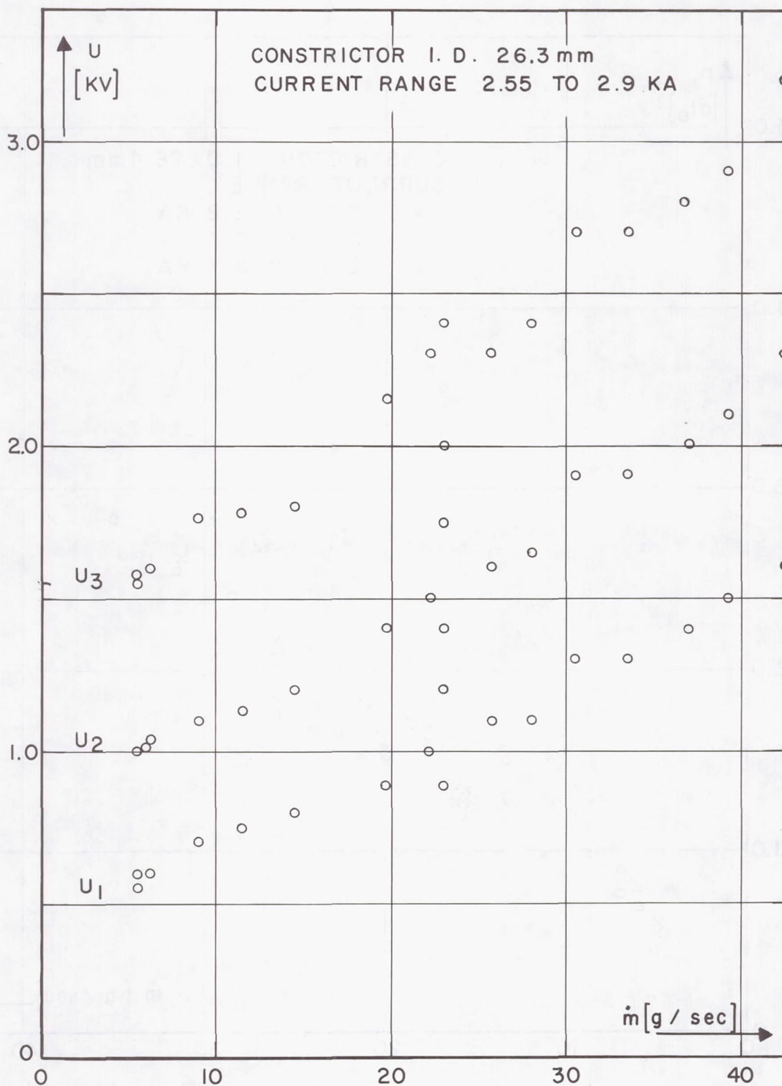
Fig. 14. Arc voltage U as function of nitrogen flow rate \dot{m} .
