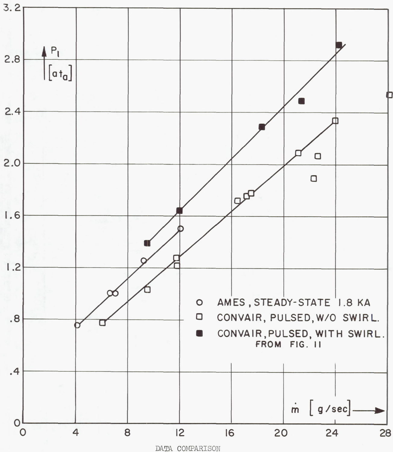
Fig. 21 Inlet pressure P_1 as function of nitrogen flow rate \dot{m} .
