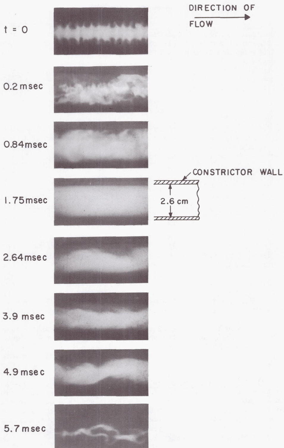
Fig. 27. High speed film displaying the time history of the pulsed arc with axial flow. 11 g/sec nitrogen flow, 2 KA. Position about 20 cm downstream of cathode.
