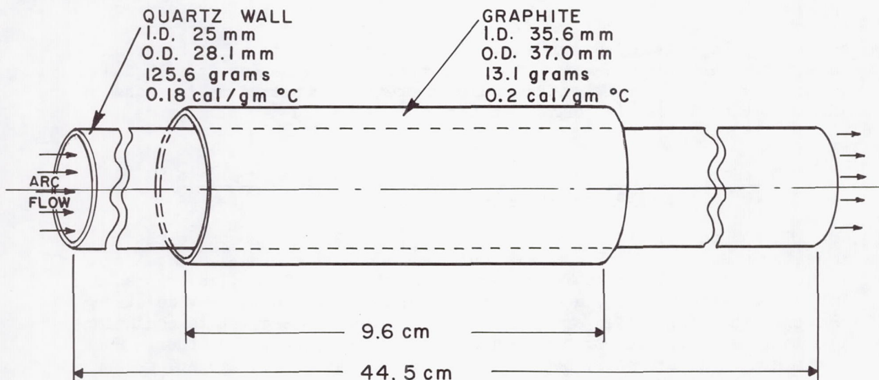
Fig. 18. Calorimeter geometry for measuring wall heat flux.
