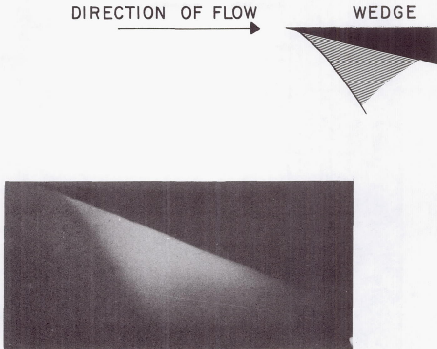
Fig. 30. A wedge exposed to the exhaust stream of the pulsed arc heater. Position of leading edge about 4 cm from exit plane of anode. 30.7 g/sec nitrogen flow, 3.5 KA current, exposure time about 1 \mu sec.
