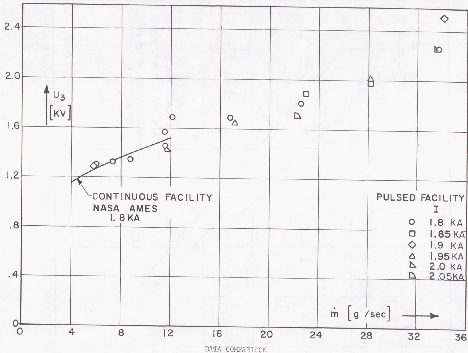
Fig. 20. Voltage between cathode and 54" station U_3 as function of nitrogen flow rate \dot{m} .
