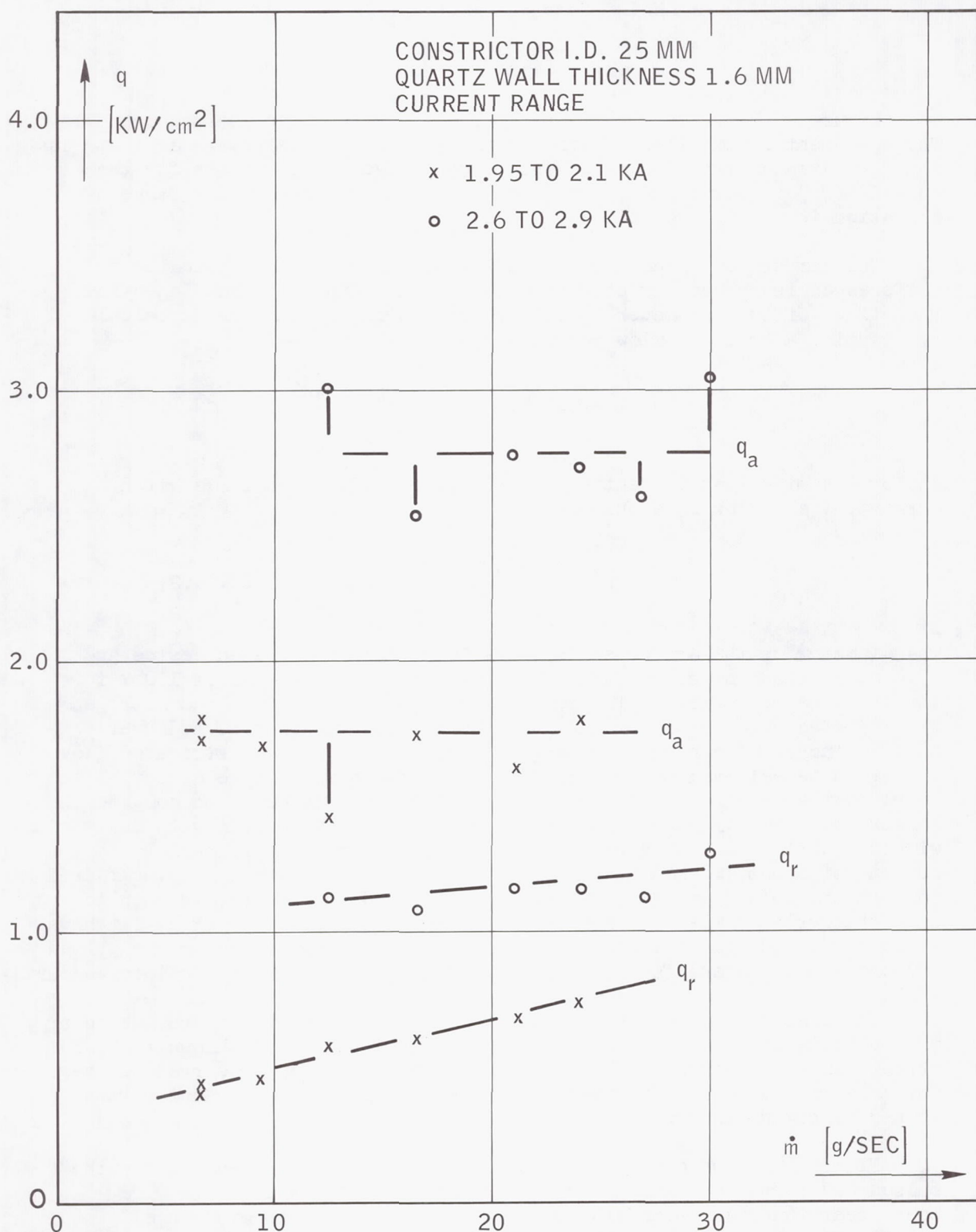
Fig. 19. Heat flux absorbed in quartz constrictor wall q_a and heat flux transmitted through quartz wall q_r as function of nitrogen flow rate \dot{m} .
