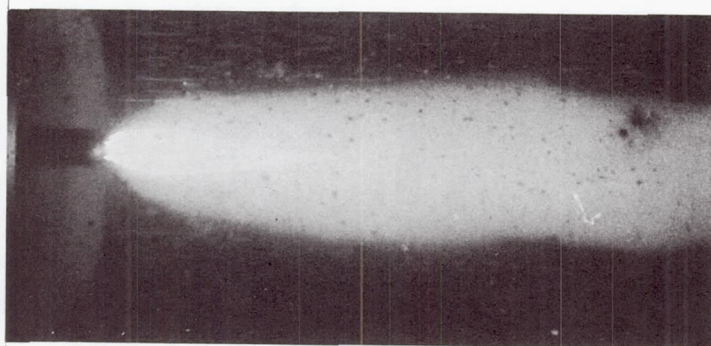
Fig. 26. Arc attachment on the cathode of Fig. 23B with pointed end face. 16 g/sec nitrogen flow, 2 KA, lower photo is retouched in order to show the cathode jet more clearly.
