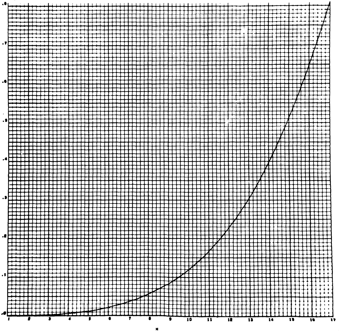
Figure 5 - Interpolative Approximation, L = 17 , N = 4 , k = 4
