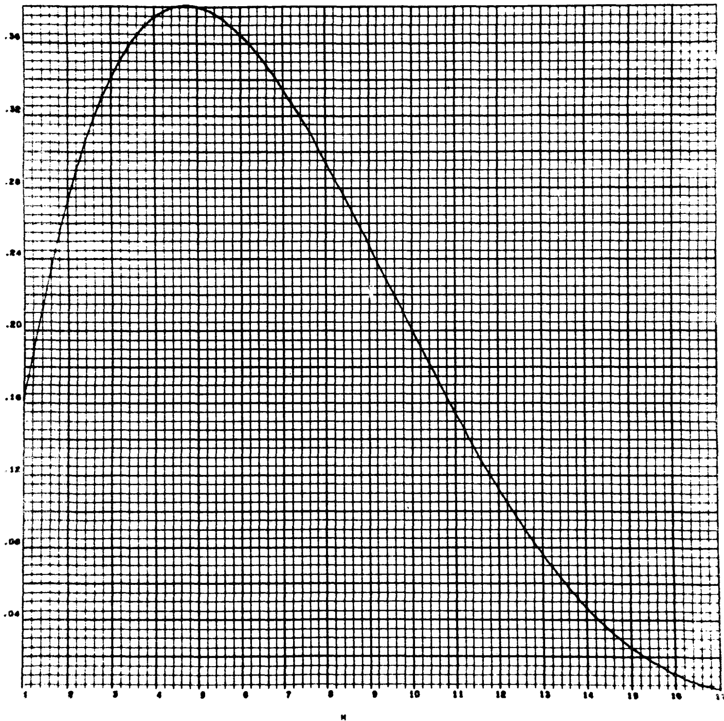
Figure 2 - Interpolative Approximation, L = 17 , N = 4 , k = 2
