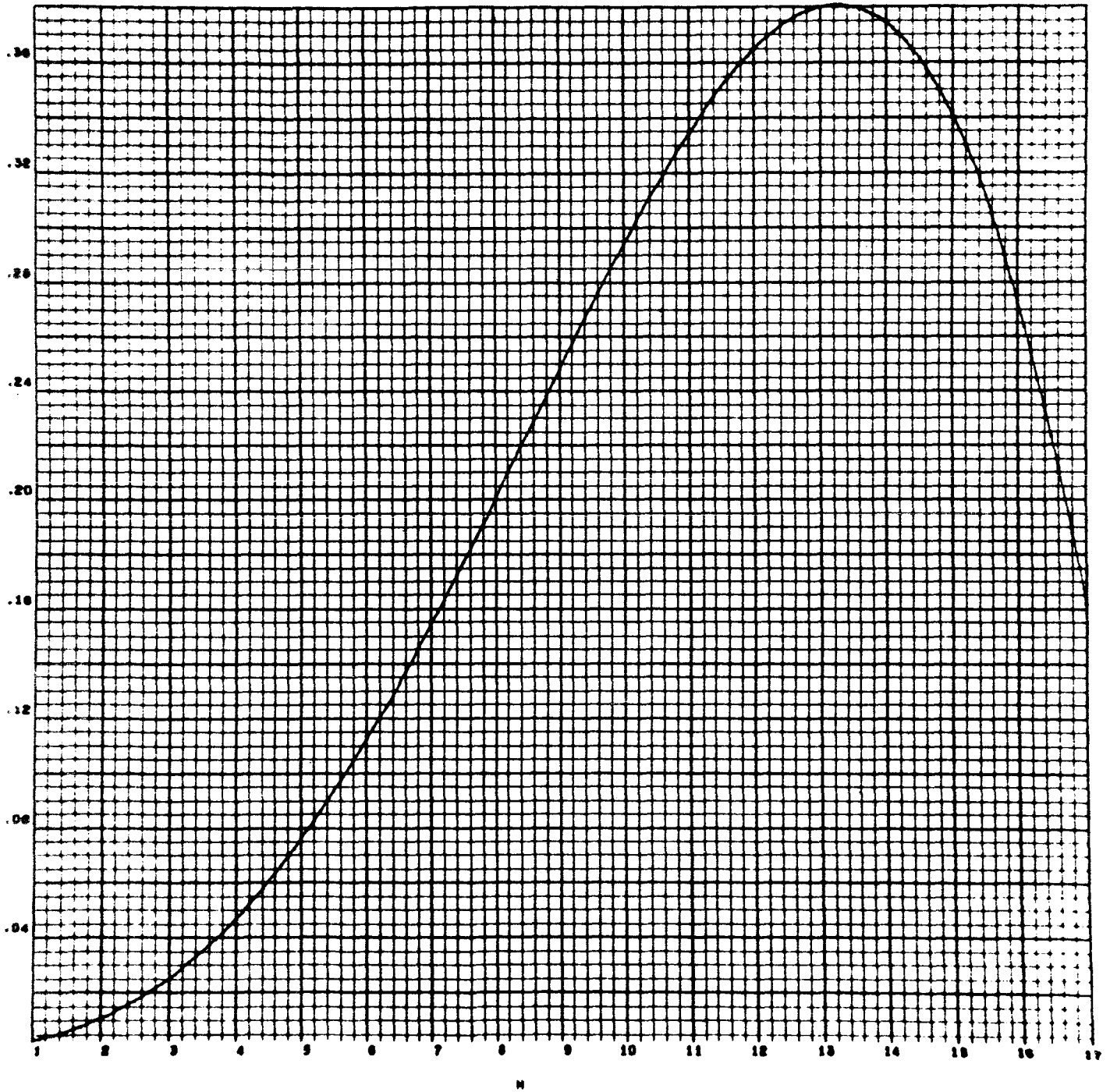
Figure 4 - Interpolative Approximation, L = 17 , N = 4 , k = 3
