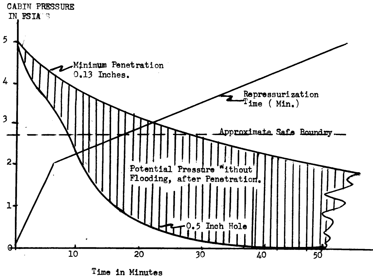
Figure 2-14. Cabin Depressurization/Pressurization Rates, Apollo CSM
