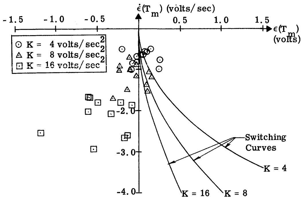
Figure 5.2.1 Average Terminal States in the Phase Plane for Exploratory Prediction.
