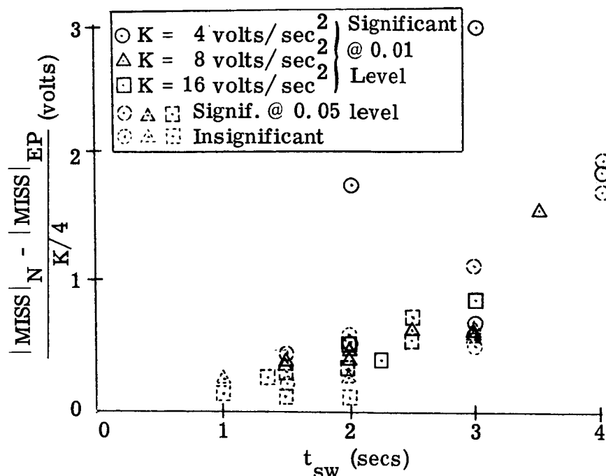
Figure 5.5.1 Difference in Gain-Normalized Absolute MISS Between Normal Display (N) and Exploratory Prediction (EP) vs. Switch Time.
