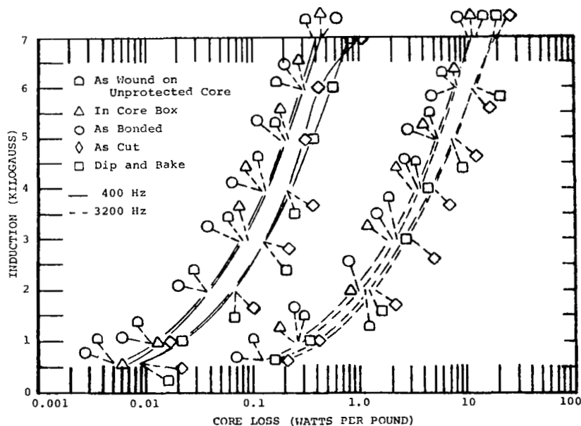
Figure 97. - Degradation Test, P_c , sq, Total Core Loss, 0.004-Inch 4%Mo-79%Ni-17%Fe Toroid, Square Loop, Core 39, Room Ambient. Processing Variables: In Core Box, As Bonded, As Cut, and Dip and Bake
