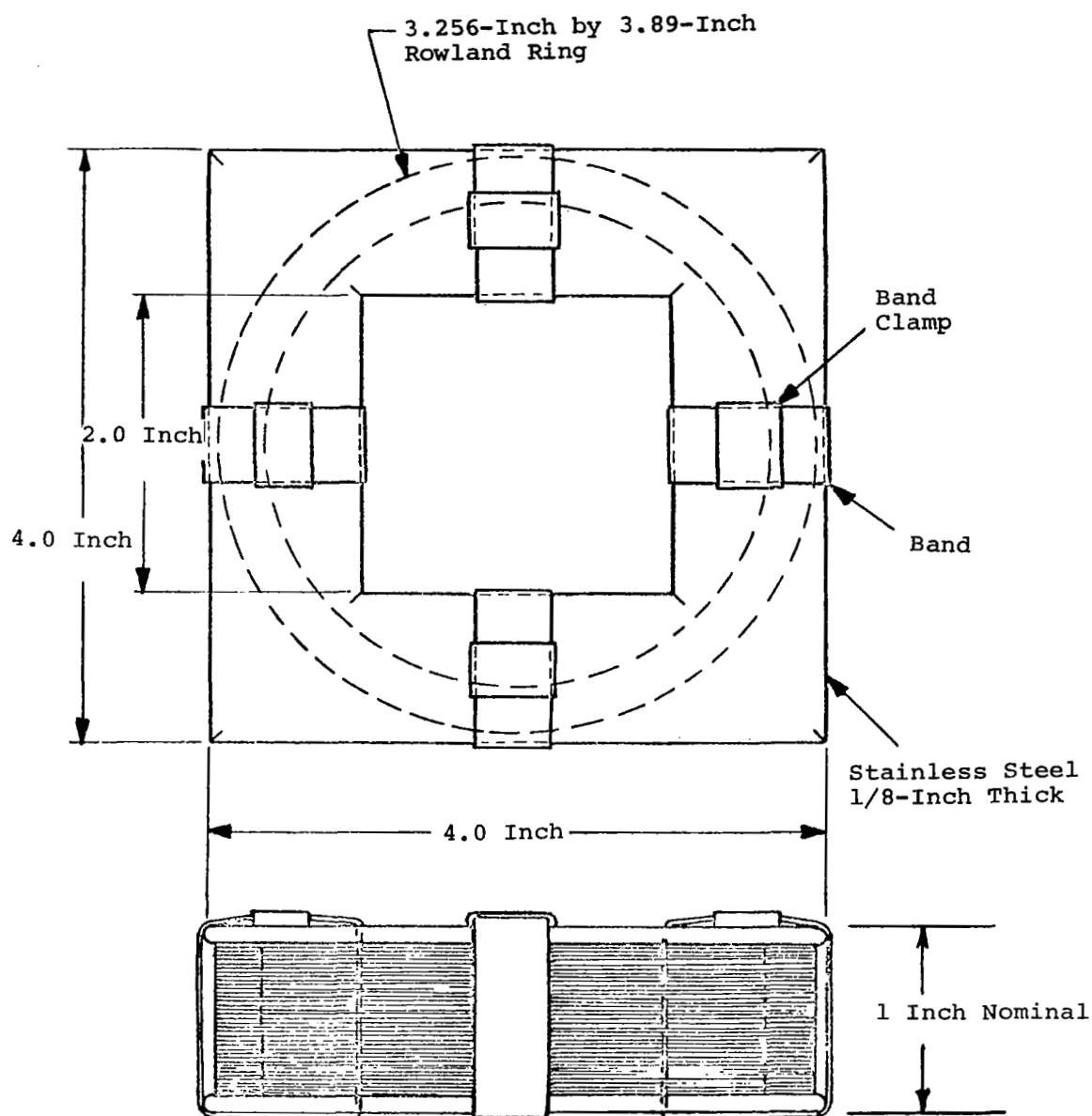
Figure 5. - Clamping Arrangement for Rowland Rings Vacuum Testing
