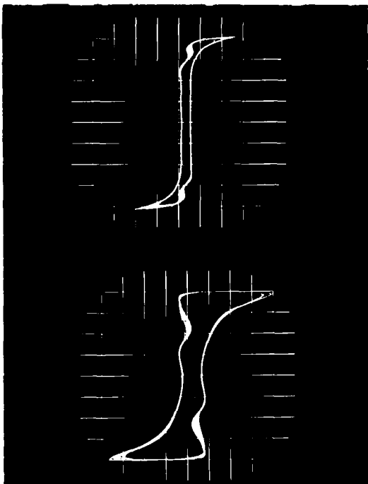
Figure 42. - AC Hysteresis Loop, Square Wave Excitation, 400, 800, 1600, and 3200 Hz, 0.004-Inch 49%Co-2%V-49%Fe Rowland Ring, Magnetic Field Annealed, 250° C
