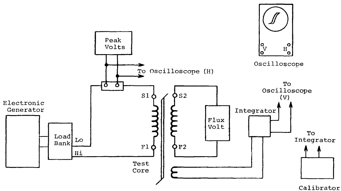
Figure 113. - Major AC Hysteresis Loop Test Circuit
