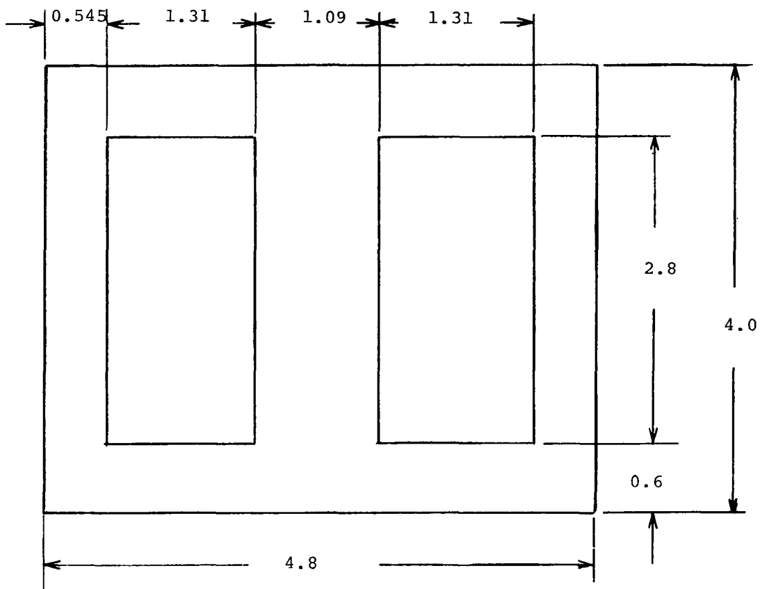
Figure 2. - Double Window Lamination
