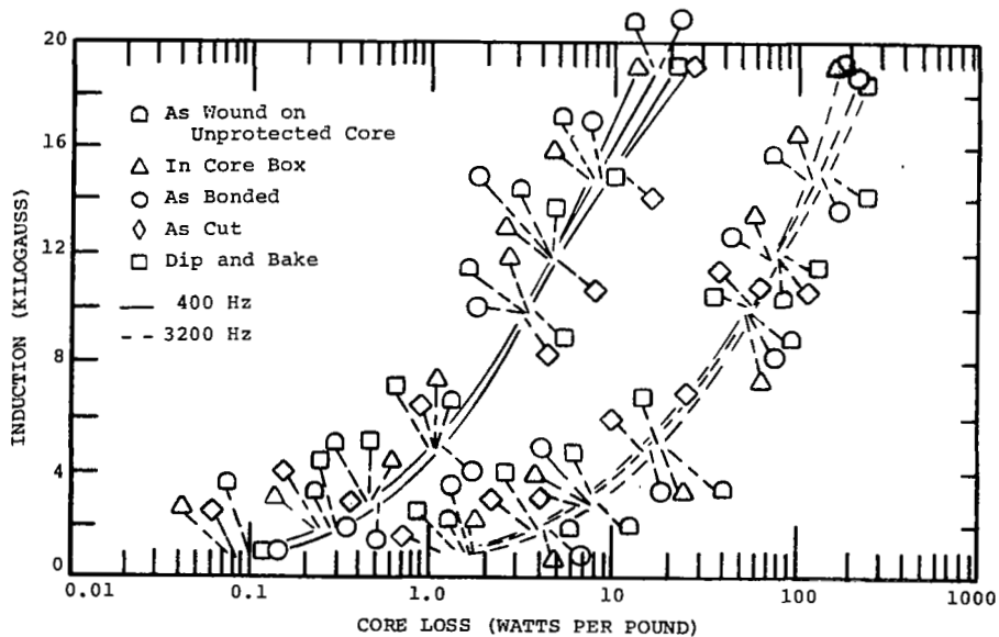
Figure 95. - Degradation Test, P_c , P_{sq} , Total Core Loss, 0.006-Inch Singly Grain Oriented Silicon Steel, Square Toroid, Core 40, Room Ambient. Processing Variables: In Core Box, As Wound, As Bonded, As Cut and Dip and Bake
