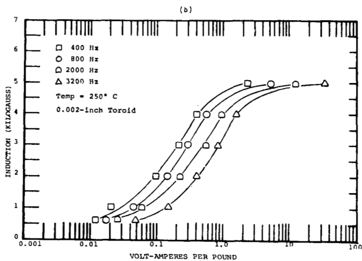
Figure 11. - P_{a, sq} , Apparent Power vs Induction and Frequency, 0.002-Inch 4%Mo-79%Ni-17%Fe Toroid, Square Loop
