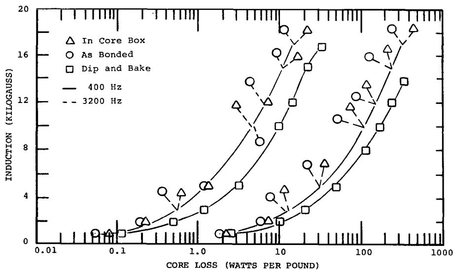
Figure 93. - Degradation Test, P_{c, sq} , Total Core Loss, 0.006-Inch Doubly Grain Oriented Silicon Steel, Double Window, Magnetic Field Annealed, Core 1, Room Ambient. Processing Variables: In Core Box, As Bonded, and Dip and Bake
