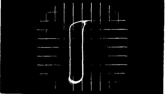
Figure 16.- AC Hysteresis Loop, Square Wave Excitation, 400, 800, 1600, and 3200 Hz, 0.002-Inch 4%Mo-79%Ni-17%Fe Toroid, Square Loop, Room Ambient
