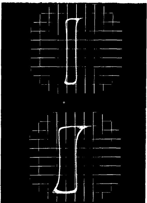
Figure 30. - AC Hysteresis Loop, Square Wave Excitation, 400, 800, 1600, and 3200 Hz, 0.002-Inch 50%Ni-50%Fe Toroid, Grain Oriented, Room Ambient
