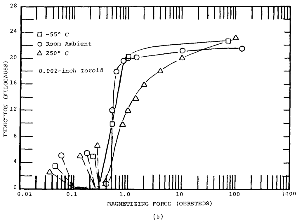
Figure 34. - DC Magnetization, 0.004- and 0.002-Inch 49%Co-2%V-49%Fe Toroid, Magnetic Field Annealed
