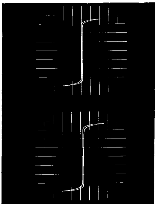
Figure 58. - AC Hysteresis Loop, Square Wave Excitation, 400, 800, 1600, and 3200 Hz, 0.002-Inch Singly Grain Oriented Silicon Steel, Room Ambient
