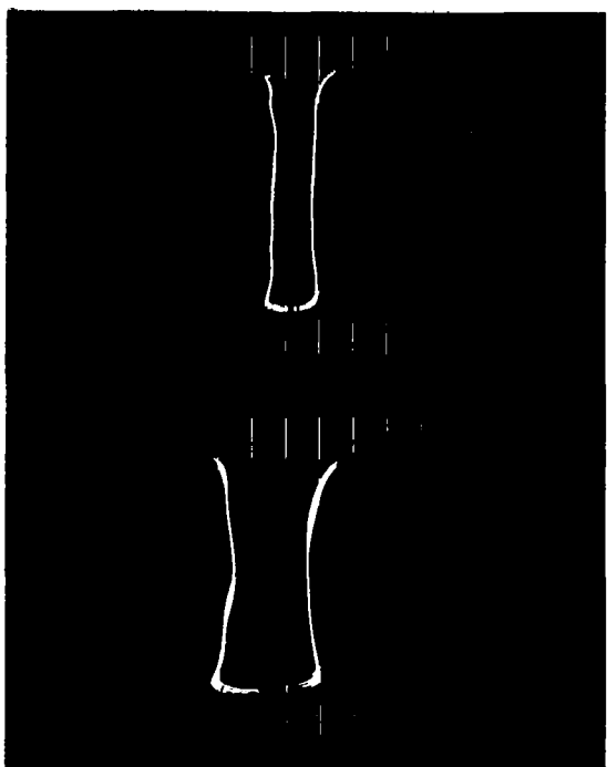
Figure 43. - AC Hysteresis Loop, Square Wave Excitation, 400, 800, 1600, and 3200 Hz, 0.002-Inch 49%Co-2%V-49%Fe Toroid, Magnetic Field Annealed, -55^{\circ} \text{ C}
