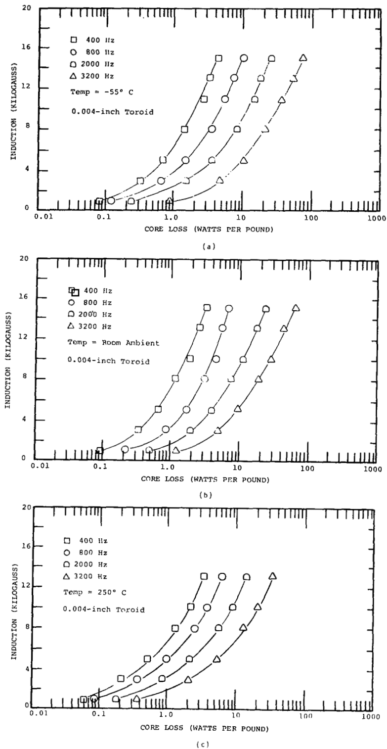
Figure 22. - P_{c, sq} , Total Core Loss vs Induction and Frequency, 0.004-Inch 50%Ni-50%Fe Toroid Grain Oriented
