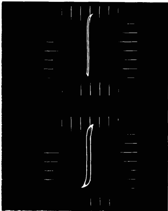
Figure 15.— AC Hysteresis Loop, Square Wave Excitation, 400, 800, 1600, and 3200 Hz, 0.002-Inch 4%Mo-79%Ni-17%Fe Toroid, Square Loop, -55° C
