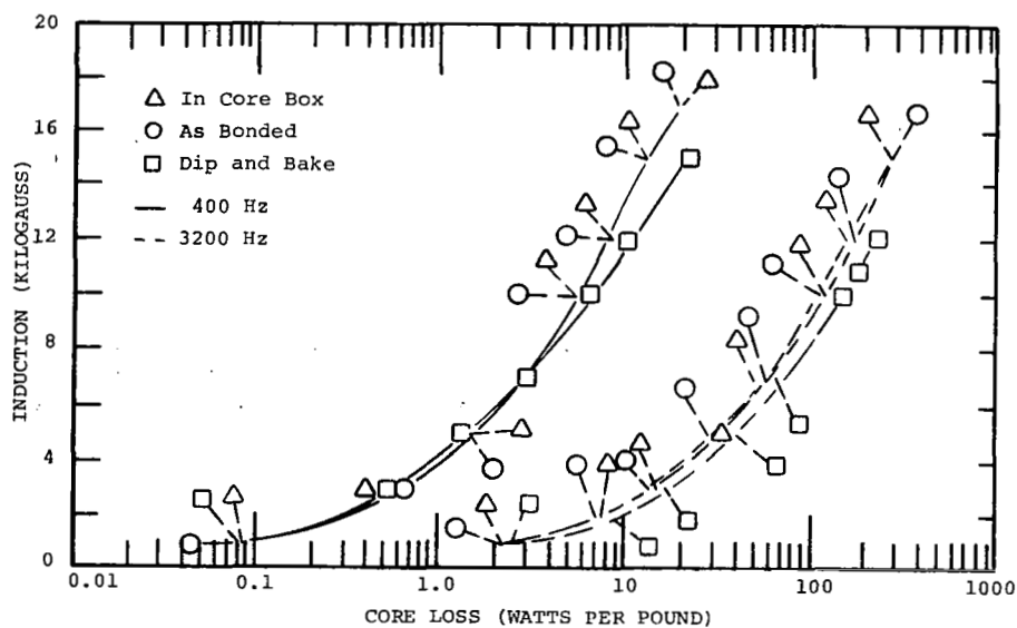
Figure 91. - Degradation Test, P_c , s_q , Total Core Loss, 0.006-Inch Doubly Grain Oriented Silicon Steel, Double Window, Stress Relief Annealed, Core 2, Room Ambient. Processing Variables: In Core Box, As Bonded, and Dip and Bake
