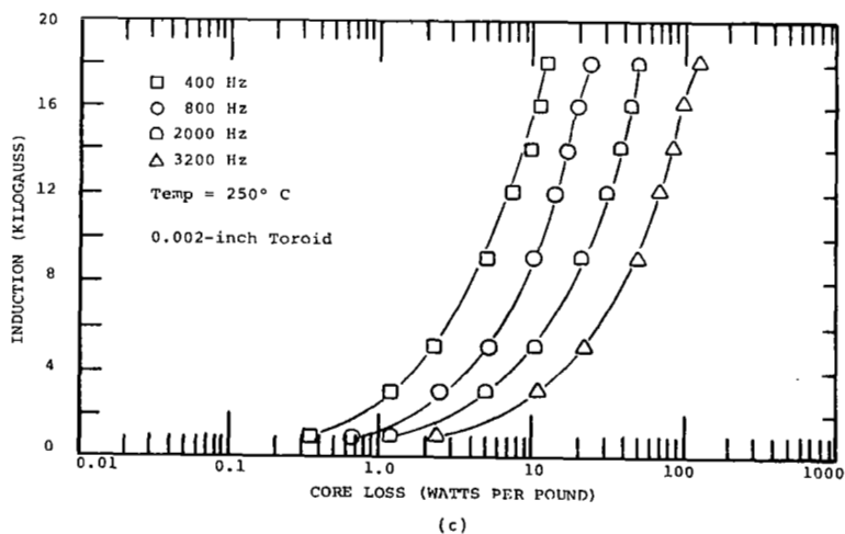
Figure 37. - P_{c, sq} , Total Core Loss vs Induction and Frequency, 0.002-Inch 49%Co-2%V-49%Fe Toroid, Magnetic Field Annealed
