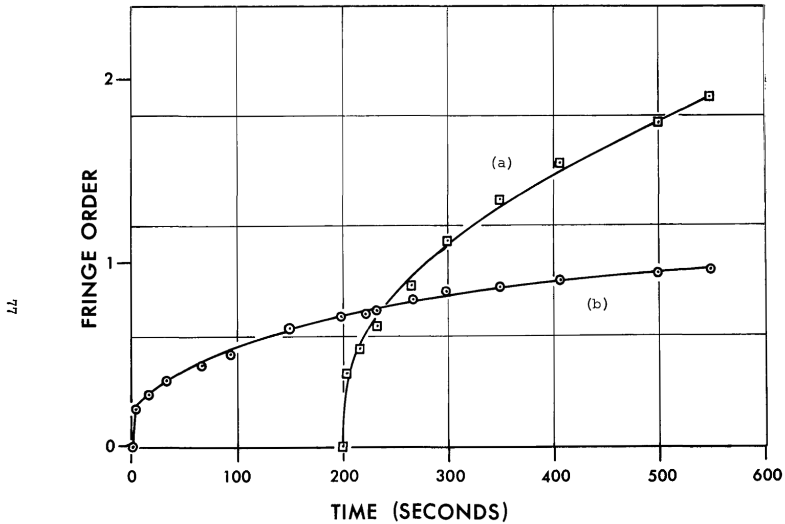
Figure 23. Tensile analog input fringe order functions. (a) n(t) \sin 2\zeta (b) n(t) \cos 2\zeta
