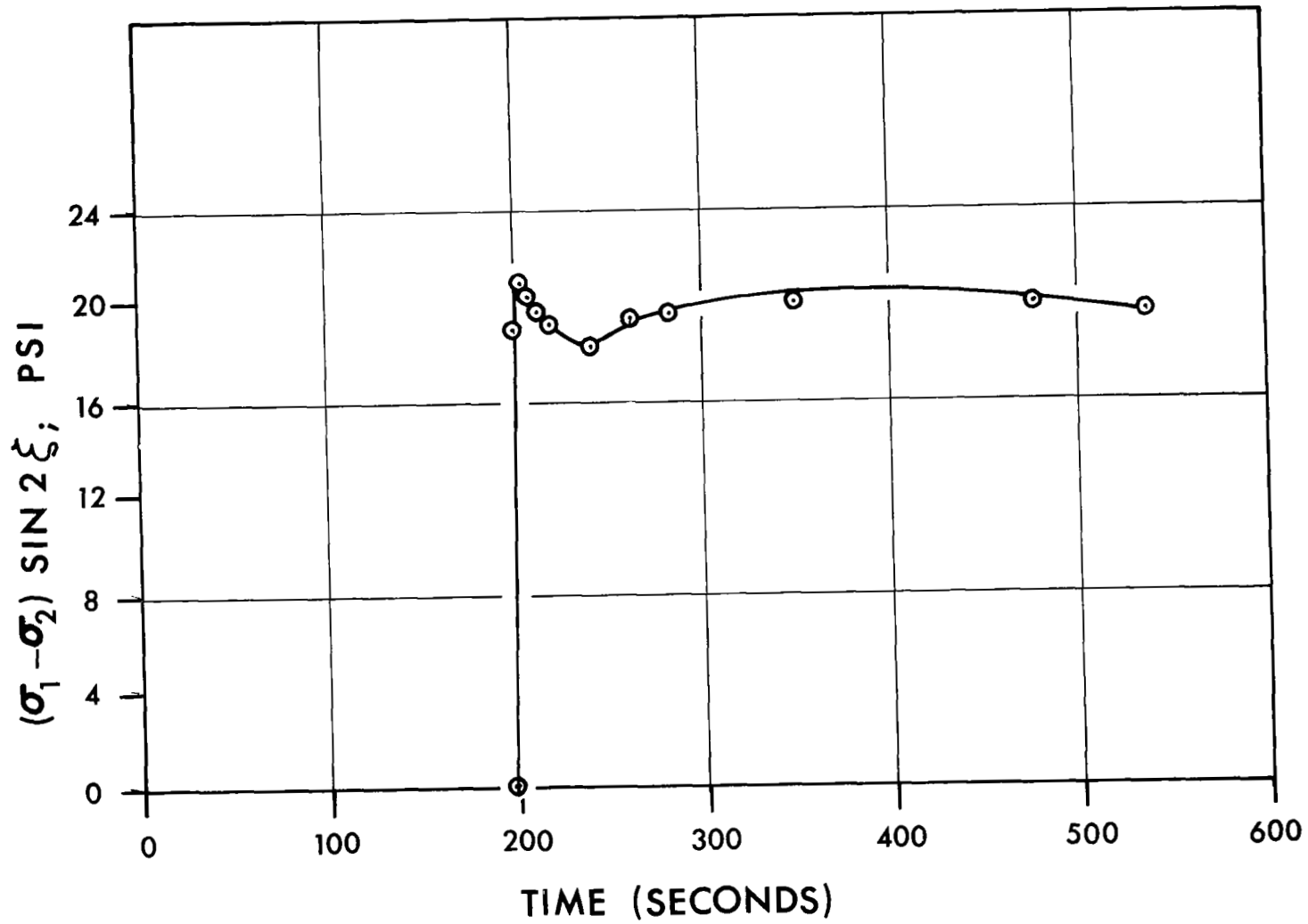
Figure 24. Output stress history from analog corresponding to input function n(t) \sin 2\xi
