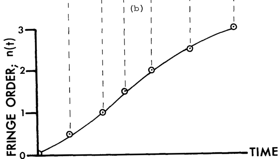
Figure 33. Relationship between light intensity variation and fringe order.
