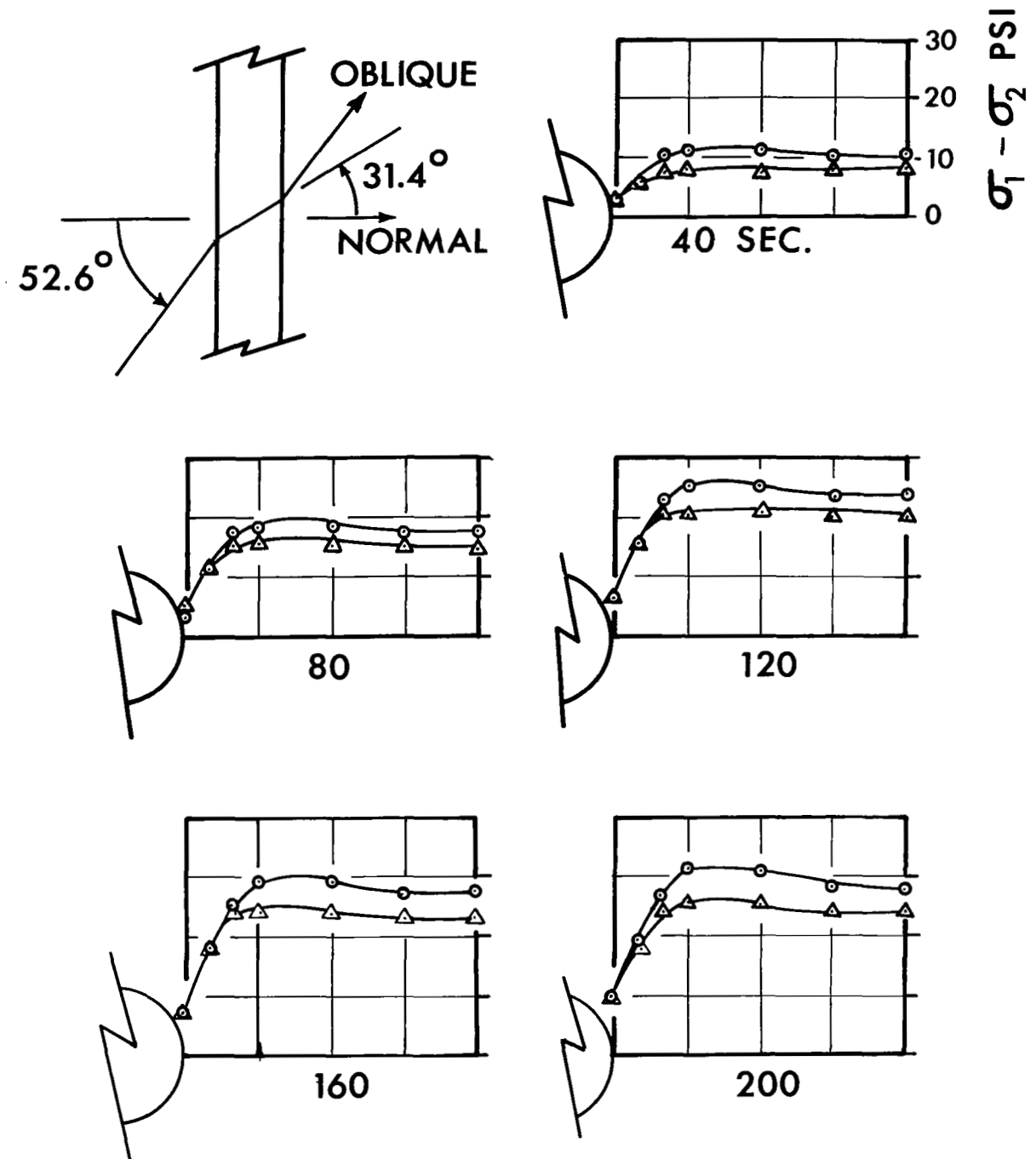
Figure 14. Normal and oblique stress-differences as determined with tensile analog.
