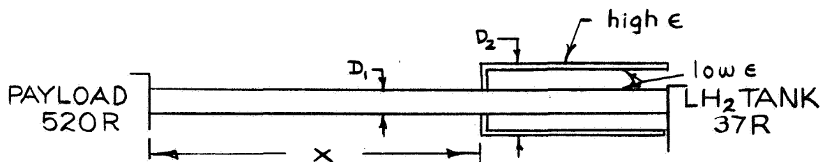
b) SUPPORTS WITH PANT LEG RADIATORS
