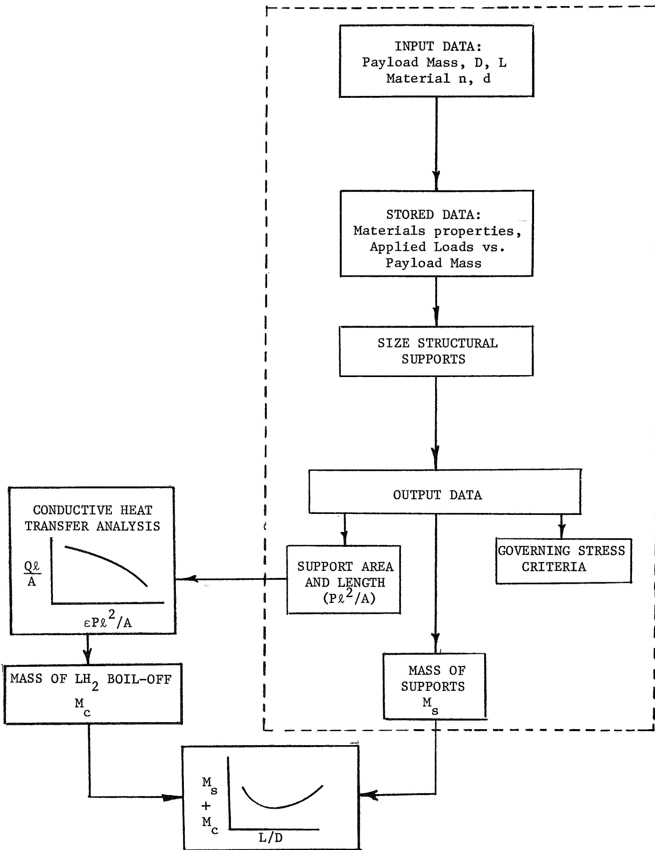
FIGURE 21 PARAMETRIC STUDIES OF FIXED STRUCTURES
