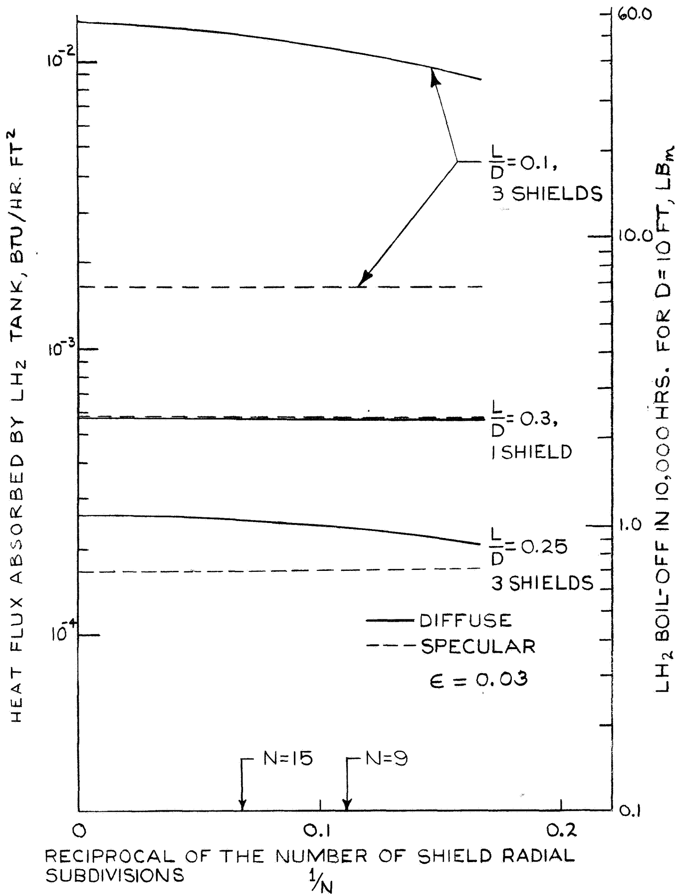
FIGURE 16 - EFFECT OF NUMBER OF RADIAL SUBDIVISIONS ON LH 2 BOIL-OFF
