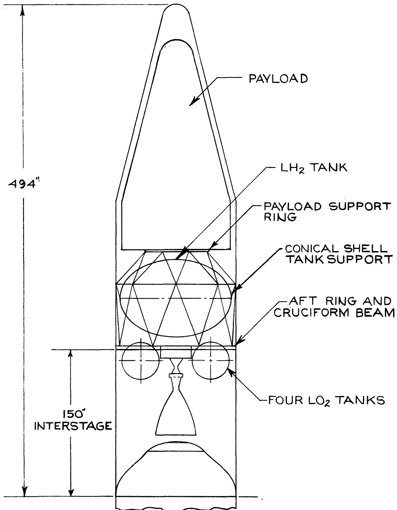
FIGURE 1-TYPICAL UPPER STAGE CONFIGURATION
