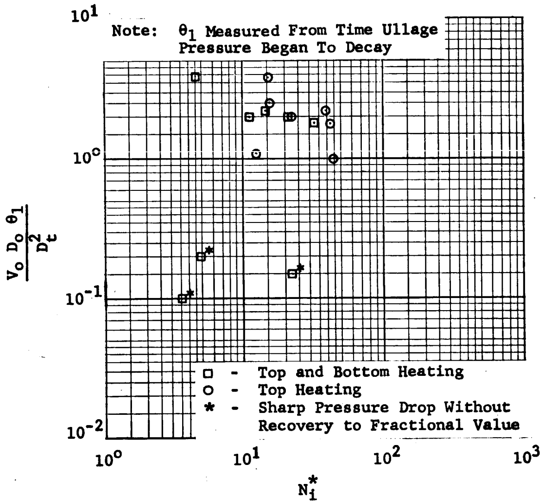
Figure 5-20 Correlation of Dimensionless Time For T_s - T_b To Reach 0.2 of Its Initial Value; Closed Tank Tests
