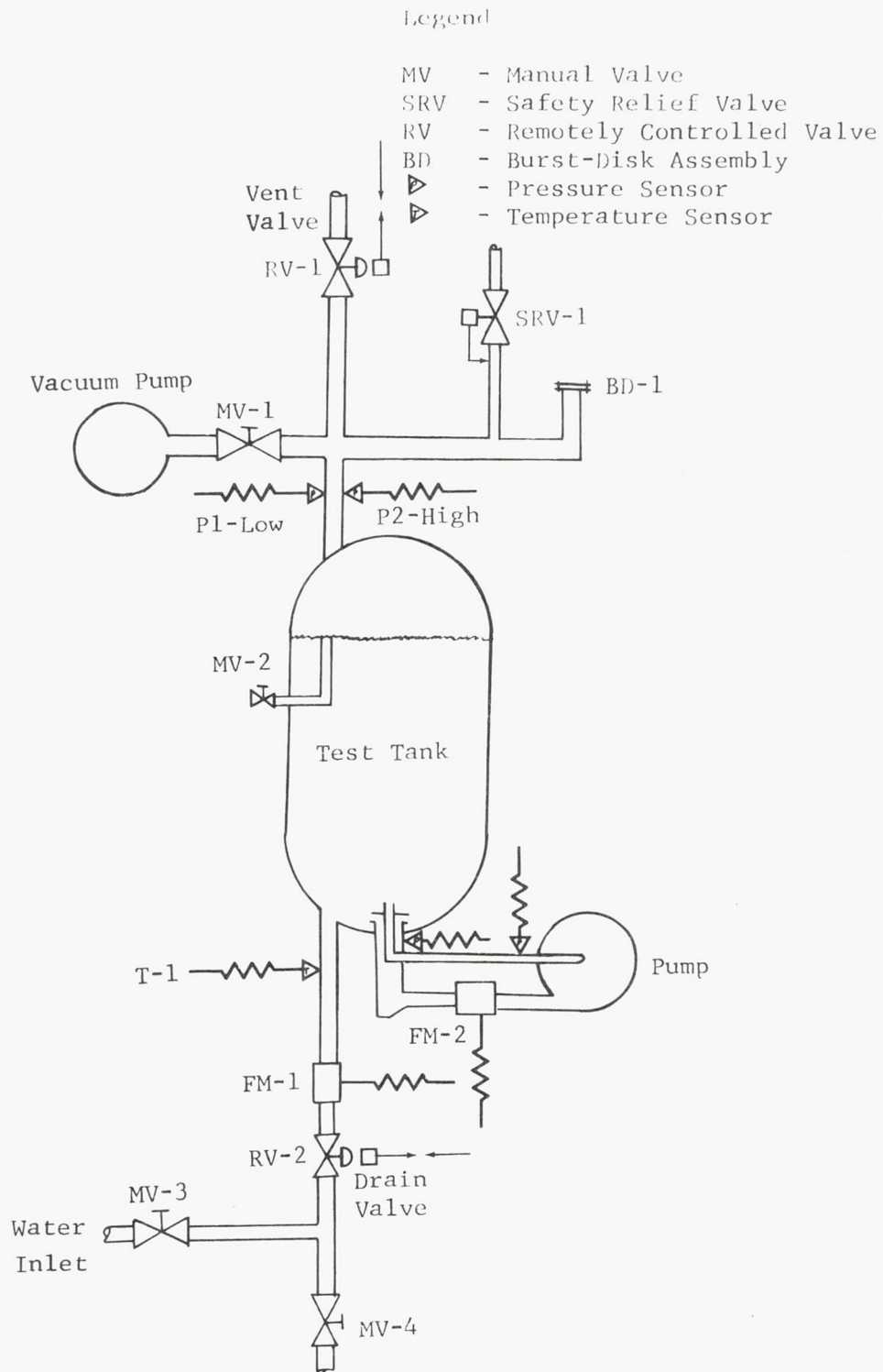
Figure 4-7 Schematic of the Closed Tank Test System
