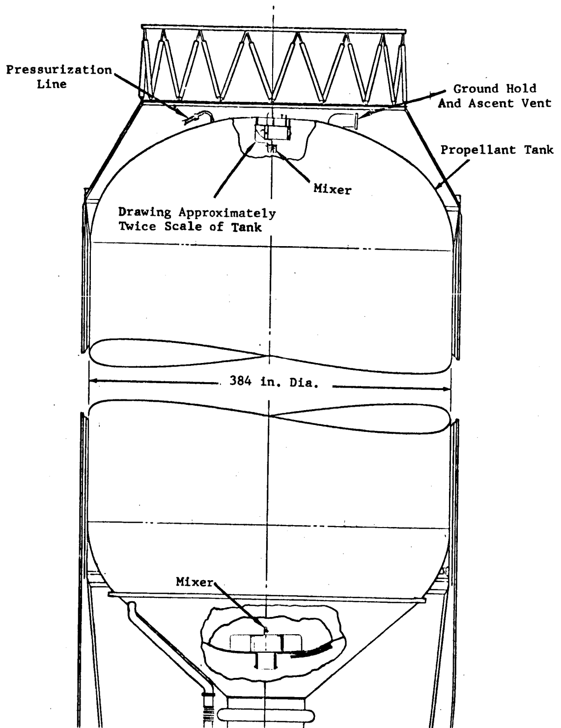
Figure 3-4 Mixer Installation in Nuclear Flight Module
