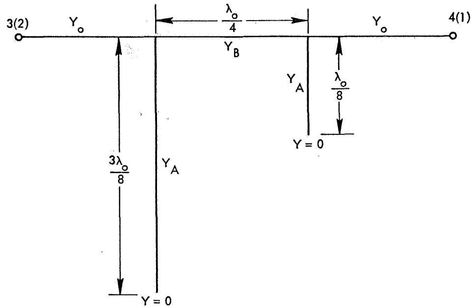
EVEN MODE REPRESENTATION, UNIT INPUT AT PORT 3
