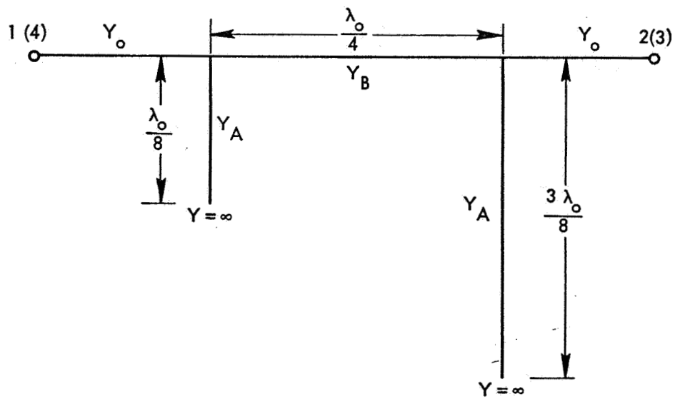
ODD MODE REPRESENTATION, UNIT INPUT AT PORT 1 FIGURE 12
