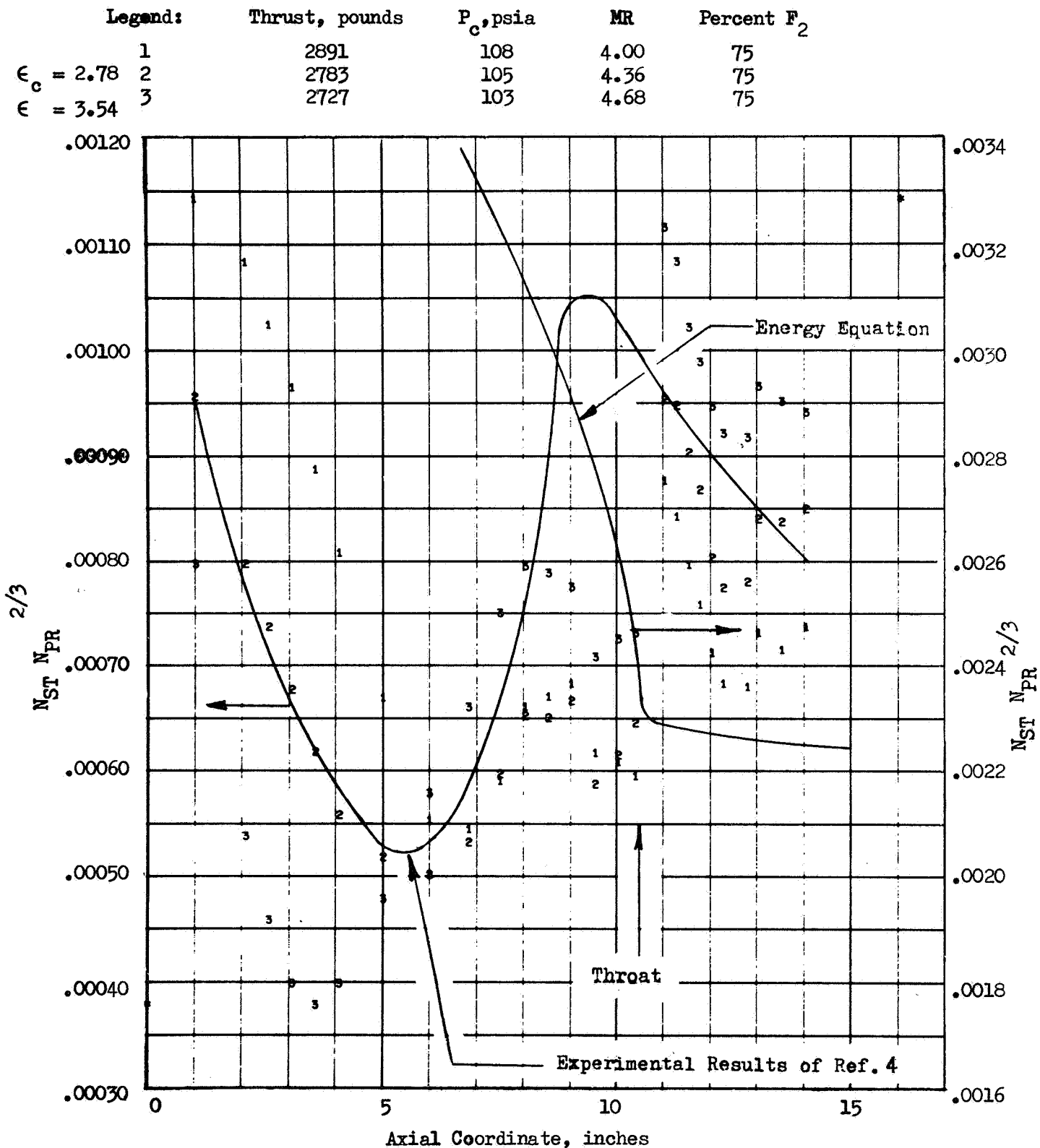
Figure B2 . Nondimensionalized Heat Transfer Rate vs Axial Coordinate for FLOX/Propane
