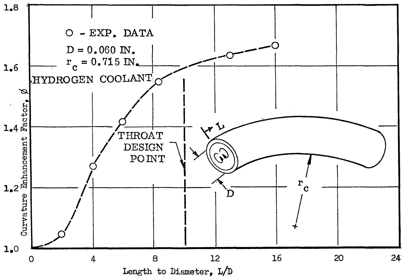
Figure E1. Coolant-Side Curvature Enhancement Factor
