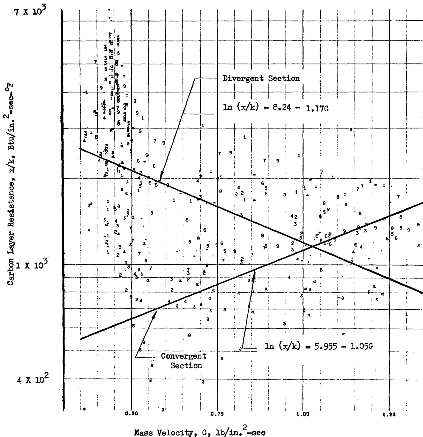
Figure B9 . Carbon Layer Resistance Correlation for FLOX/Methane
