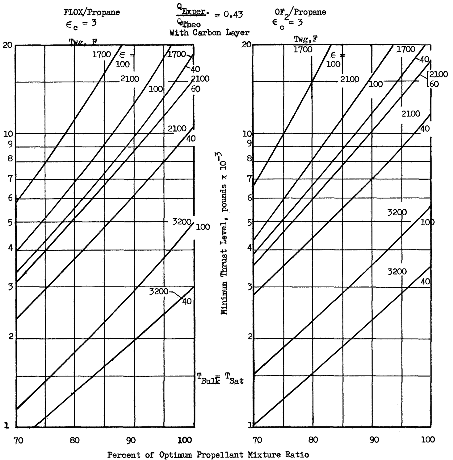
Figure 30 . Minimum Thrust Limits for Propane at P_c = 100 psia
