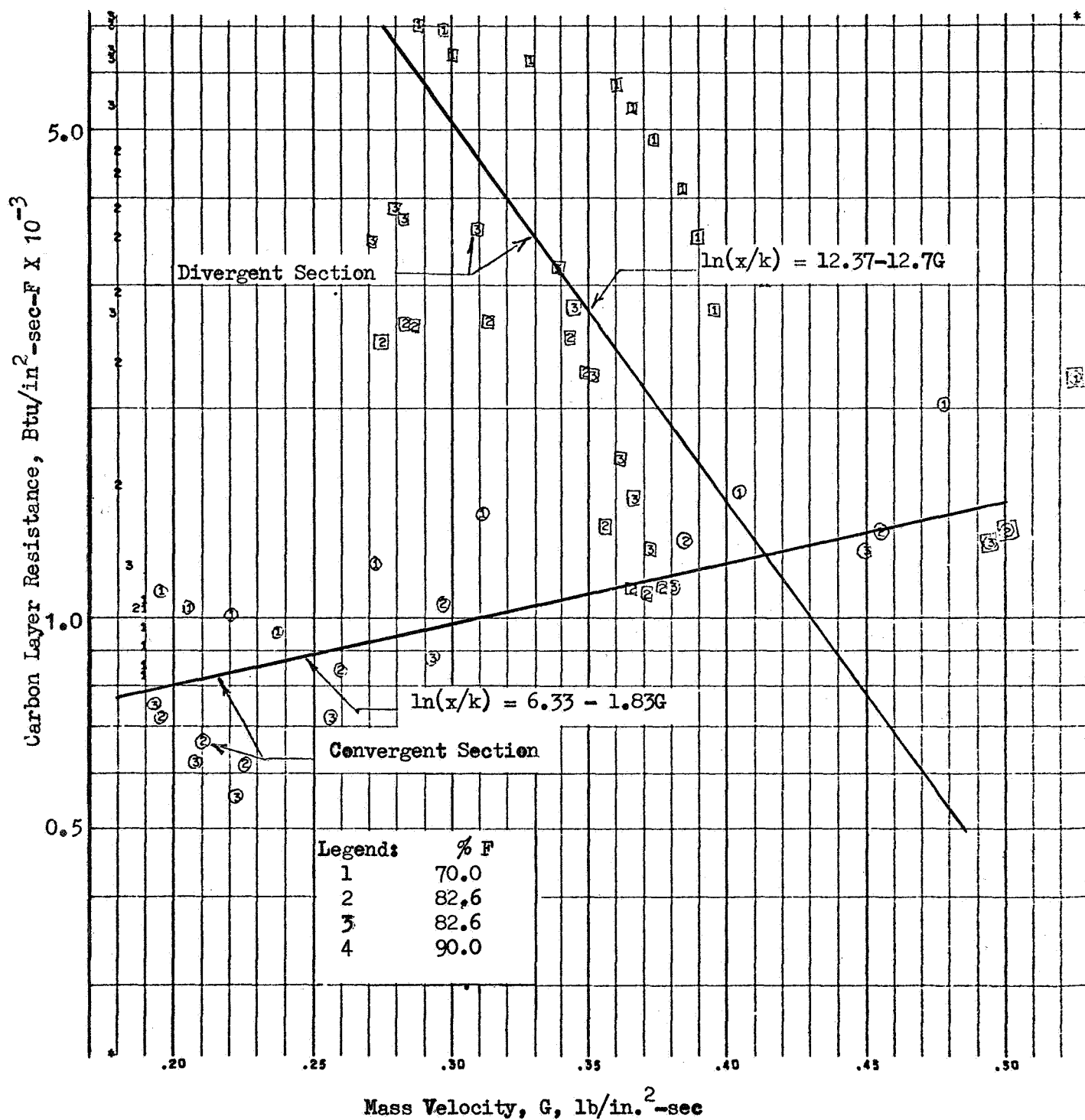
Figure B5. Carbon Layer Resistance Correlation for FLOX/Methane
