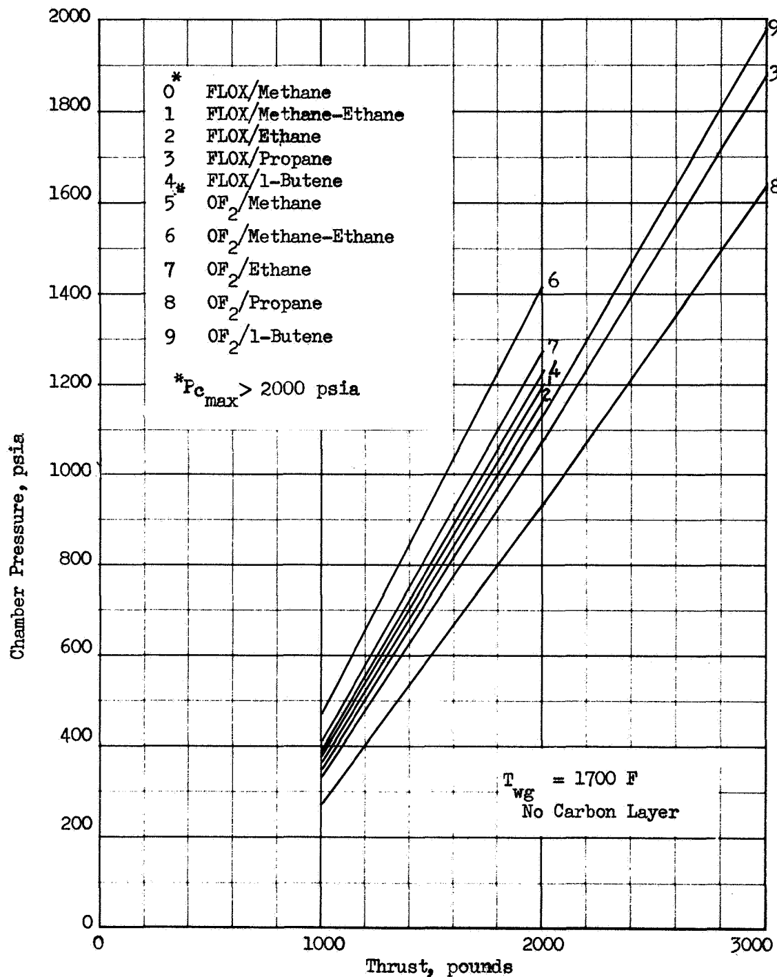
Figure 26. Regenerative Cooling Limits Based on Propellant Decomposition, \epsilon_c = 4 , \epsilon = 40
