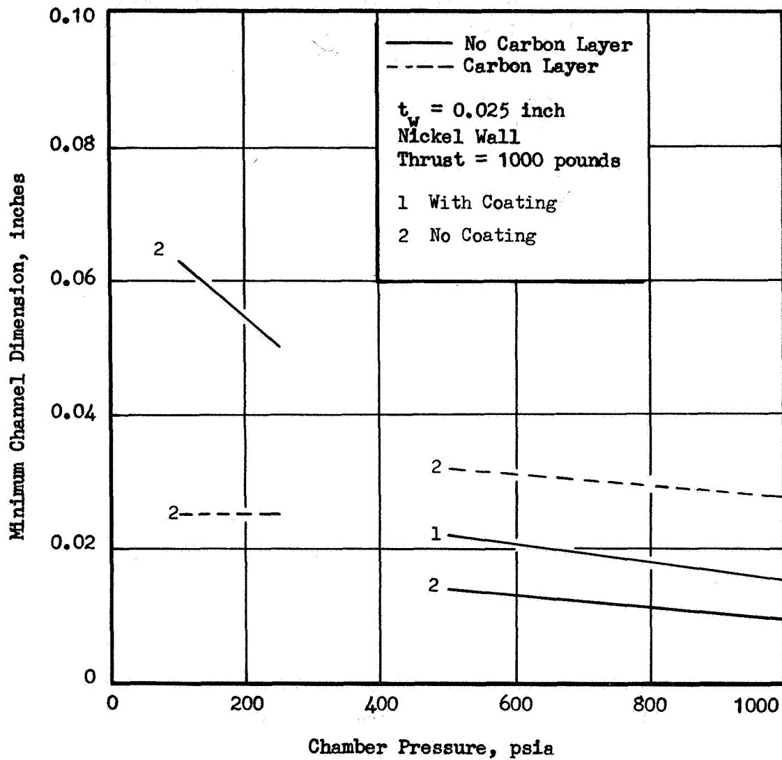
Figure 54. Channel Dimension vs Chamber Pressure for \text{OF}_2/1\text{-Butene}
