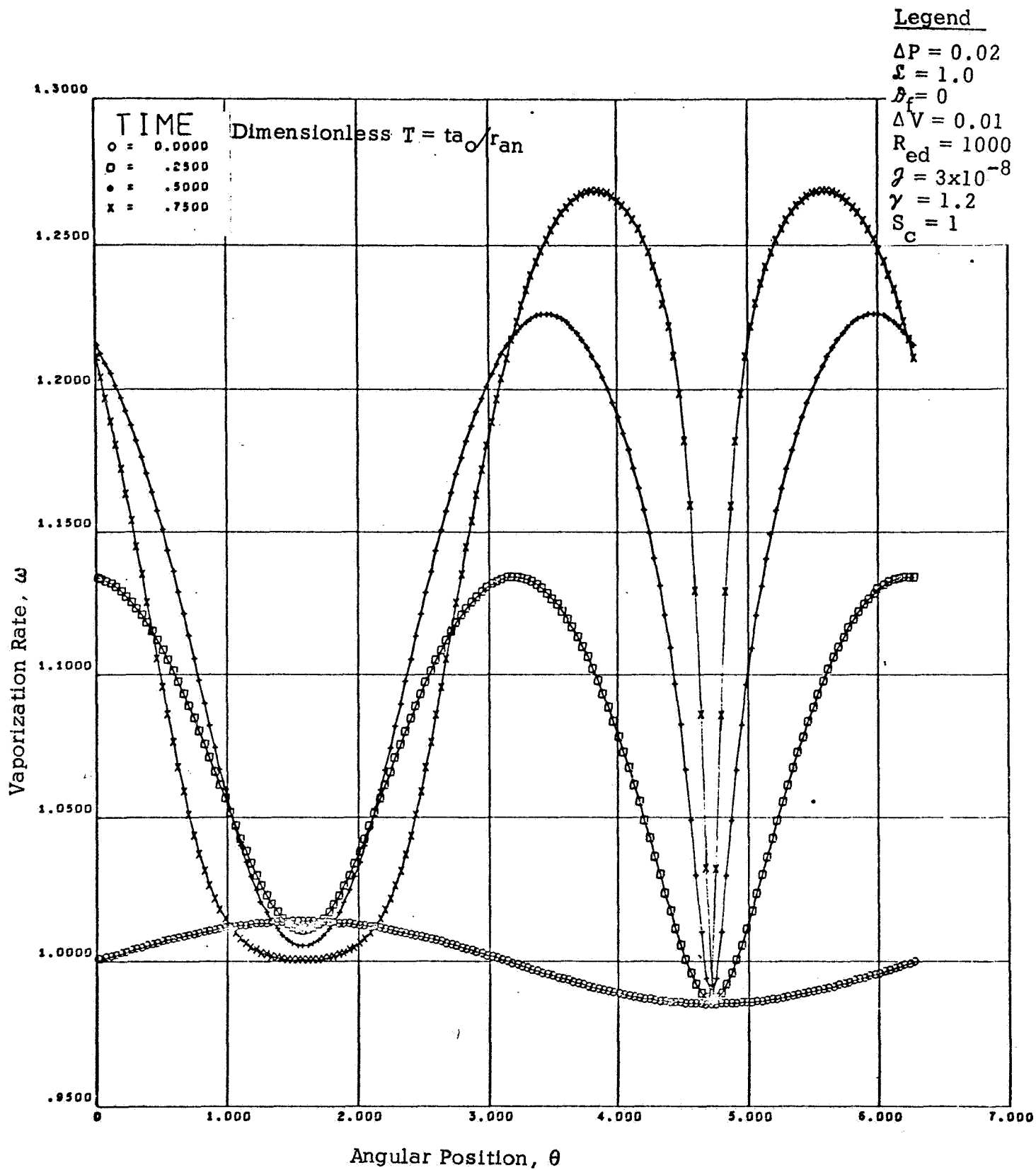
Figure 8. Time Growth of Vaporization Rate.
