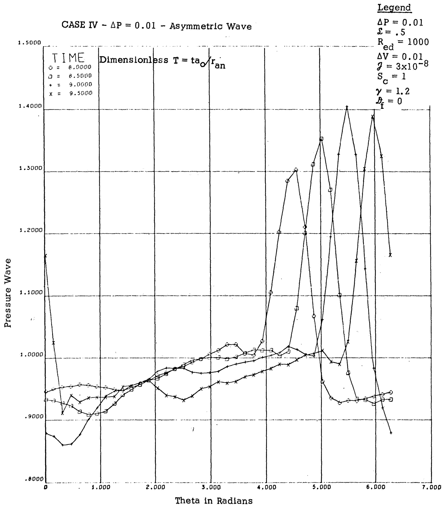
Figure 5. Growth of an Asymmetric Wave into a Single Traveling Pulse (time = 8.0 - 9.5)
