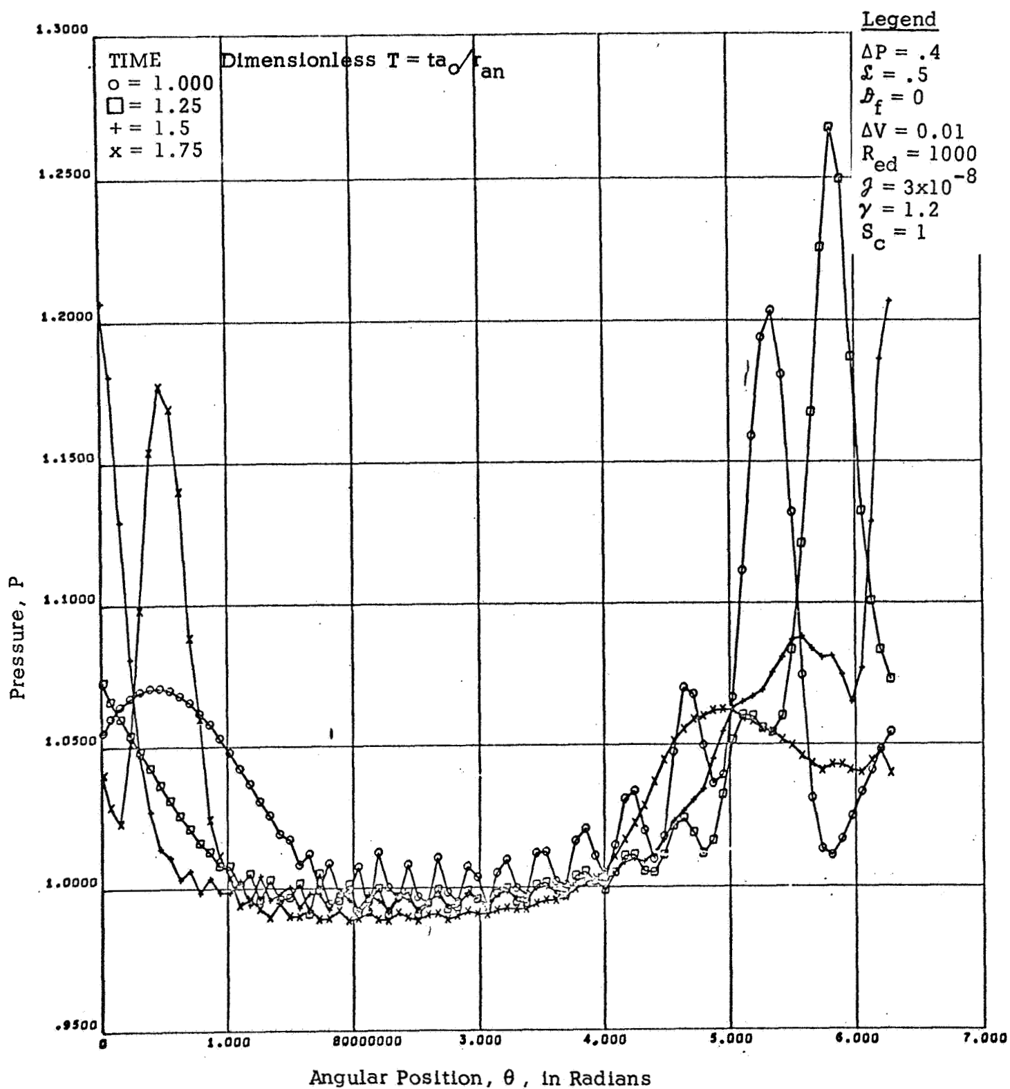
Figure 14b. Time History of a Discontinuous Pressure Disturbance (time = 1.0-1.75).
