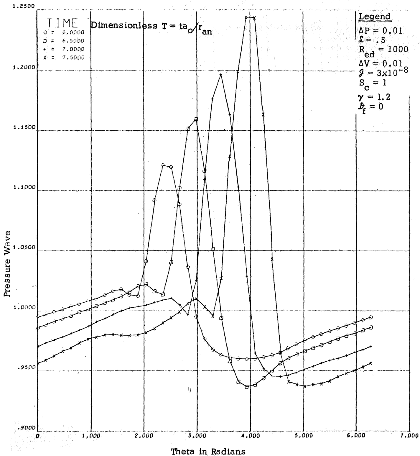
Figure 4. Growth of an Asymmetric Wave into a Single Traveling Pulse (time = 6.0 - 7.5)
