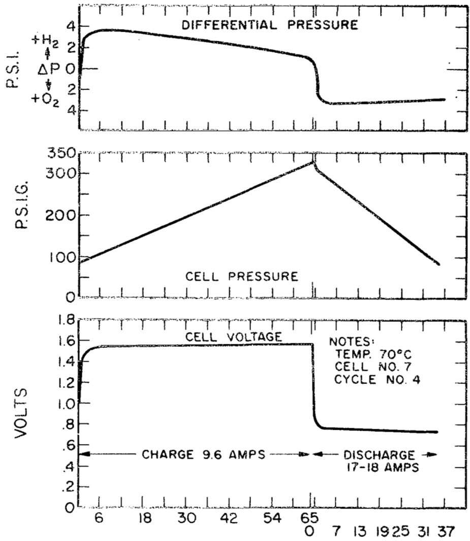
Figure 9. Cycling Data - Hydrogen-Oxygen Electrolytic Regenerative Fuel Cell
