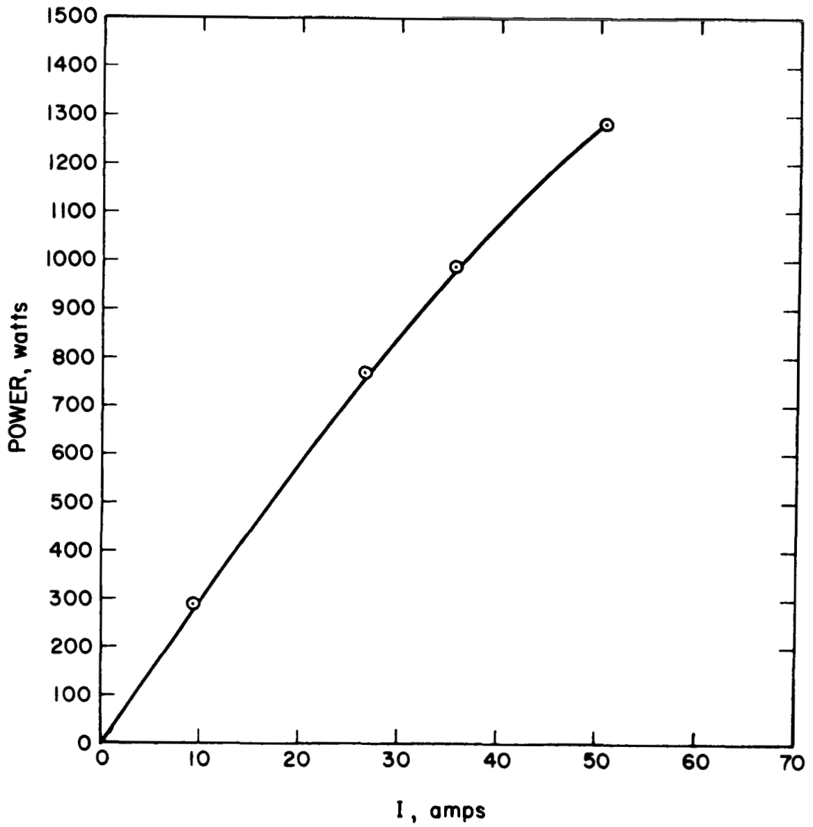
Figure 117. Power versus Current for 500-Watt Regenerative Hydrogen-Oxygen Fuel Cell S/N 1002-34
