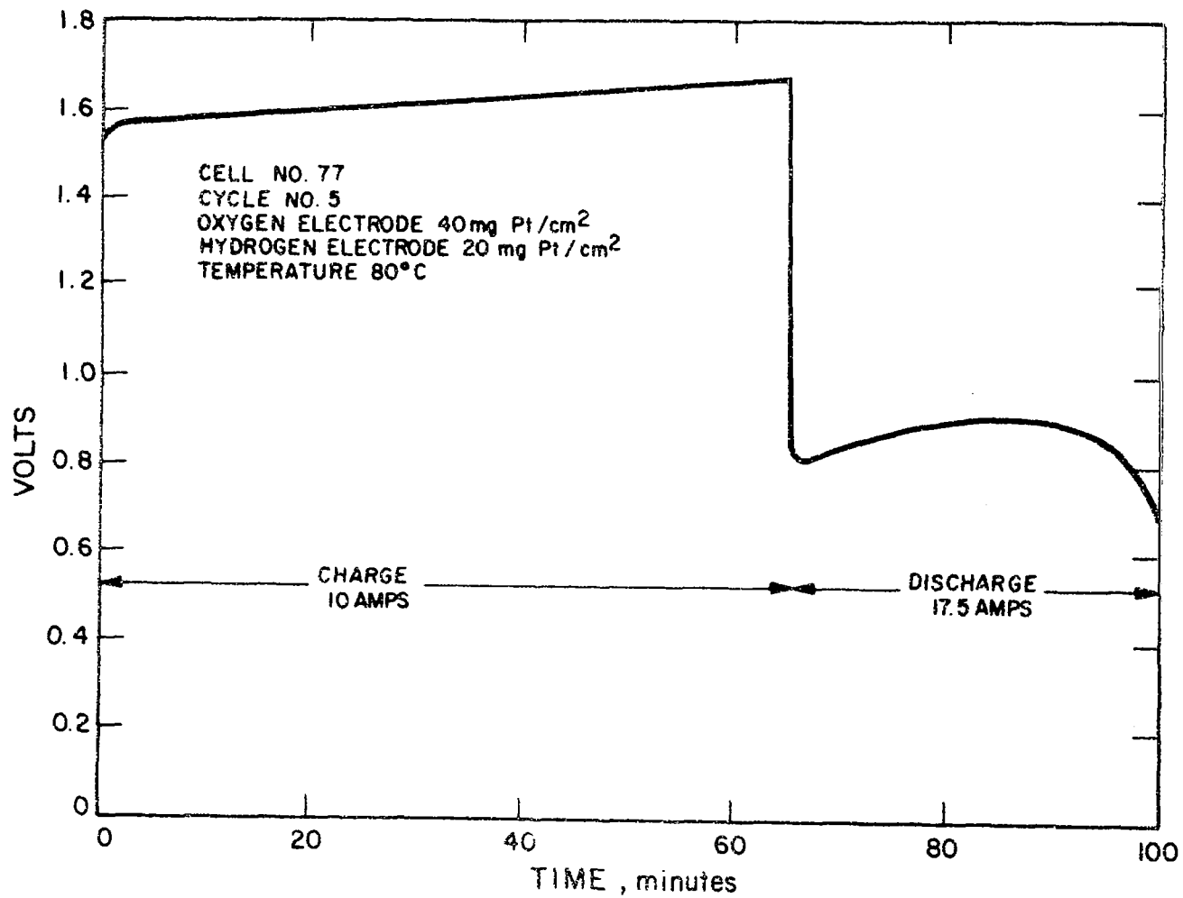
Figure 16. Performance Data of High Catalyst Loaded Oxygen Electrode
