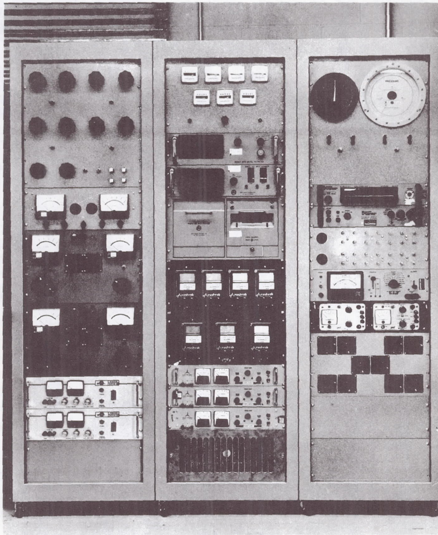
Figure 93. Fuel Cell Test Console
