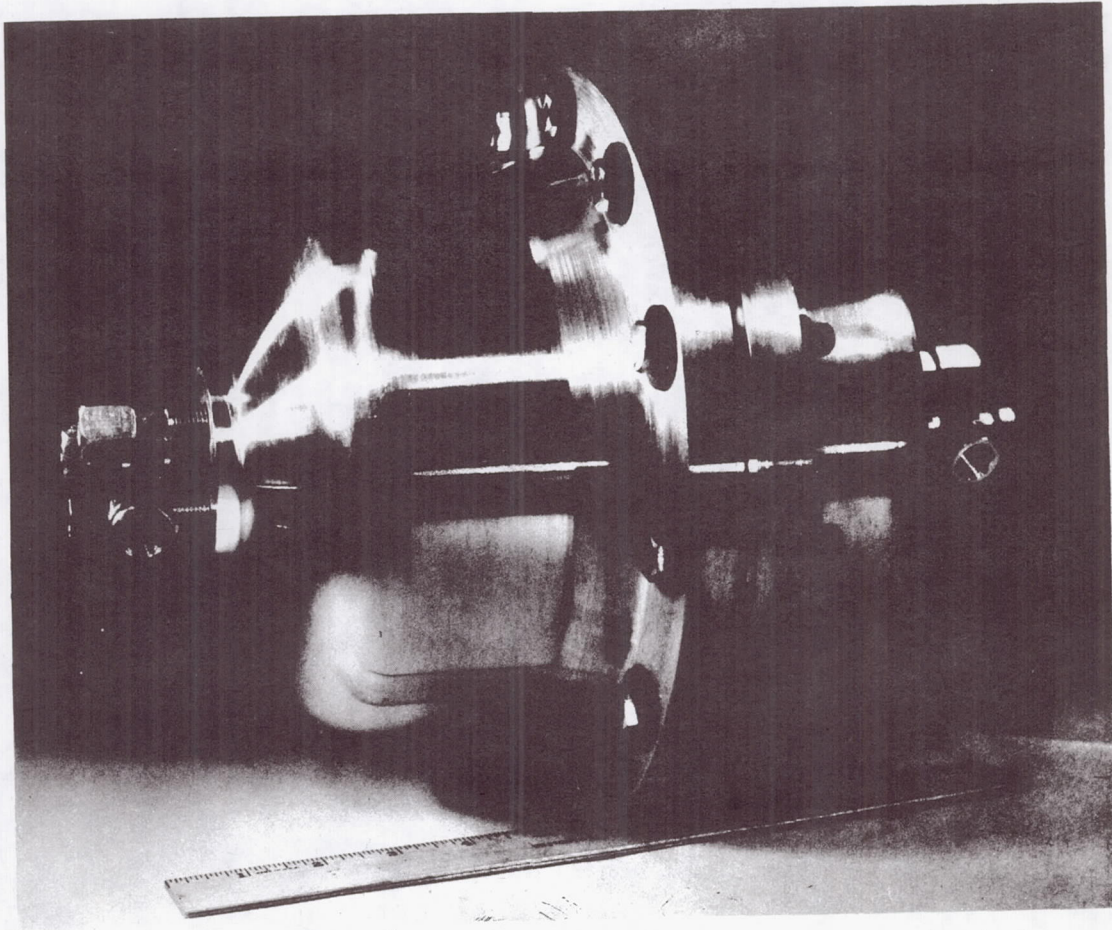
Figure 86. Six-Cell Fuel Cell Assembly
