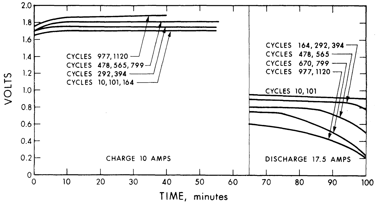
Figure 78. Cycling Performance of Cell 274
