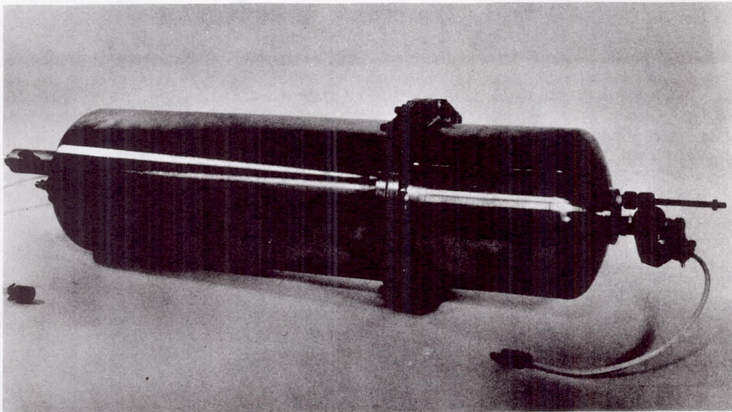
Figure 112. 500-Watt Regenerative Hydrogen-Oxygen Fuel Cell Assembly
