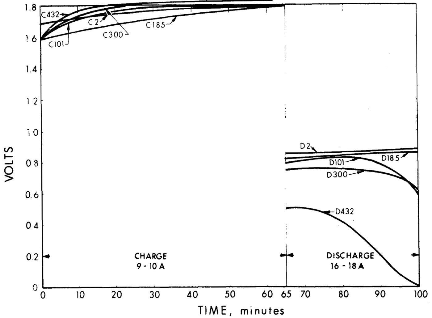
Figure 29. Cycling Performance of Cell 217
