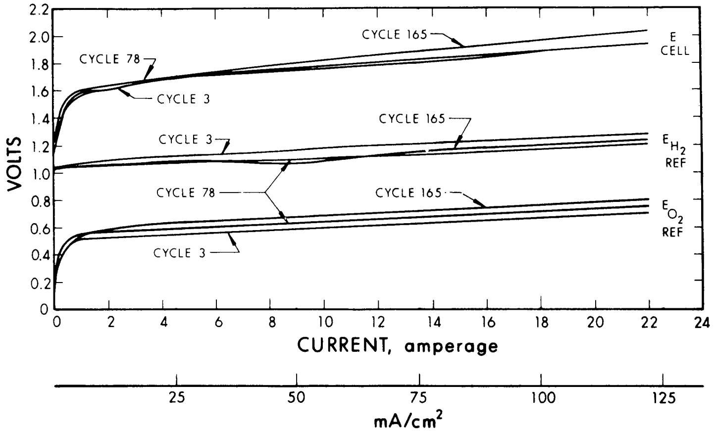
Figure 33. Charge Polarization at 80°C, Cell 250
