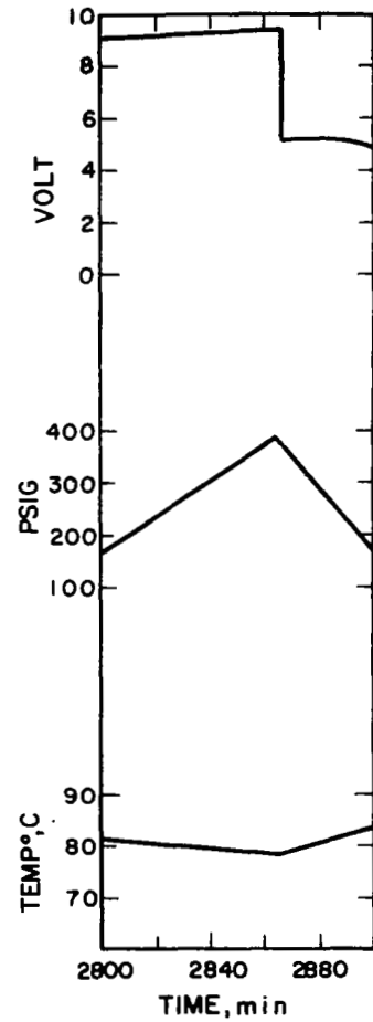
Figure 98. Continuous 48-Hour Cycling of 75 Watt Electrolytic Regenerative H_2-O_2 Fuel Cell
