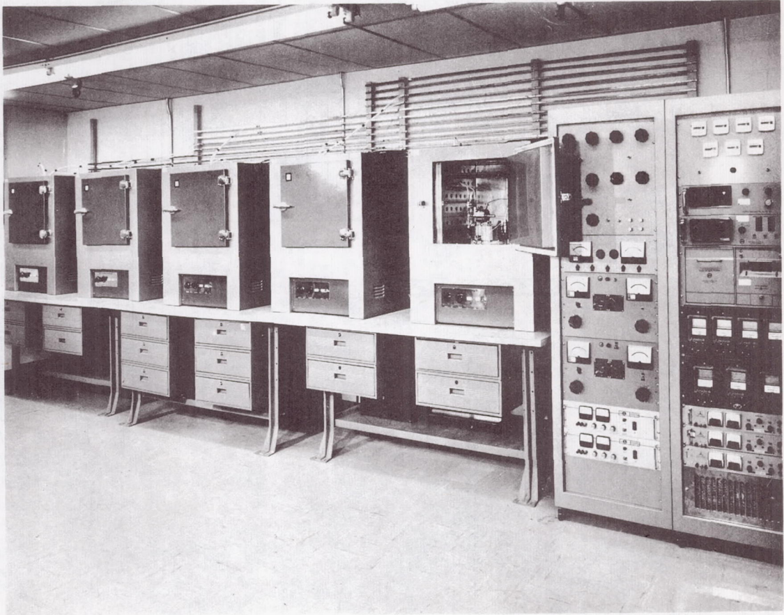
Figure 7. Single Fuel Cell Test Station
