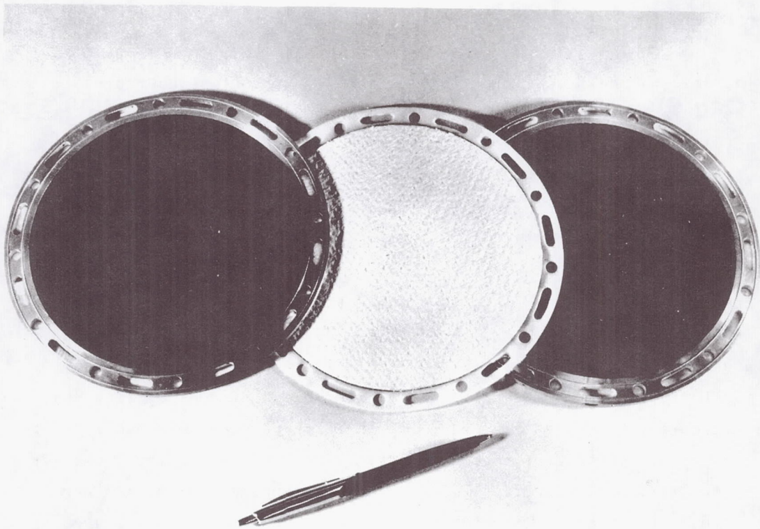
Figure 88. Electrode and Separator of Assembly
