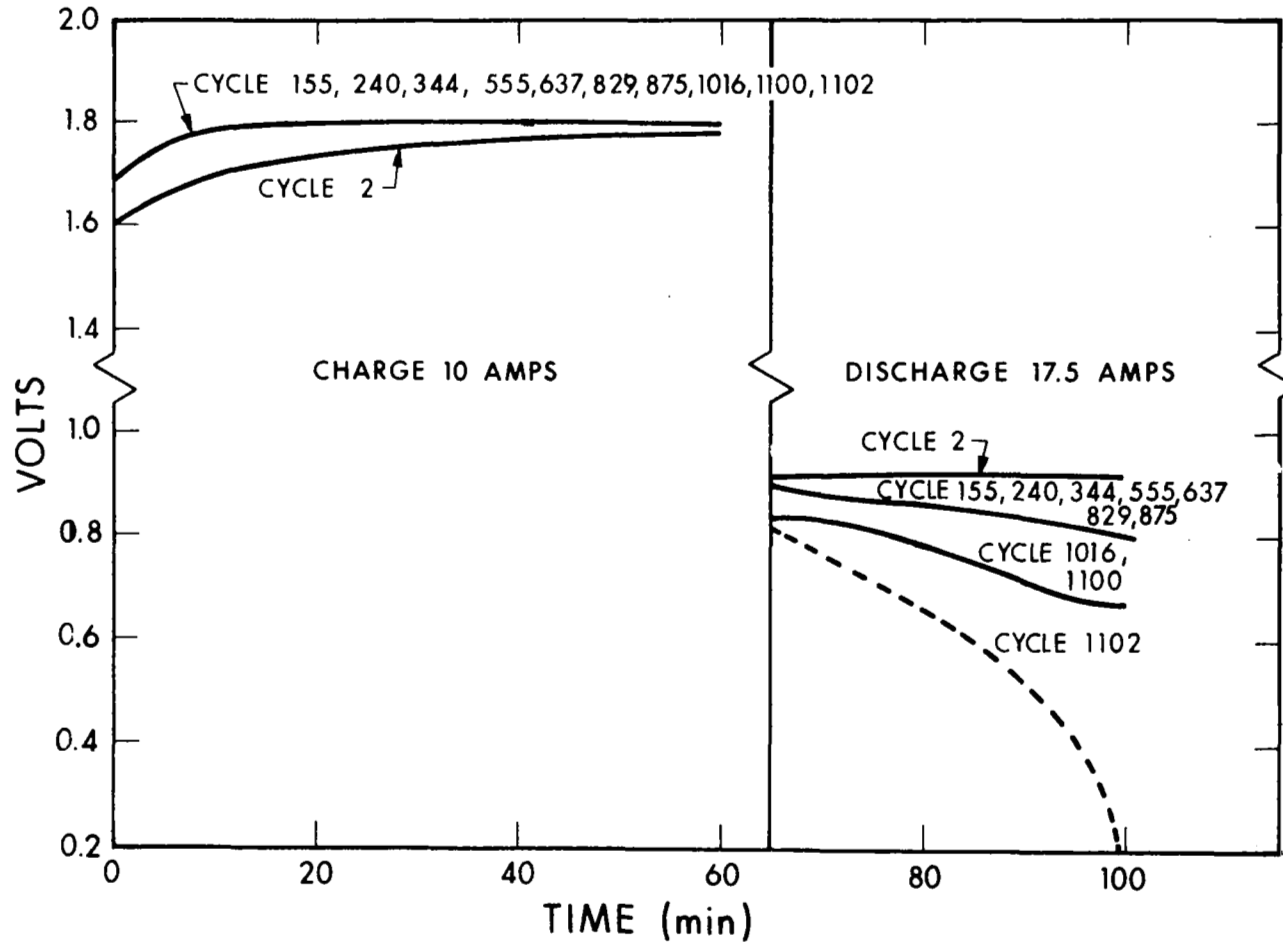
Figure 77. Cycling Performance of Cell 276
