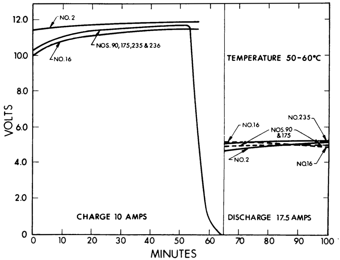
Figure 109. Cycling Performance of Six-Cell Unit S/N 115
