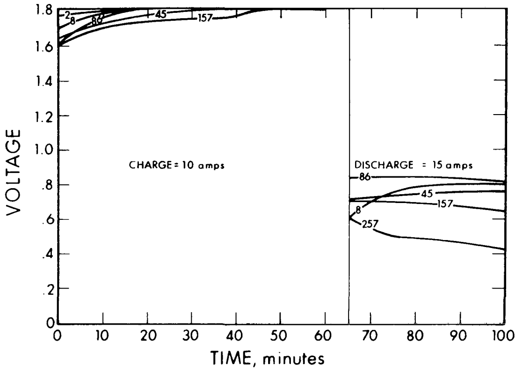
Figure 68. Cycling Performance of Cell 246
