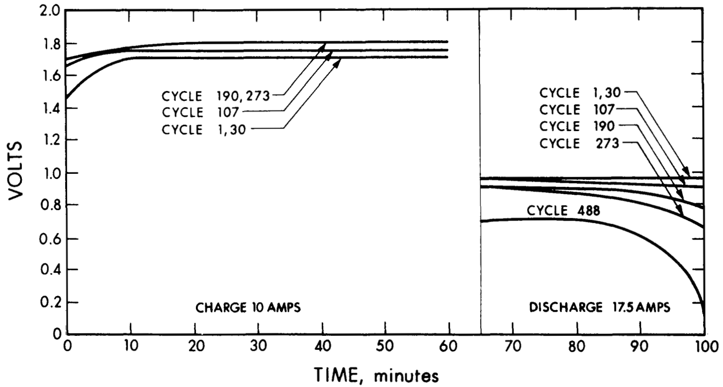
Figure 79. Cycling Performance of Cell 282
