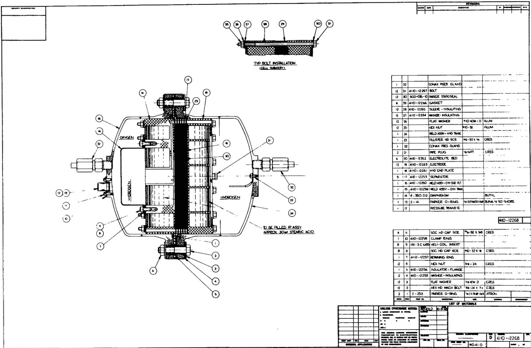
Figure 85. Six-Cell Fuel Cell Assembly
