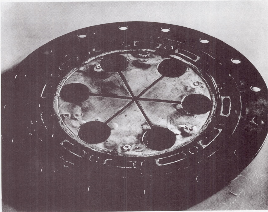
Figure 110. H 2 End Plate From Six-Cell Unit S/N 115
