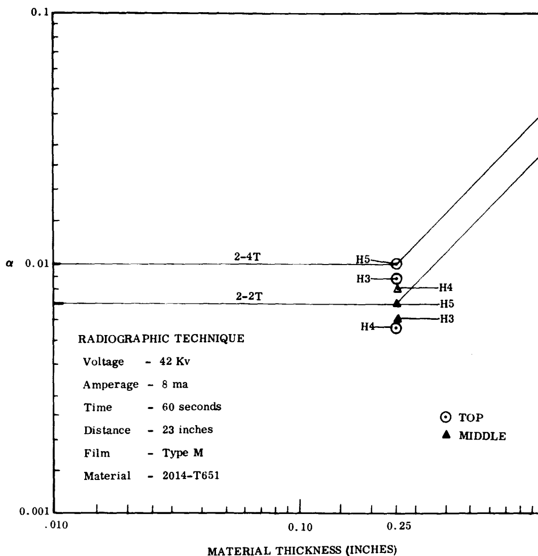
Figure 15. Minimum \alpha Observed in H5, H4 and H3 Penetrameters Compared to Quality Levels Required by MIL-STD-453
