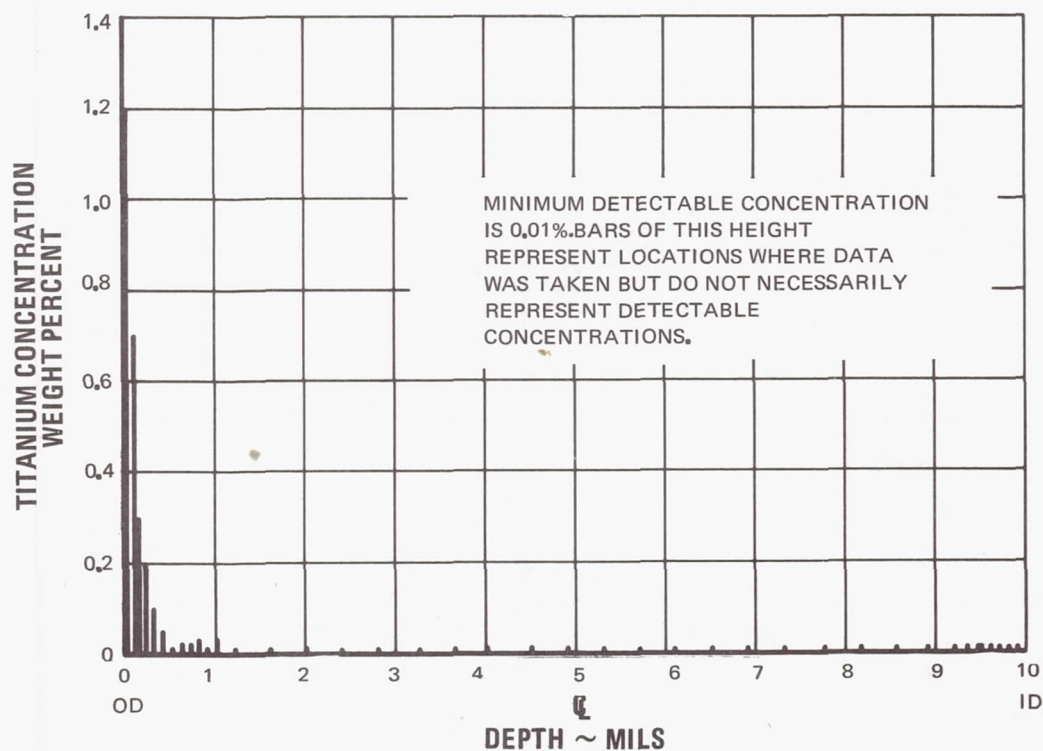
Figure 65 Concentrations of Aluminum and Titanium Across Columbian-1 Percent Zirconium Tube Coated With Aluminum-Oxide-Aluminum Titanate and Endurance Tested at 1700°F for 10,000 Hours
