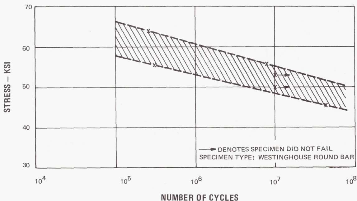
Figure 20 Fatigue Test Results Obtained at Room Temperature for AISI-310 Stainless Steel
