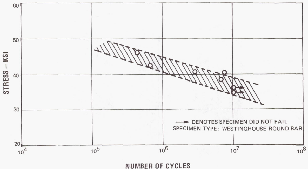
Figure 24 Fatigue Test Results Obtained at Room Temperature for Columbium-1 Percent Zirconium Coated With Iron Titanate
