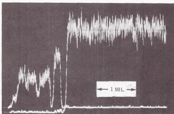
Figure 74 X-ray Line Scan Intensities for Titanium and Columbian Across Interface of Iron Titanate and Columbian-1 Percent Zirconium After 5,000 Hours of Testing Between 1500°F and 1800°F
