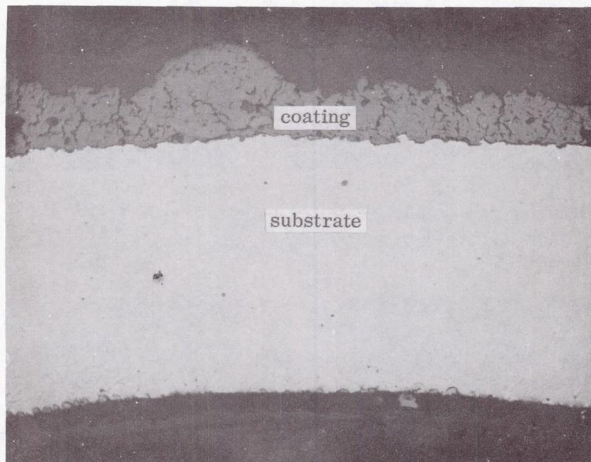
Figure 38 Unetched Photomicrograph of AISI-310 Stainless Steel Tube Coated With Calcium Titanate and Tested for 20,000 Hours at 1350°F
