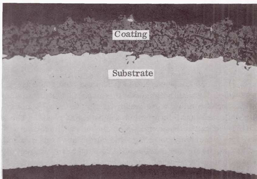
Figure 45 Photomicrographs of AISI-310 Stainless Steel Tube Coated With Iron Titanate and Tested for 20,000 Hours at 1350°F
