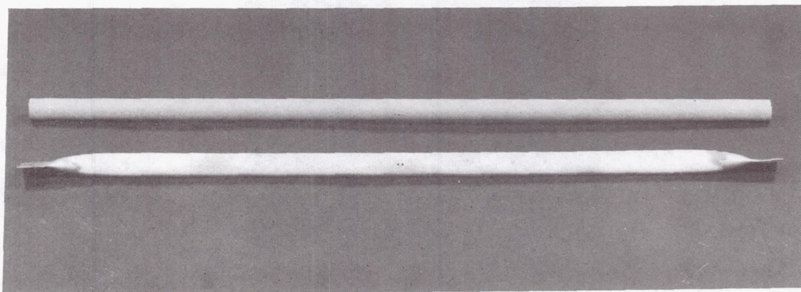
Figure 60 Appearance of Aluminum-Oxide-Aluminum-Titanate-Coated Columbium-1 Percent Zirconium Tube Before (Top) and After (Bottom) Testing for 10,000 Hours at 1700°F Mag: 0.5X XP-64742
