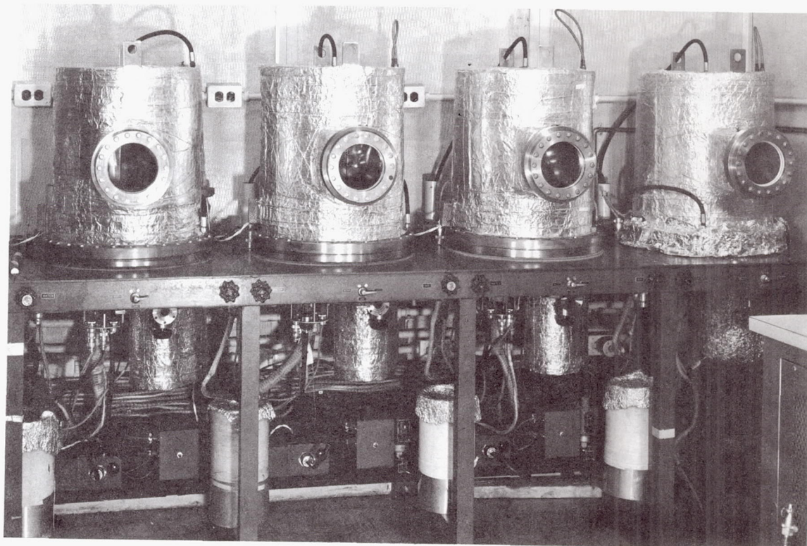
Figure 18 Long-Term Endurance Total Hemispherical Emittance Test Chambers XP-23123
