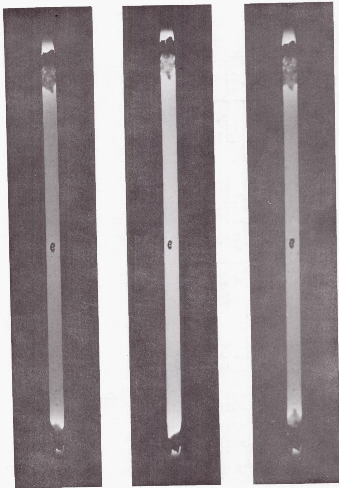
Figure 43 Appearance of Iron-Titanate-Coated AISI-310 Stainless Steel Tube at 1350°F After 15,400 Hours (Left), 17,500 Hours (Center), and 20,000 Hours (Right) Showing Progression of Coating Separation
