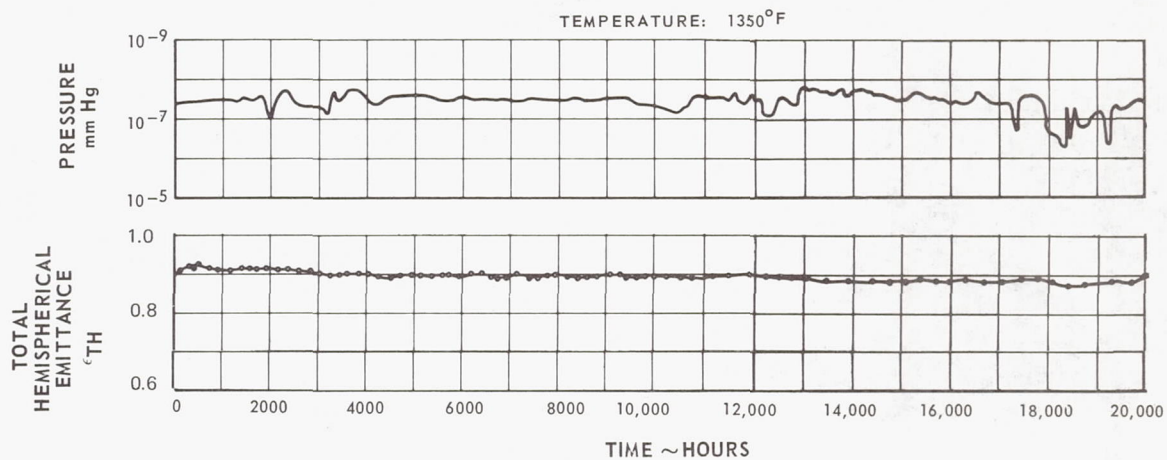
Figure 34 Pressure and Total Hemispherical Emittance for Long-Term Endurance Test of Calcium-Titanate-Coated AISI-310 Stainless Steel
