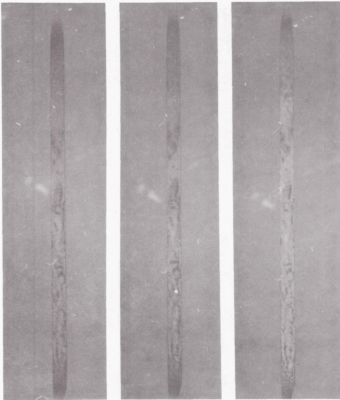
Figure 77 Iron-Titanate-Coated Columbium-1 Percent Zirconium Tube at 1500°F (Left), 1700°F (Center), and 1900°F (Right) in Vacuum Prior to Completion of 10,000-Hour 1500°F to 1900°F Cycling Test
