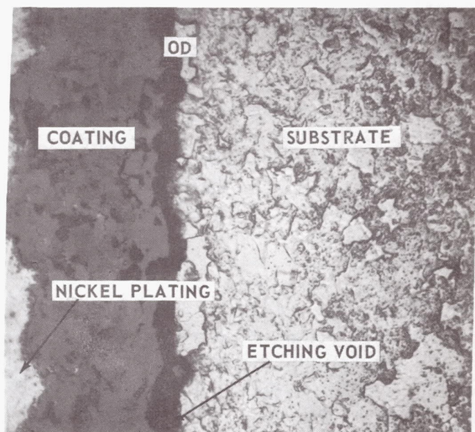
Figure 54 Cross Sectional Photomicrograph of Iron-Titanate-Coated Columbium-1 Percent Zirconium Tube After Endurance Testing at 1700°F for 10,000 Hours
