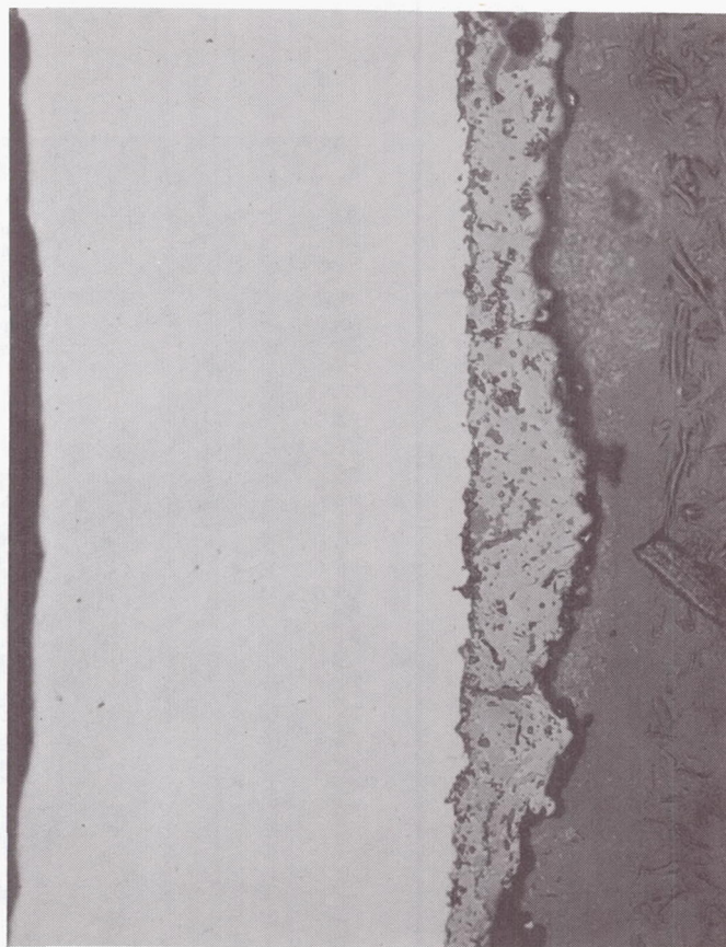
Figure 51 Photomicrograph of Iron-Titanate on Columbiu-1 Percent Zirconium After 10,000 Hours of Testing at 1700°F
