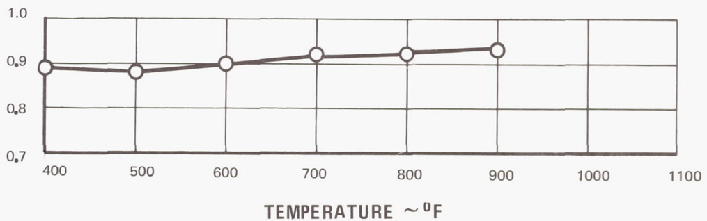
Figure 7 Total Hemispherical Emittance Measurement Results for Calcium-Titanate-Coated Beryllium Plates Using Thermal Decay Method
