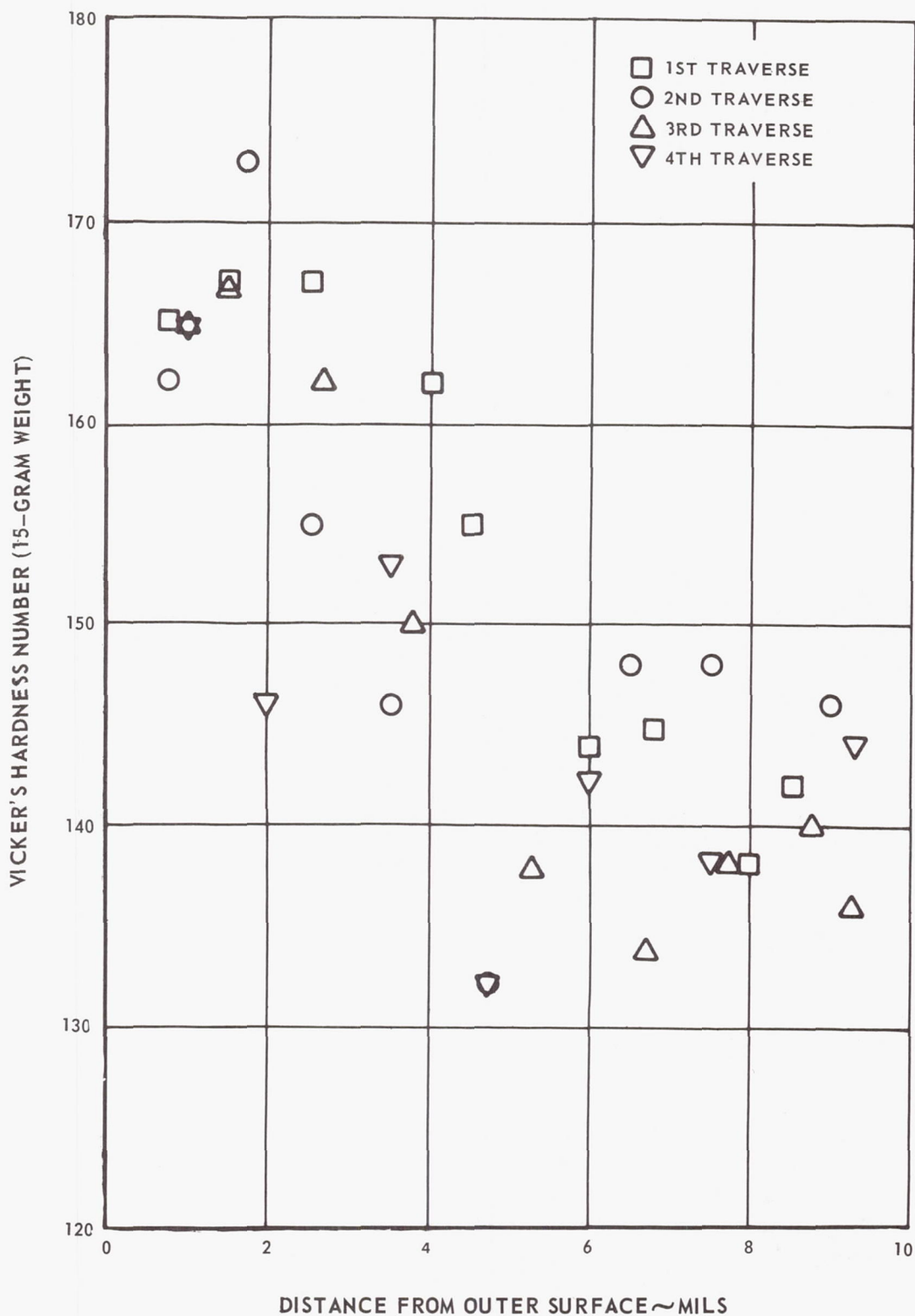
Figure 79 Hardness Traverse Test Results for Substrate of Iron-Titanate-Coated Columbium-1 Percent Zirconium Tube After Cycling Between 1500°F and 1900°F for 10,000 Hours
