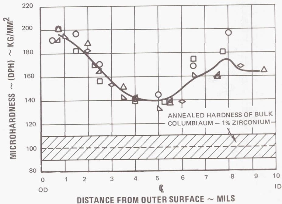
Figure 52 Microhardness Traverse Results for Endurance-Tested Columbium-1 Percent Zirconium Tube Coated With Iron Titanate After 10,000 Hours at 1700^{\circ}\text{F}
