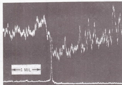
Figure 48 Relative X-ray Line Scan Intensities for Iron and Titanium Across Interface of Iron Titanate and AISI-310 Stainless Steel After Testing for 20,000 Hours at 1350°F
