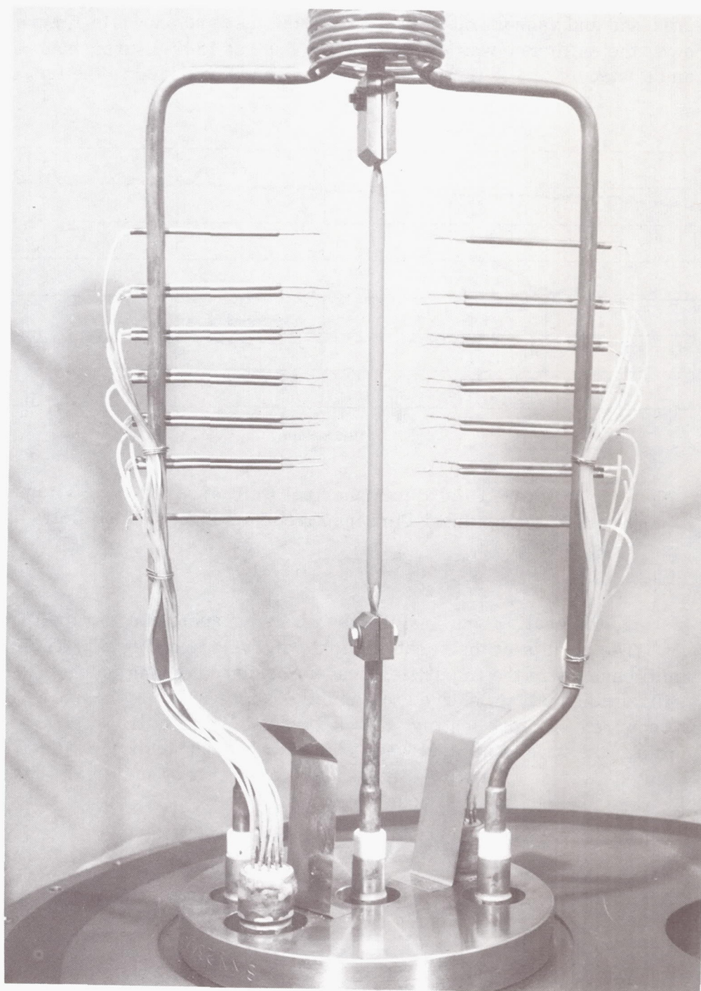
Figure 69 Mag: 0.6X Appearance of Iron-Titanate-Coated Columbium-1 Percent Zirconium Tube Thermally Cycled for 5,000 Hours Between 1500° and 1800°F X-24557
