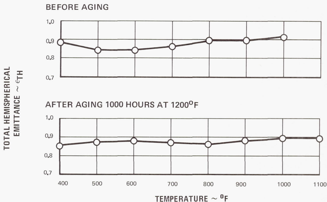
Figure 13 Total Hemispherical Emittance Measurement Results for Zirconium-Titanate-Coated Beryllium Plates
