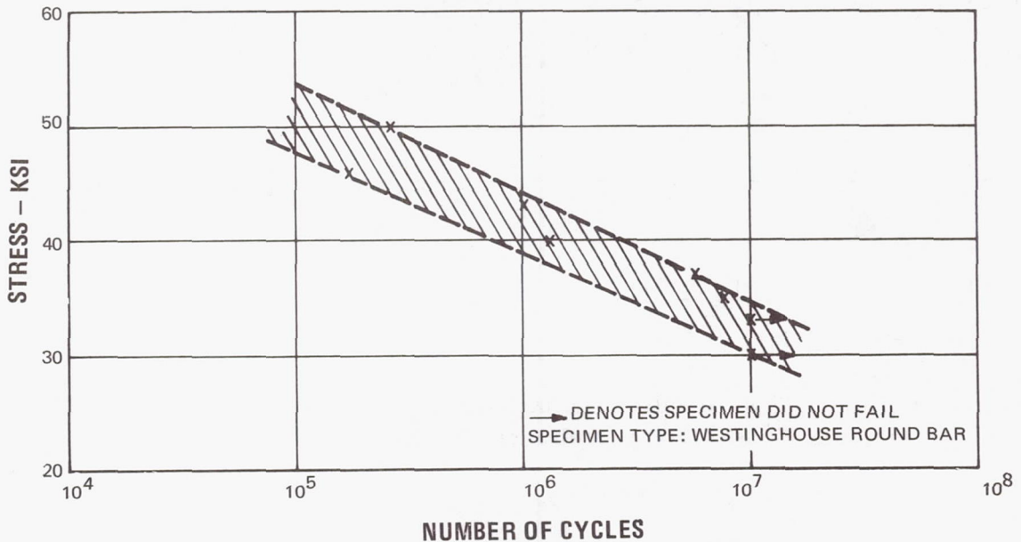
Figure 23 Fatigue Test Results Obtained at Room Temperature for Columbium-1 Percent Zirconium
