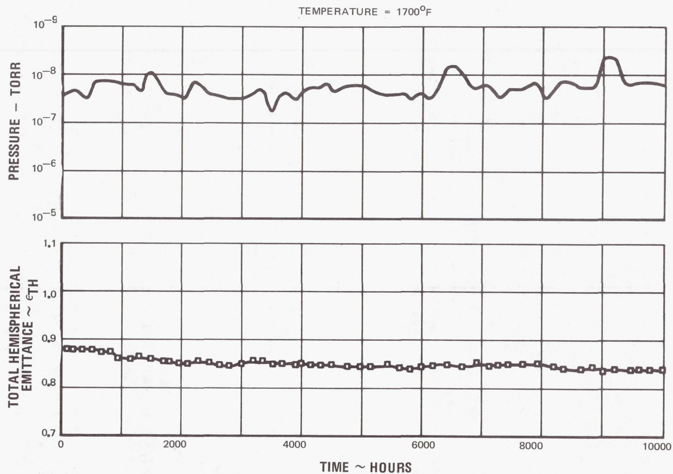
Figure 49 Pressure and Total Hemispherical Emittance for Iron-Titanate-Coated Columbian-1 Percent Zirconium Specimen
