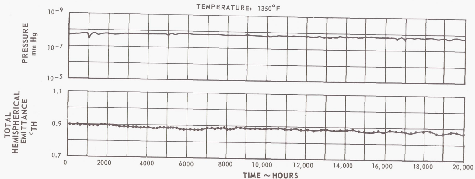
Figure 42 Pressure and Total Hemispherical Emittance for Long-Term Endurance Test of Iron-Titanate-Coated AISI-310 Stainless Steel
