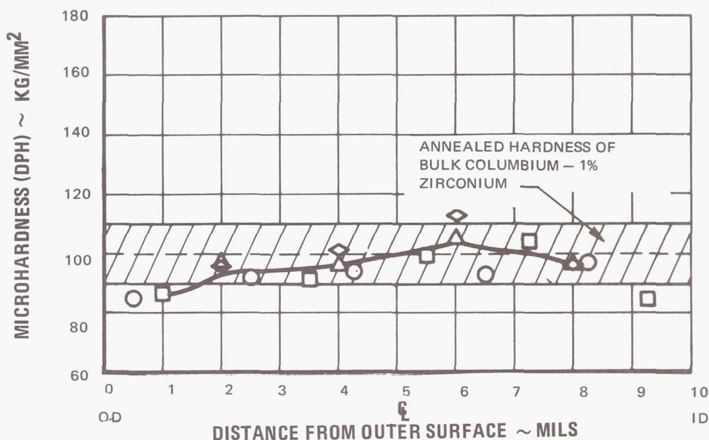
Figure 64 Microhardness Traverse Results for Columbium-1 Percent Zirconium Tube Coated With Aluminum Oxide Aluminum Titanate and Endurance Tested for 10,000 Hours at 1700°F
