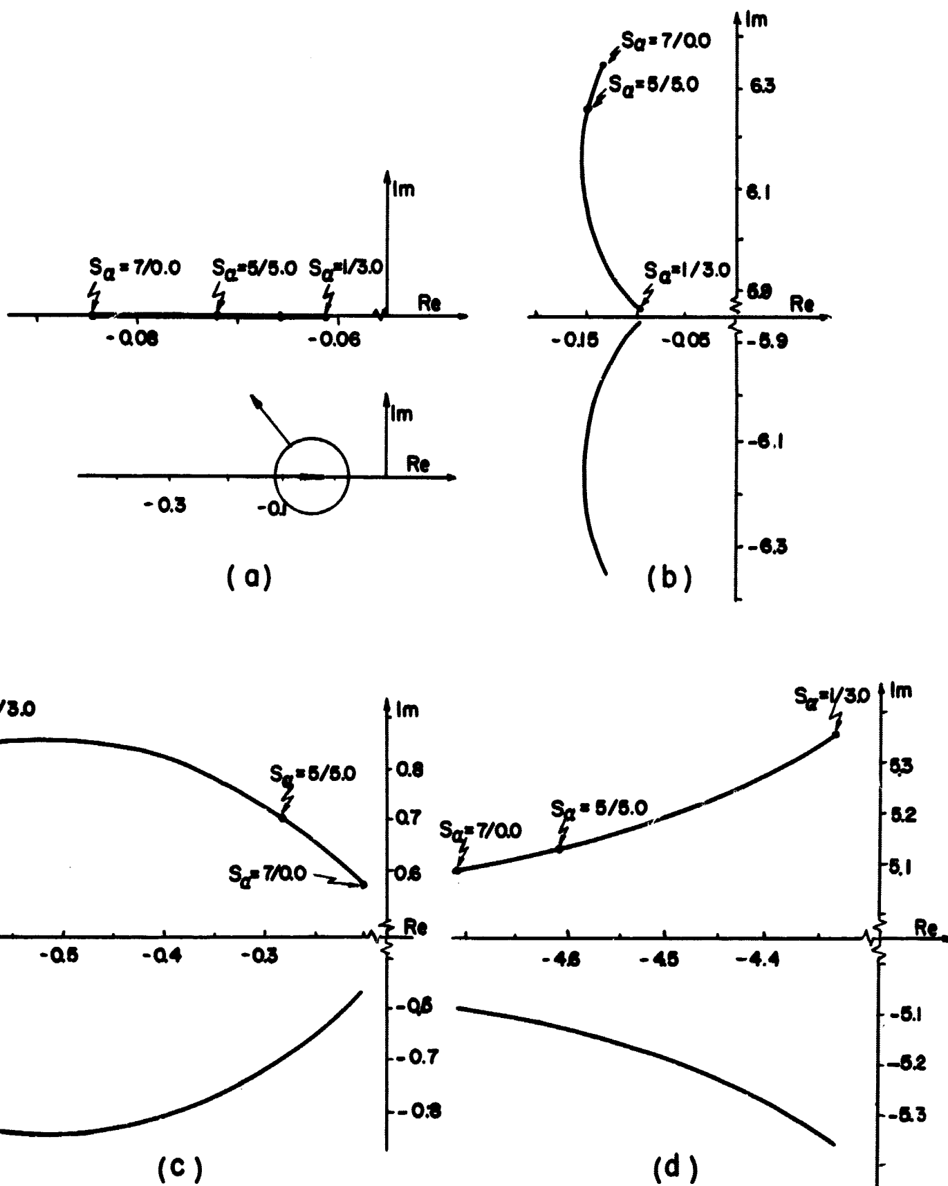
FIGURE 7.17 S_d ROOT LOCUS
