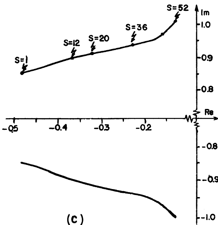
FIGURE 7.18 SENSITIVITY ROOT LOCUS
