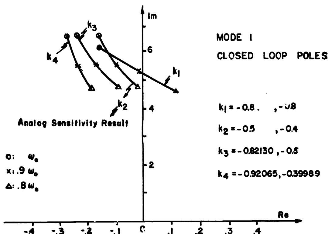
FIGURE 7.21 ROOT LOCUS
