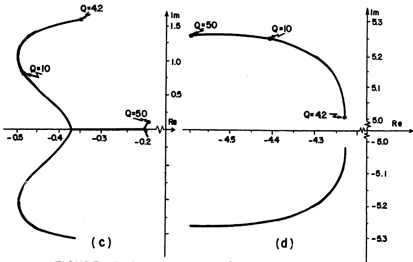
FIGURE 7.10 Q ROOT LOCUS
