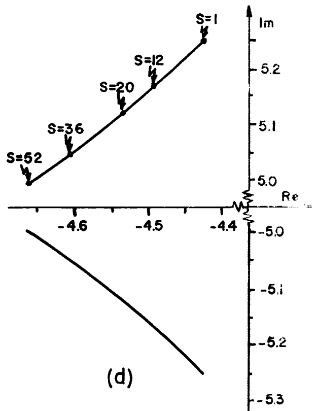
FIGURE 7.18 SENSITIVITY ROOT LOCUS
