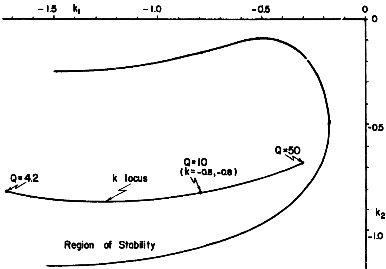
FIGURE 7.8 Q - k LOCUS
