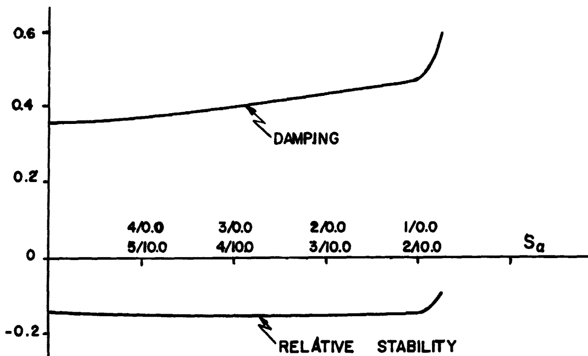
FIGURE 7.12 DAMPING and RELATIVE STABILITY vs. S_a
