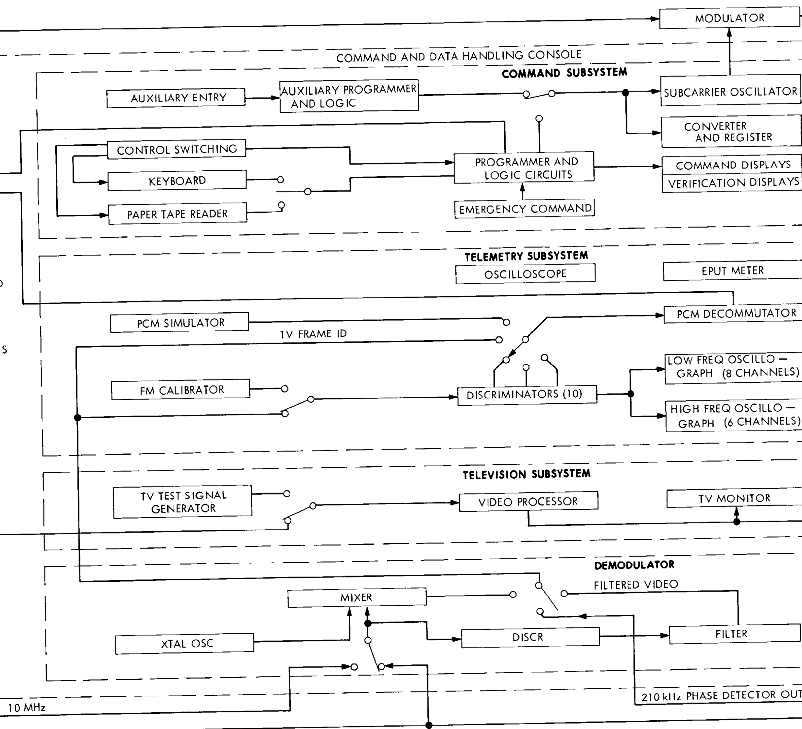
DEEP SPACE INSTRUMENTATION FACILITY, SURVEYOR CONFIGURATION
