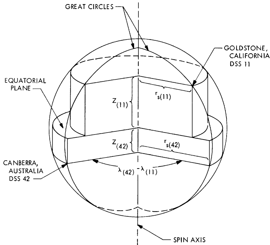
Fig. 16. Station coordinate system
