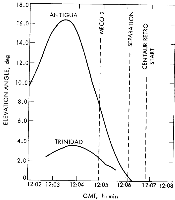
Fig. 36. AFETR tracking coverage for Surveyor IV
