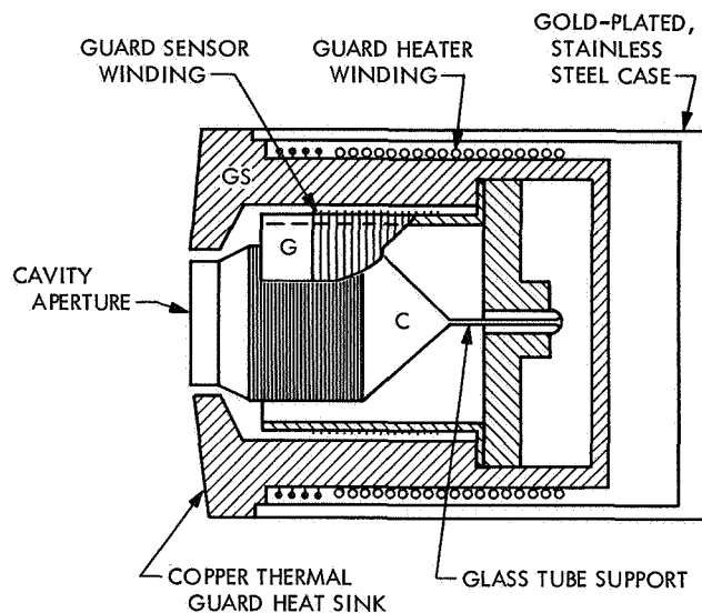
Fig. 1. Active Cavity Radiometer
