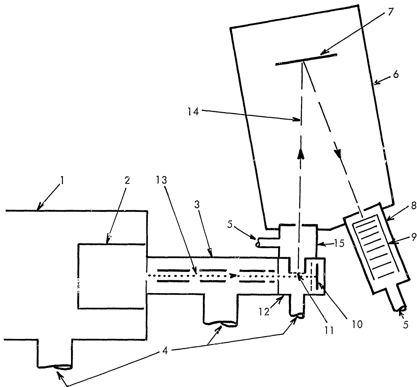
FIG. 3. Experimental apparatus for detection of 584-Å radiation in low-energy \text{He}^+ -He collisions.
